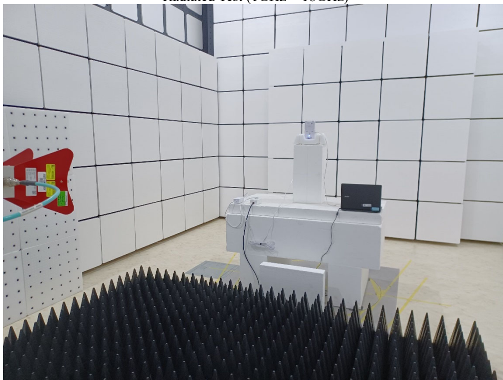
Radiated Test (1GHz ~ 18GHz)
