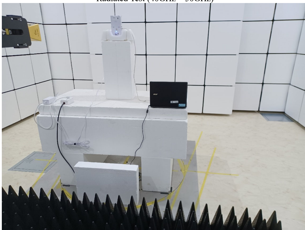
Radiated Test (40GHz ~ 50GHz)
