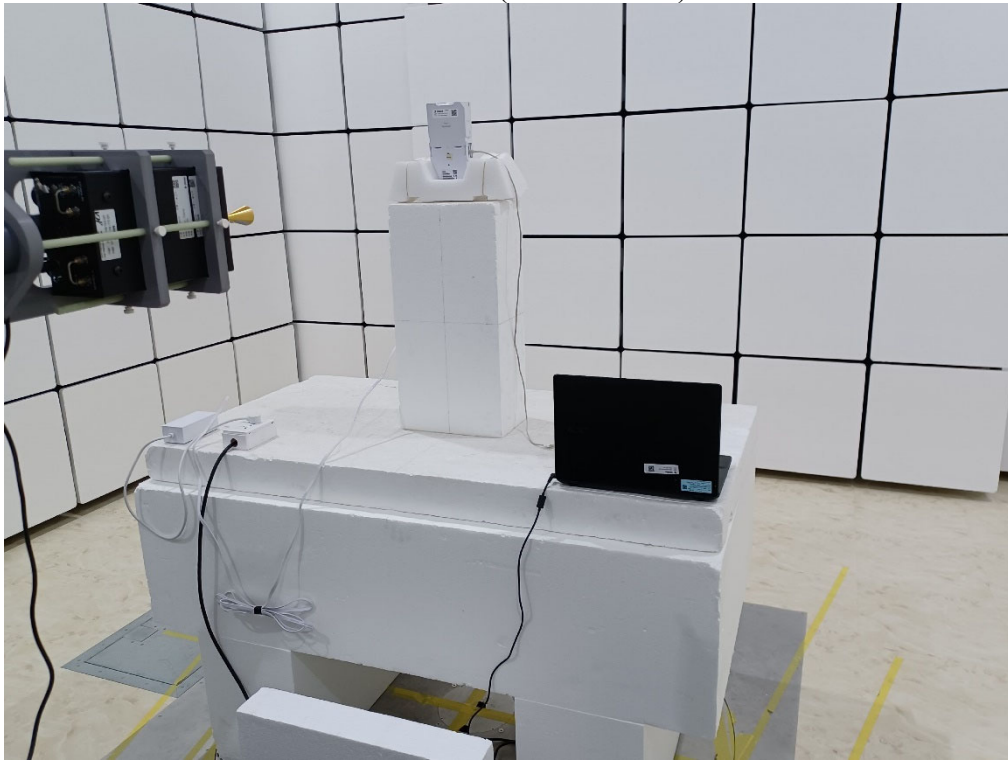
Radiated Test (Above 50GHz)
