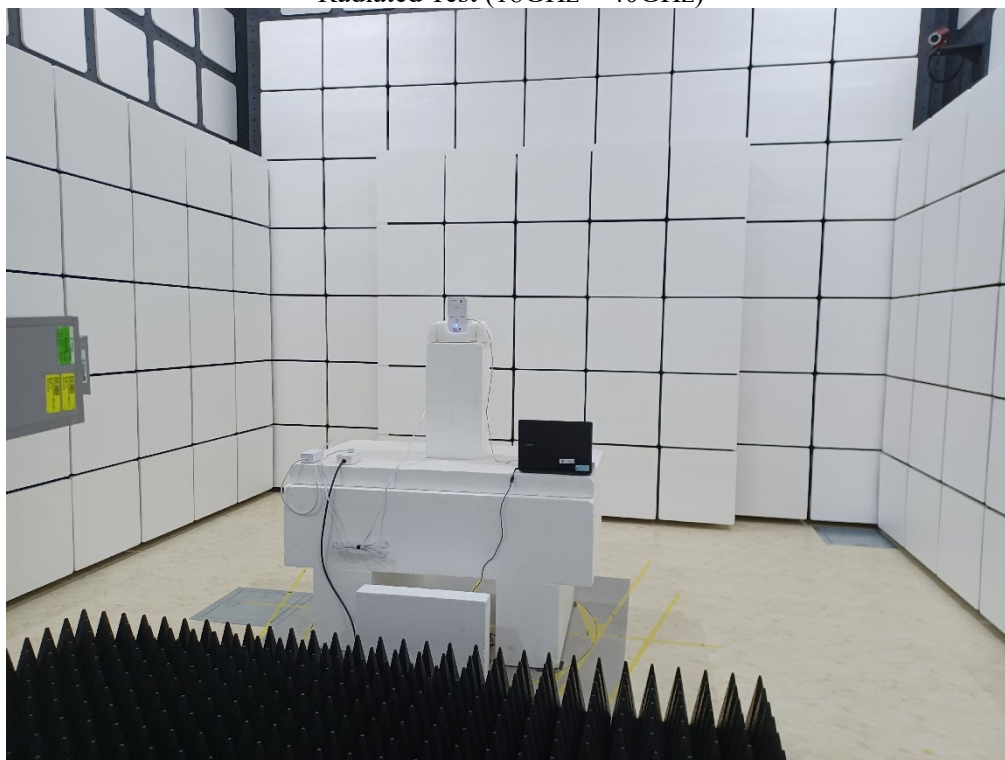
Radiated Test (18GHz ~ 40GHz)
