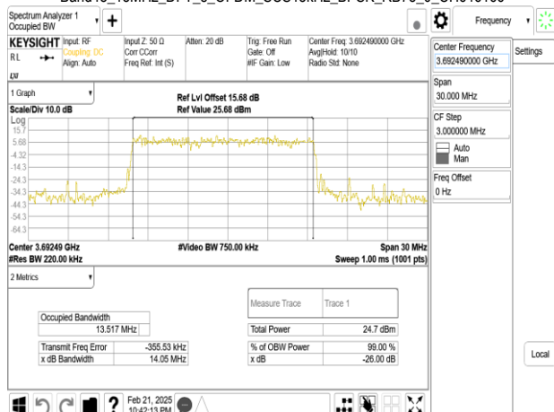
Band48_15MHz_DFT_s_OFDM_SCS15kHz_BPSK_RB75_0_CH646166
