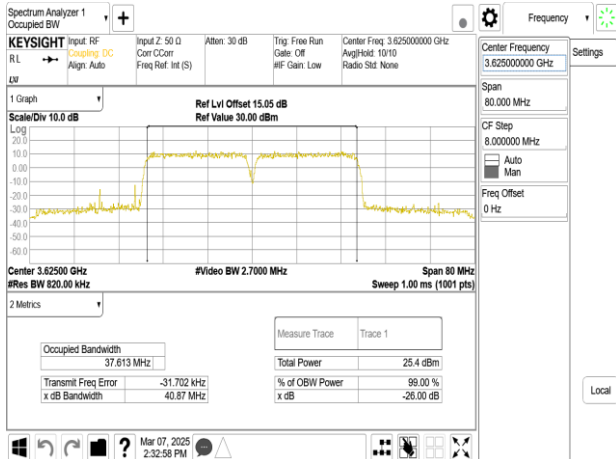
Band48_20MHz+20MHz_64QAM_RB100-0+RB100-0_CH55891+CH56089
