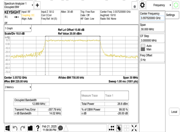
Band48_15MHz_DFT_s_OFDM_SCS30kHz_16QAM_RB36_0_CH641668
