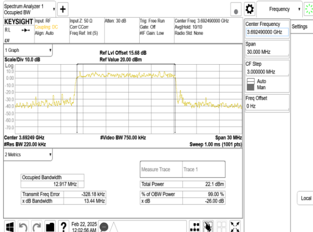
Band48_15MHz_DFT_s_OFDM_SCS30kHz_64QAM_RB36_0_CH646166
