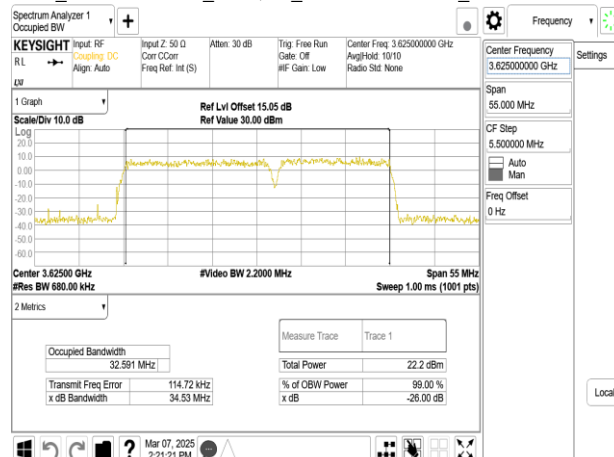
Band48_20MHz+15MHz_256QAM_RB100-0+RB75-0_CH55916+CH56087
