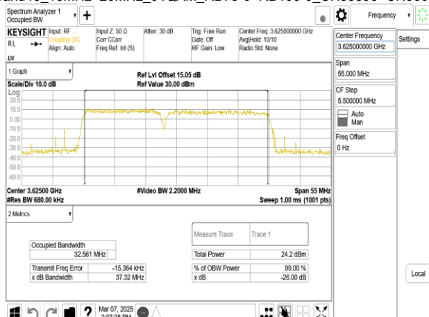
Band48_15MHz+20MHz_256QAM_RB75-0+RB100-0_CH55893+CH56064
