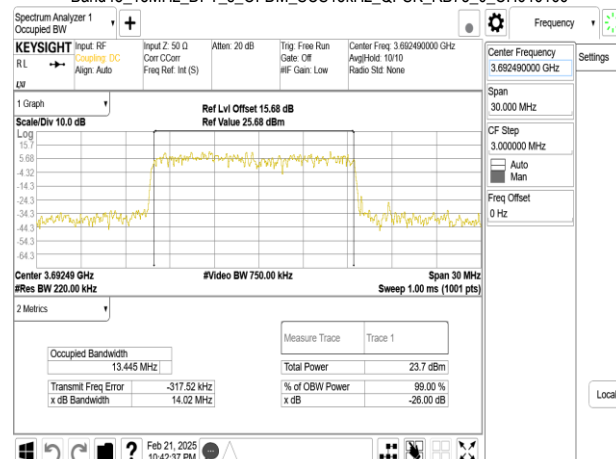
Band48_15MHz_DFT_s_OFDM_SCS15kHz_QPSK_RB75_0_CH646166
