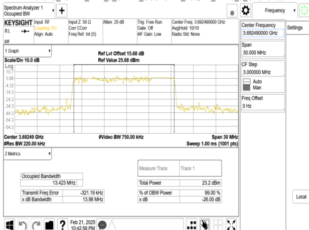
Band48_15MHz_DFT_s_OFDM_SCS15kHz_16QAM_RB75_0_CH646166
