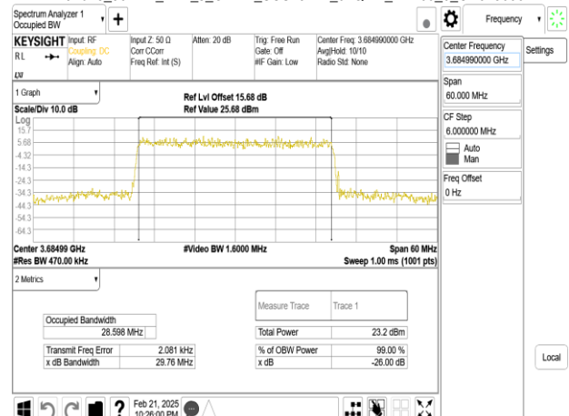
Band48_30MHz_DFT_s_OFDM_SCS15kHz_64QAM_RB160_0_CH645666
