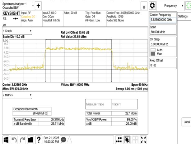
Band48_30MHz_DFT_s_OFDM_SCS15kHz_256QAM_RB160_0_CH645666
