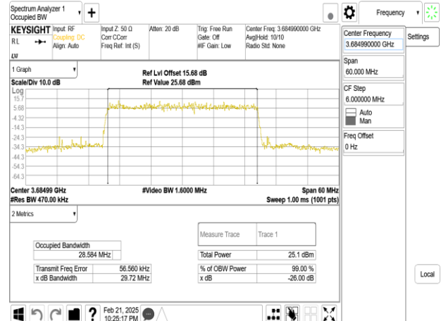
Band48_30MHz_DFT_s_OFDM_SCS15kHz_QPSK_RB160_0_CH645666
