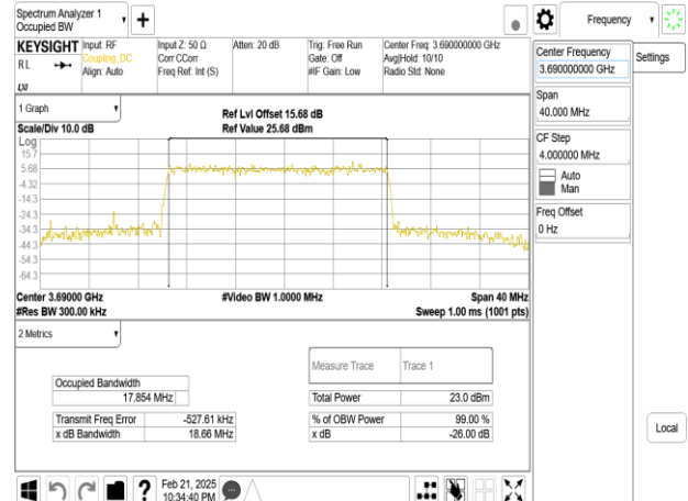
Band48_20MHz_DFT_s_OFDM_SCS15kHz_64QAM_RB100_0_CH646000
