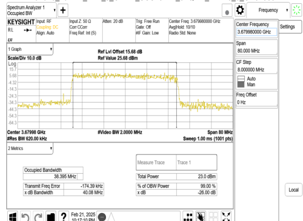
Band48_40MHz_DFT_s_OFDM_SCS15kHz_64QAM_RB216_0_CH645332
