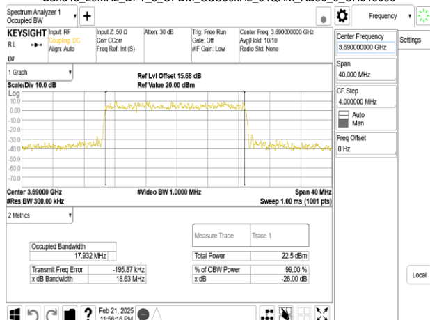
Band48_20MHz_DFT_s_OFDM_SCS30kHz_64QAM_RB50_0_CH646000
