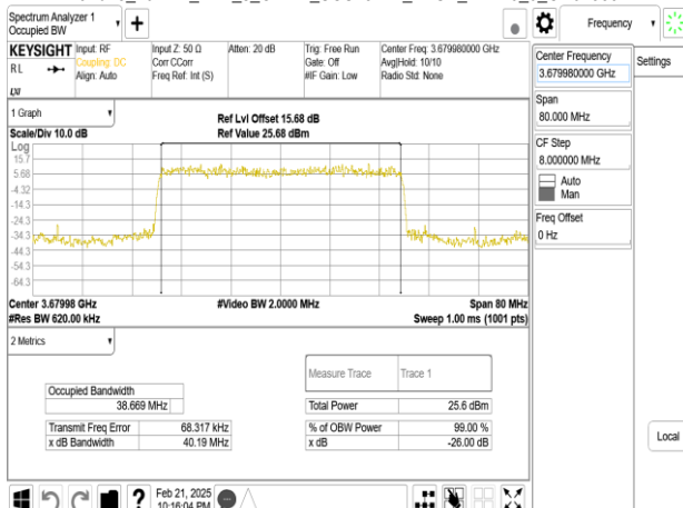
Band48_40MHz_DFT_s_OFDM_SCS15kHz_BPSK_RB216_0_CH645332
