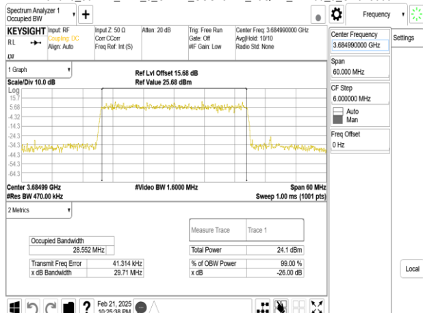
Band48_30MHz_DFT_s_OFDM_SCS15kHz_16QAM_RB160_0_CH645666
