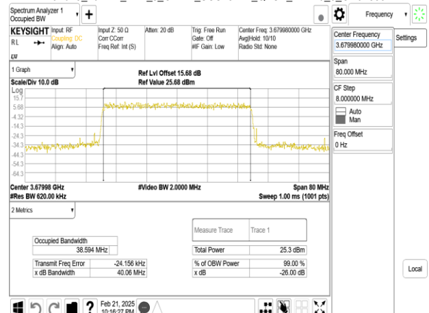
Band48_40MHz_DFT_s_OFDM_SCS15kHz_QPSK_RB216_0_CH645332
