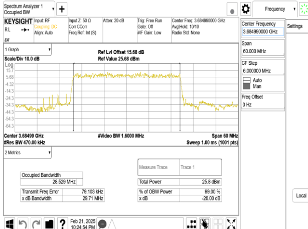
Band48_30MHz_DFT_s_OFDM_SCS15kHz_BPSK_RB160_0_CH645666
