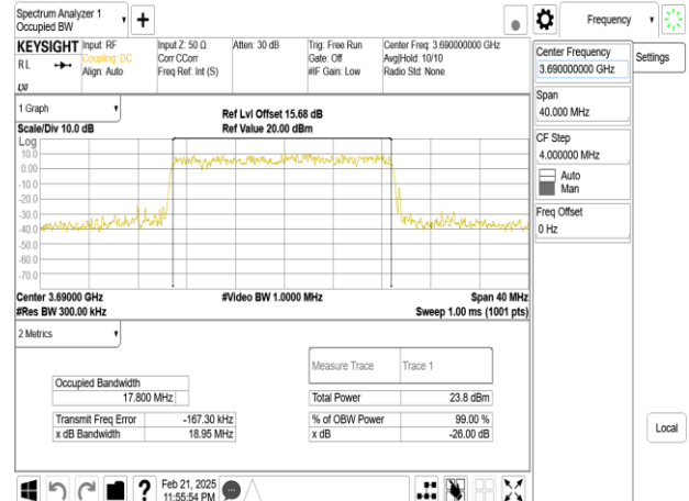
Band48_20MHz_DFT_s_OFDM_SCS30kHz_16QAM_RB50_0_CH646000
