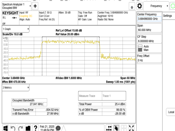
Band48_30MHz_DFT_s_OFDM_SCS30kHz_QPSK_RB75_0_CH645666
