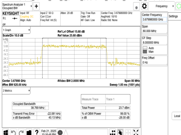
Band48_40MHz_DFT_s_OFDM_SCS15kHz_16QAM_RB216_0_CH645332
