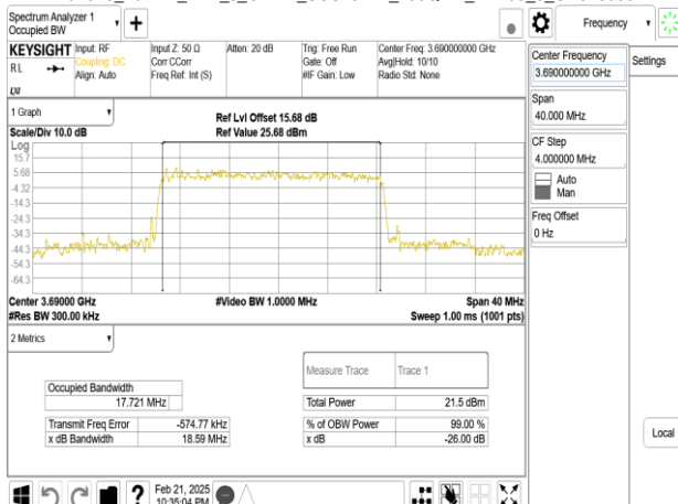
Band48_20MHz_DFT_s_OFDM_SCS15kHz_256QAM_RB100_0_CH646000
