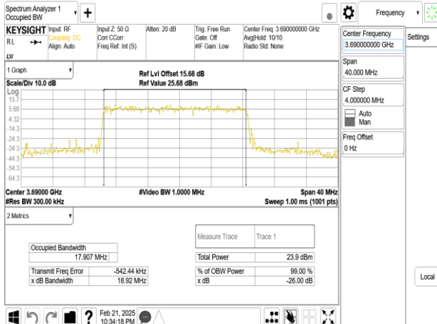
Band48_20MHz_DFT_s_OFDM_SCS15kHz_16QAM_RB100_0_CH646000
