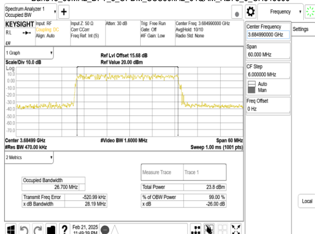
Band48_30MHz_DFT_s_OFDM_SCS30kHz_64QAM_RB75_0_CH645666
