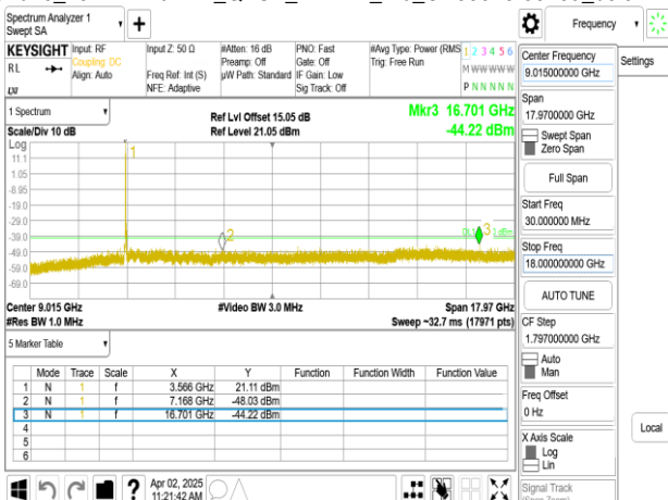
Band48_15MHz+20MHz_QPSK_RB1-74_1-0_CH55318-55489_upper 18G
