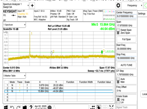
Band48_15MHz+20MHz_QPSK_RB1-74_1-0_CH56469-56640_upper 18G
