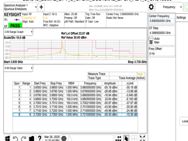
Band48_20MHz_DFT_s_OFDM_SCS15kHz_BPSK_RB1_0_CH646000
