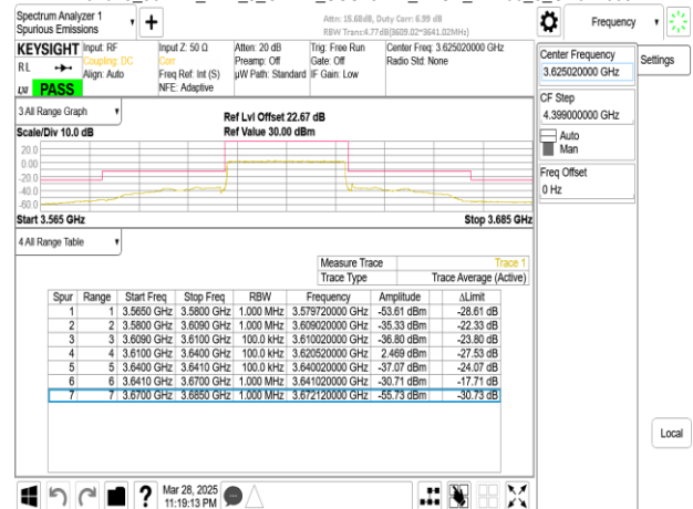
Band48_30MHz_DFT_s_OFDM_SCS15kHz_BPSK_RB1_0_CH641668
