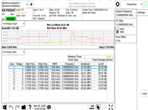
Band48_20MHz_DFT_s_OFDM_SCS30kHz_BPSK_RB50_0_CH646000
