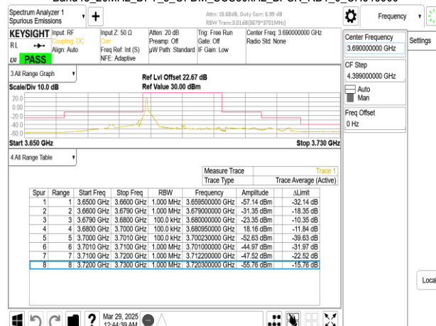
Band48_20MHz_DFT_s_OFDM_SCS30kHz_BPSK_RB1_0_CH646000
