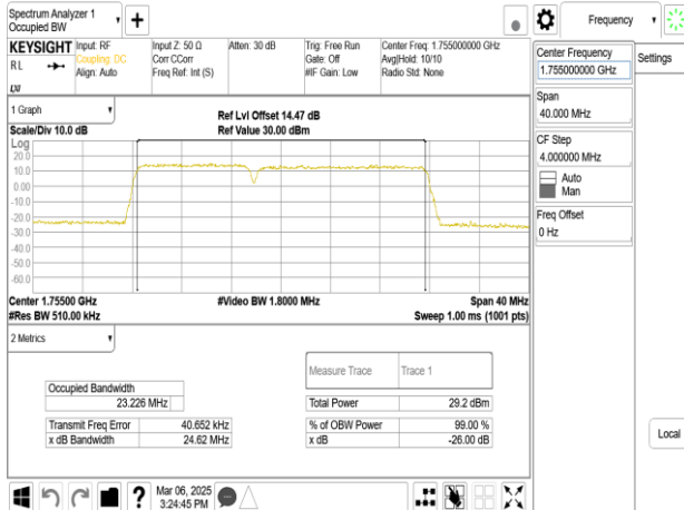
Band66_10MHz+15MHz_16QAM_RB50-0+RB75-0_CH132351+CH132471
