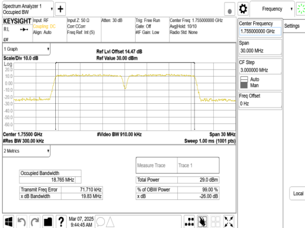
Band66B_10MHz+10MHz_64QAM_RB50-0+RB50-0_CH132373+CH132472
