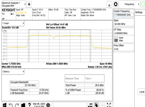
Band66_10MHz+15MHz_64QAM_RB50-0+RB75-0_CH132351+CH132471
