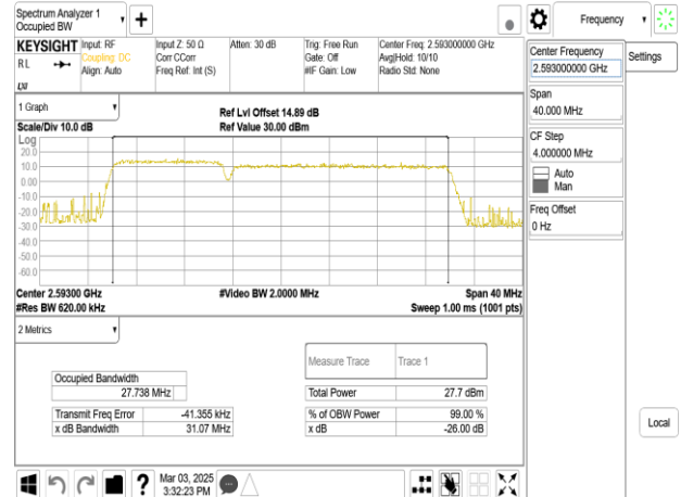
Band41_10MHz+20MHz_64QAM_RB50-0+RB100-0_CH40526+CH40670
