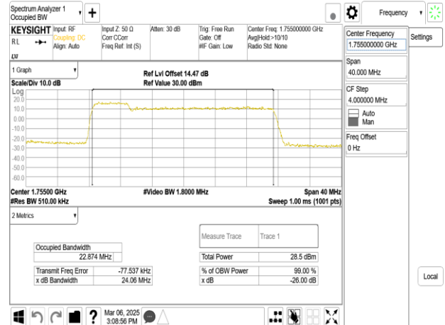
Band66_5MHz+20MHz_64QAM_RB25-0+RB100-0_CH132330+CH132447
