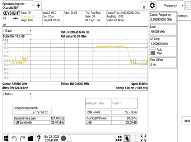
Band41_20MHz+10MHz_256QAM_RB100-0+RB50-0_CH40571+CH40715
