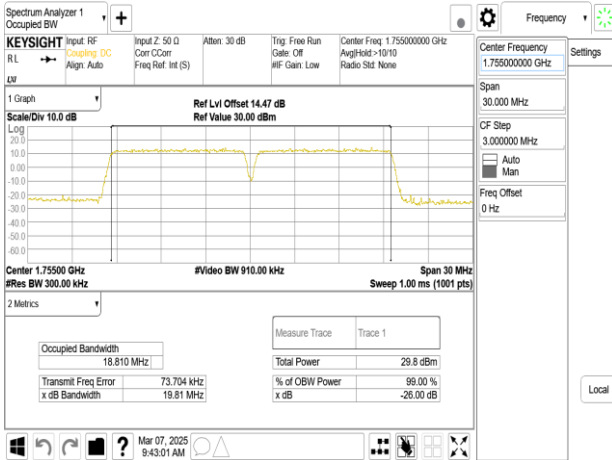
Band66B_10MHz+10MHz_16QAM_RB50-0+RB50-0_CH132373+CH132472
