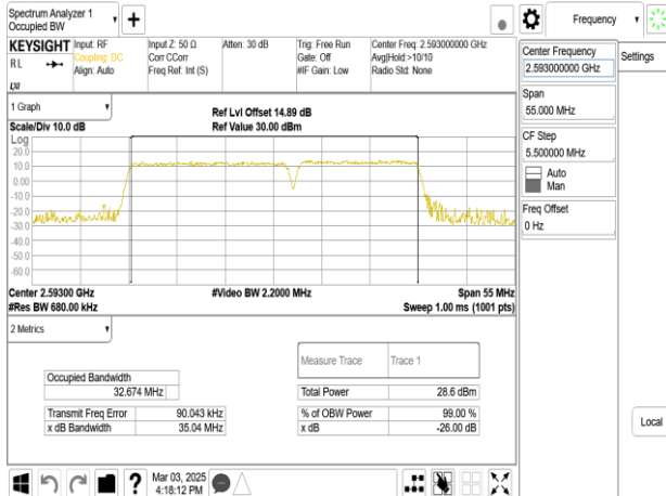
Band41_20MHz+15MHz_16QAM_RB100-0+RB75-0_CH40546+CH40717
