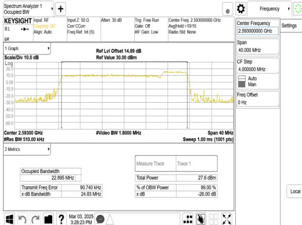
Band41_20MHz+5MHz_256QAM_RB100-0+RB25-0_CH40595+CH40712
