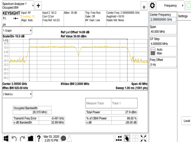
Band38_15MHz+15MHz_256QAM_RB75-0+RB75-0_CH37925+CH38075
