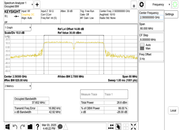
Band41_20MHz+20MHz_16QAM_RB100-0+RB100-0_CH40521+CH40719
