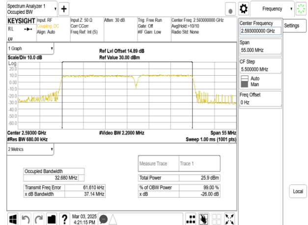
Band41_20MHz+20MHz_QPSK_RB100-0+RB100-0_CH40521+CH40719
