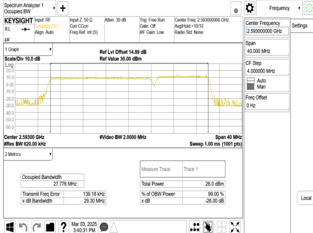
Band41_15MHz+20MHz_QPSK_RB75-0+RB100-0_CH40523+CH40694
