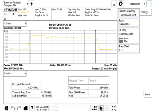
Band66B_5MHz+15MHz_256QAM_RB25-0+RB75-0_CH132353+CH132446
