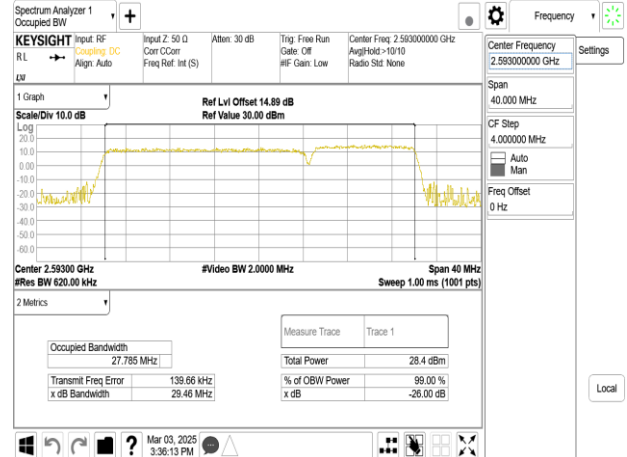
Band41_20MHz+10MHz_16QAM_RB100-0+RB50-0_CH40571+CH40715
