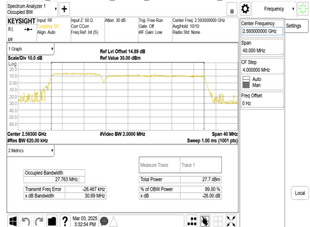
Band41_10MHz+20MHz_256QAM_RB50-0+RB100-0_CH40526+CH40670
