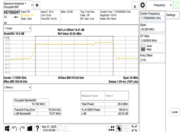
Band66B_15MHz+5MHz_16QAM_RB75-0+RB25-0_CH132398+CH132491
