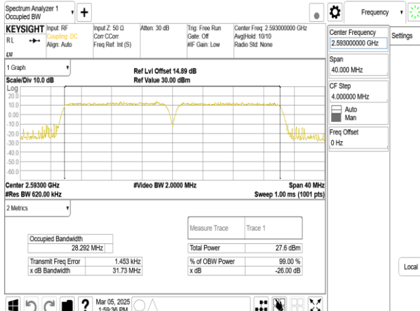
Band41_15MHz+15MHz_64QAM_RB75-0+RB75-0_CH40545+CH40695
