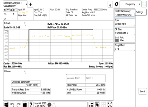
Band66B_10MHz+5MHz_16QAM_RB50-0+RB25-0_CH132397+CH132469
