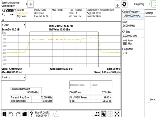
Band66_5MHz+20MHz_QPSK_RB25-0+RB100-0_CH132330+CH132447
