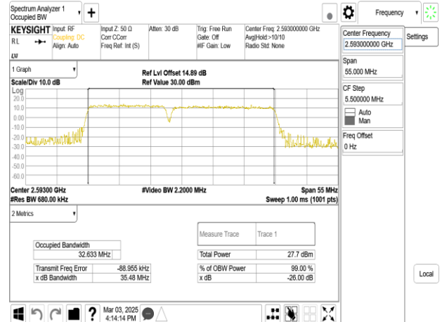
Band41_15MHz+20MHz_64QAM_RB75-0+RB100-0_CH40523+CH40694
