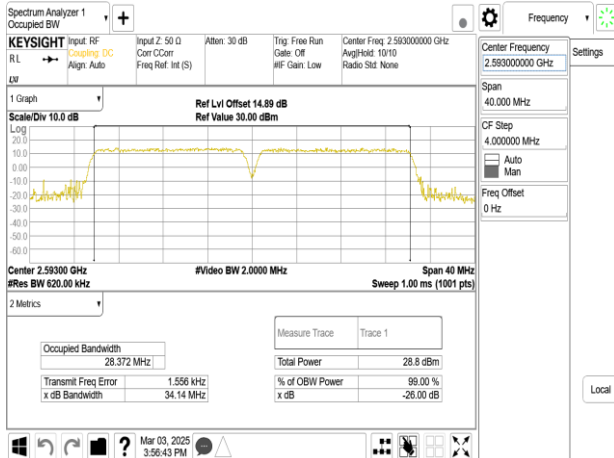
Band41_15MHz+15MHz_16QAM_RB75-0+RB75-0_CH40545+CH40695
