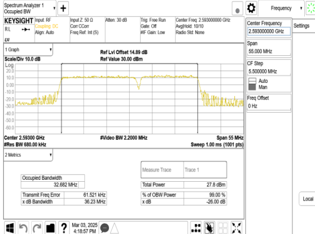
Band41_20MHz+15MHz_64QAM_RB100-0+RB75-0_CH40546+CH40717
