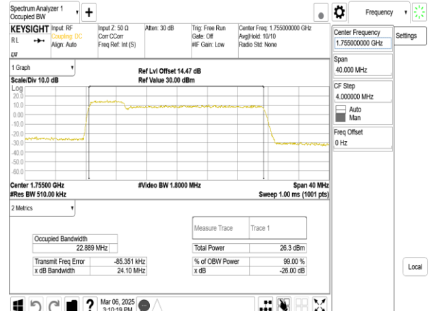
Band66_5MHz+20MHz_256QAM_RB25-0+RB100-0_CH132330+CH132447
