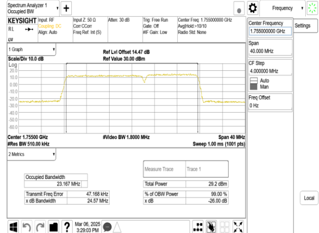
Band66_15MHz+10MHz_16QAM_RB75-0+RB50-0_CH132373+CH132493
