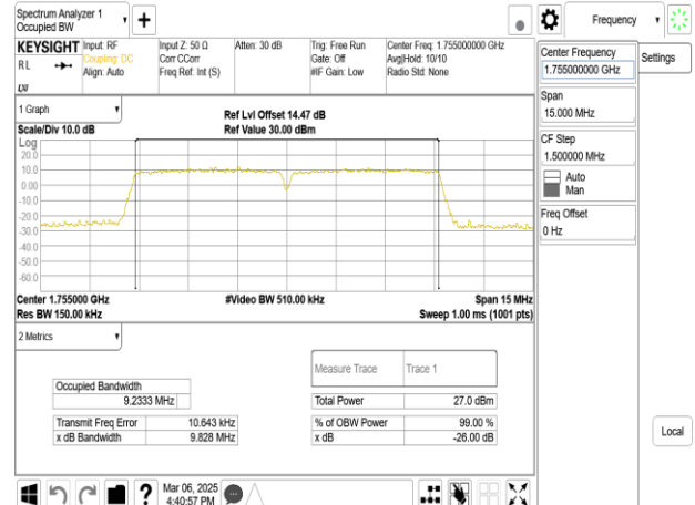
Band66B_5MHz+5MHz_256QAM_RB25-0+RB25-0_CH132398+CH132446
