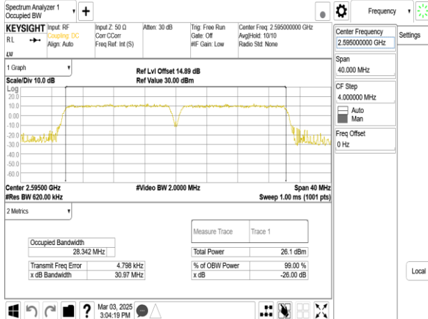
Band38_20MHz+20MHz_QPSK_RB100-0+RB100-0_CH37901+CH38099
