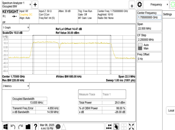
Band66B_5MHz+10MHz_64QAM_RB25-0+RB50-0_CH132375+CH132447
