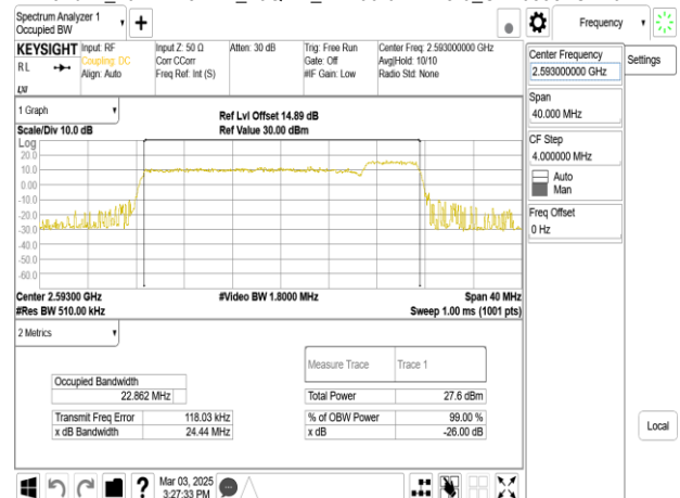
Band41_20MHz+5MHz_16QAM_RB100-0+RB25-0_CH40595+CH40712
