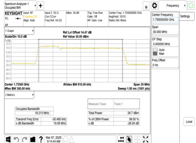
Band66B_5MHz+15MHz_64QAM_RB25-0+RB75-0_CH132353+CH132446
