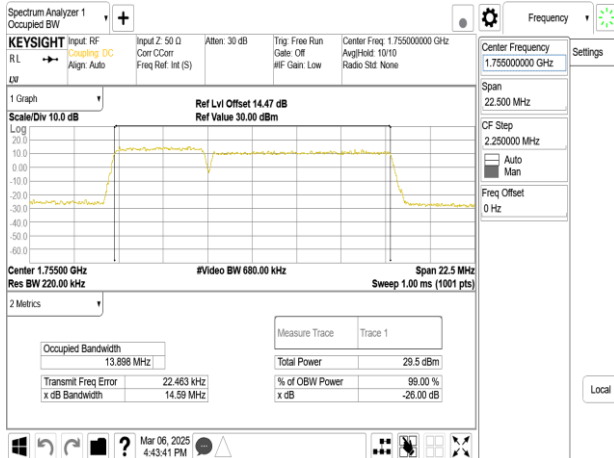
Band66B_5MHz+10MHz_16QAM_RB25-0+RB50-0_CH132375+CH132447
