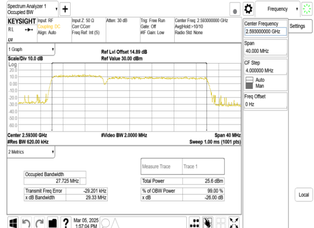
Band41_10MHz+20MHz_256QAM_RB50-0+RB100-0_CH40526+CH40670
