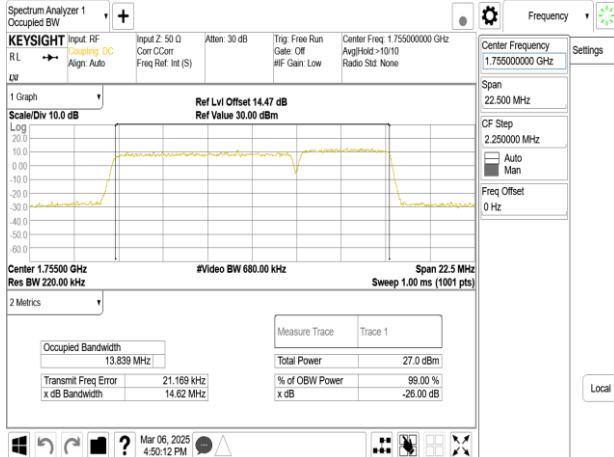
Band66B_5MHz+15MHz_QPSK_RB25-0+RB75-0_CH132353+CH132446
