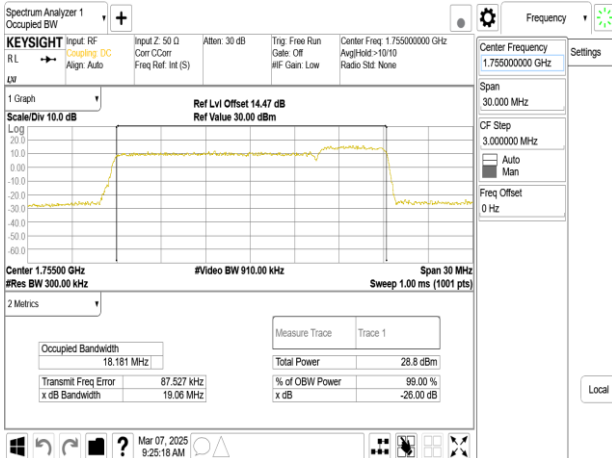
Band66B_15MHz+5MHz_256QAM_RB75-0+RB25-0_CH132398+CH132491
