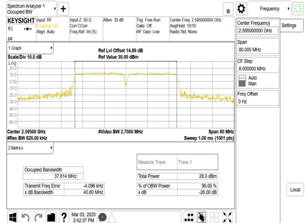
Band38_20MHz+20MHz_64QAM_RB100-0+RB100-0_CH37901+CH38099
