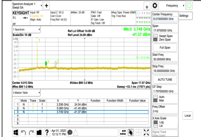
Band7_15MHz+15MHz_QPSK_RB1-74_1-0_CH21025-21175_low 18G
