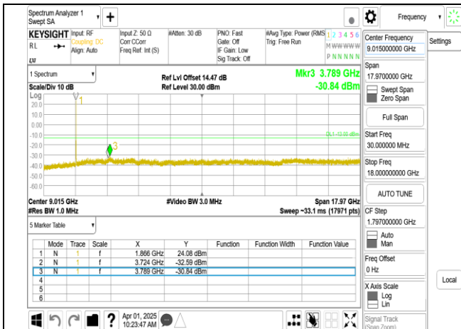
Band2_15MHz+15MHz_QPSK_RB1-74_1-0_CH18675-18825_low 18G
