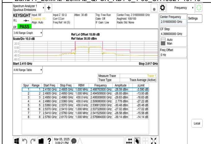
Band41 20MHz+20MHz QPSK RB100-0 100-0 CH39750-39948
