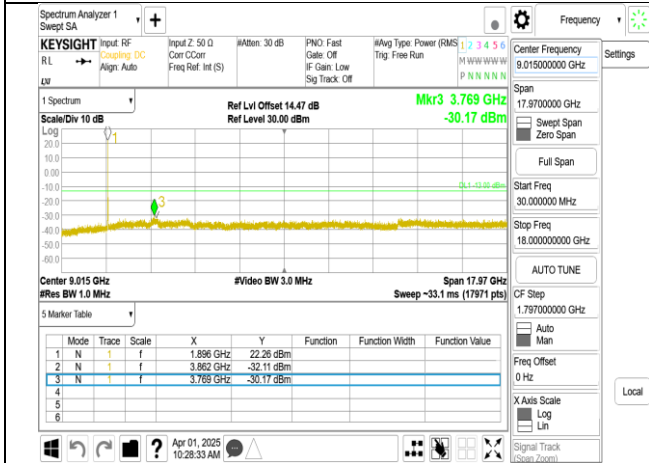
Band2_15MHz+15MHz_QPSK_RB1-74_1-0_CH18975-19125_low 18G
