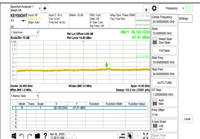
Band38_15MHz+15MHz_QPSK_RB1-74_1-0_CH37825-37975_up-per 18G
