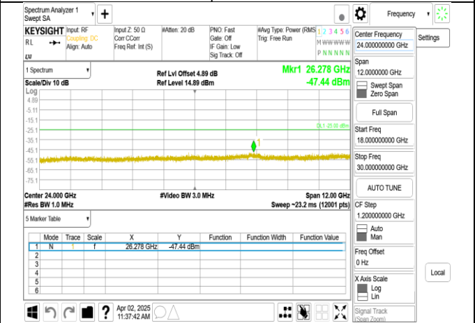
Band7_15MHz+15MHz_QPSK_RB1-74_1-0_CH21225-21375_up per 18G
