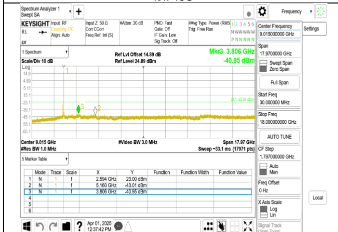
Band38_15MHz+15MHz_QPSK_RB1-74_1-0_CH37925-38075_be-low 18G
