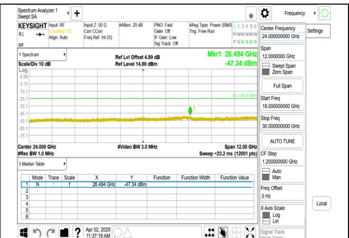
Band7_15MHz+15MHz_QPSK_RB1-74_1-0_CH20825-20975_up per 18G
