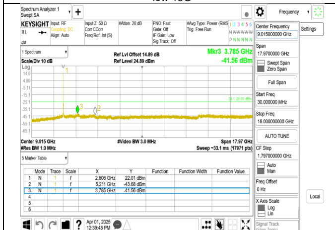
Band38_15MHz+15MHz_QPSK_RB1-74_1-0_CH38025-38175_be-low 18G
