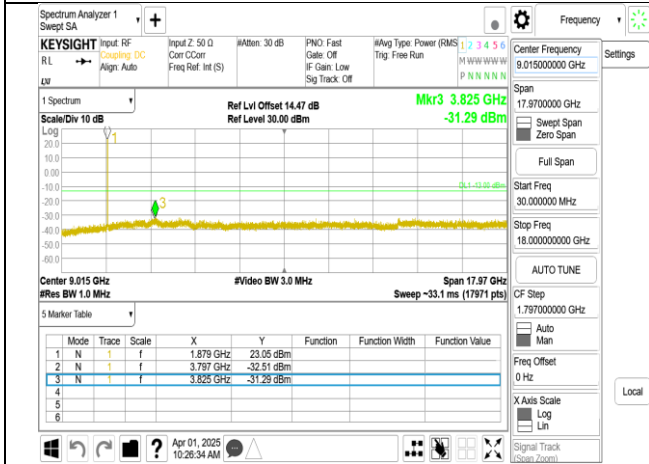
Band2_15MHz+15MHz_QPSK_RB1-74_1-0_CH18825-18975_low 18G
