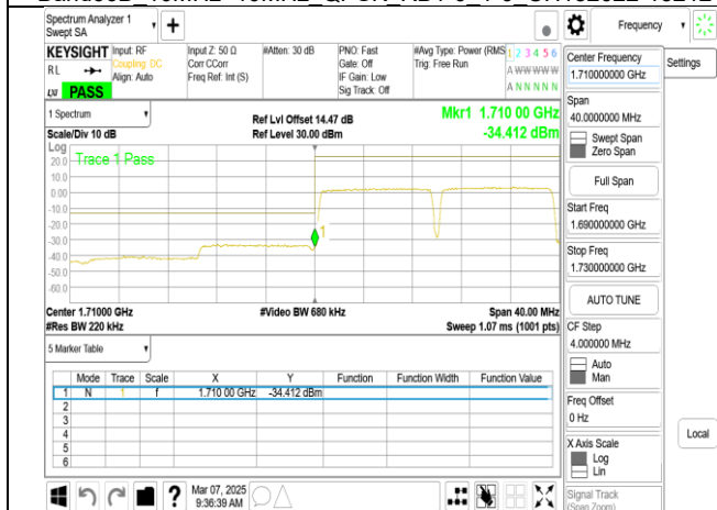
Band66B 10MHz+10MHz QPSK RB50-0 50-0 CH132022-132121
