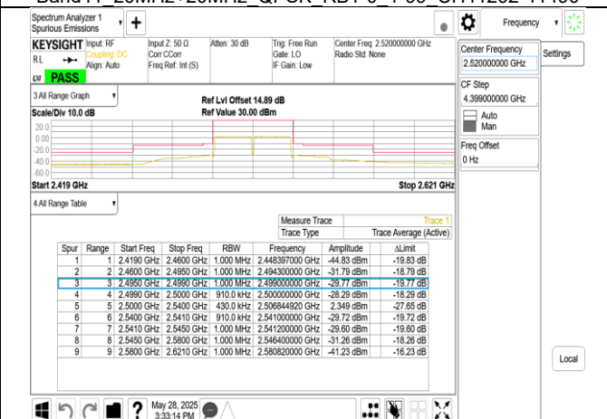
Band41 20MHz+20MHz QPSK RB100-0 100-0 CH39790-39988
