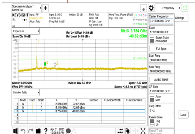
Band38_15MHz+15MHz_QPSK_RB1-74_1-0_CH37825-37975_be-low 18G
