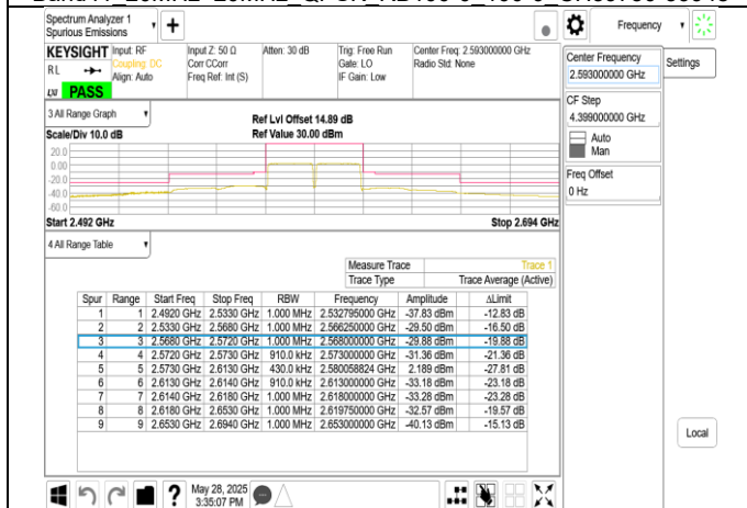
Band41 20MHz+20MHz QPSK RB100-0 100-0 CH40521-40719
