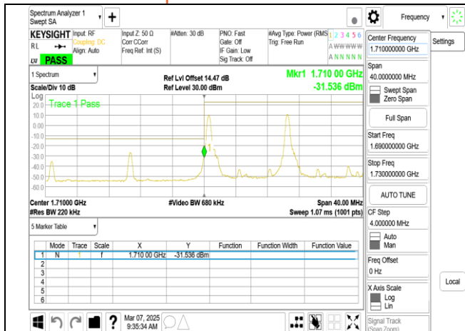
Band66B 10MHz+10MHz QPSK RB1-0 1-0 CH132022-132121
