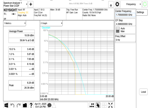
Band66_20MHz+5MHz_256QAM_RB100-0+RB25-0_CH132397+CH132514
