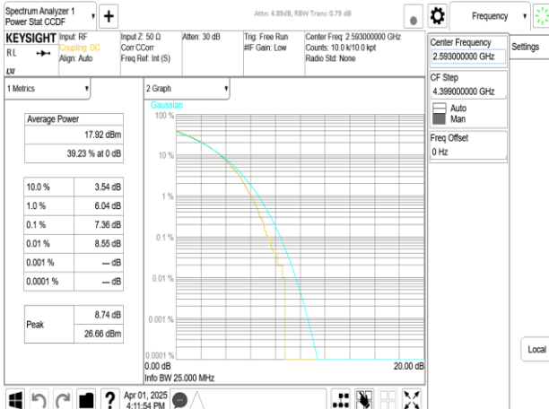
Band41_10MHz+20MHz_256QAM_RB50-0+RB100-0_CH40526+CH40670
