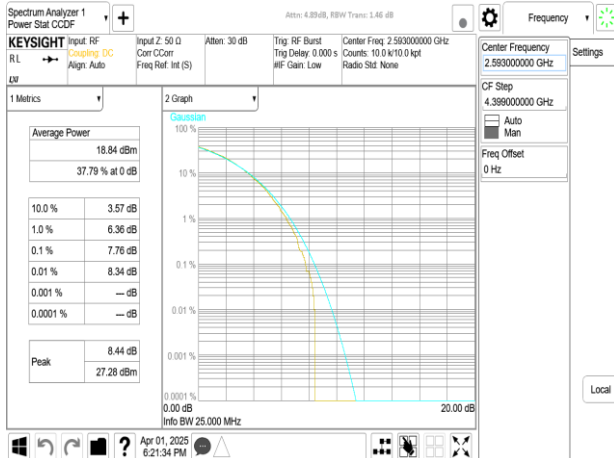
Band41_20MHz+20MHz_256QAM_RB100-0+RB100-0_CH40521+CH40719
