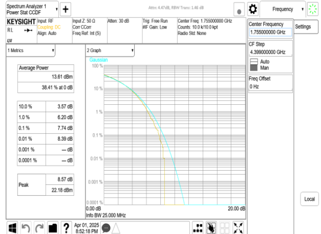
Band66_20MHz+15MHz_256QAM_RB100-0+RB75-0_CH132348+CH132519
