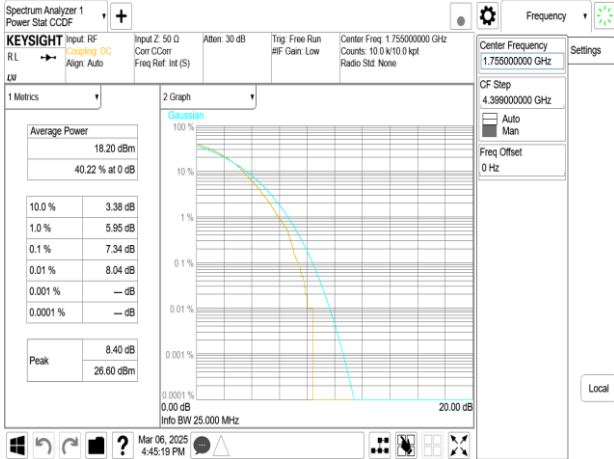
Band66B_10MHz+5MHz_256QAM_RB50-0+RB25-0_CH132397+CH132469
