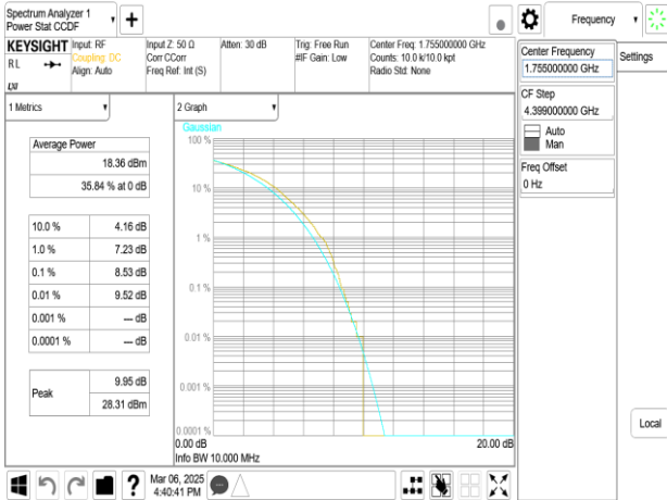
Band66B_5MHz+10MHz_256QAM_RB25-0+RB50-0_CH132375+CH132447
