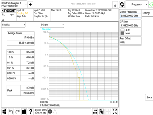
Band41_20MHz+5MHz_256QAM_RB100-0+RB25-0_CH40595+CH40712
