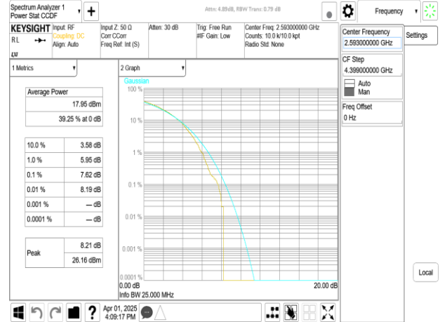
Band41_15MHz+20MHz_256QAM_RB75-0+RB100-0_CH40523+CH40694
