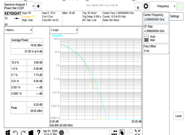
Band38_20MHz+20MHz_256QAM_RB100-0+RB100-0_CH37901+CH38099
