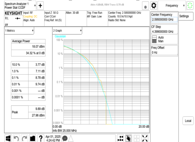
Band38_20MHz+20MHz_256QAM_RB100-0+RB100-0_CH37901+CH38099
