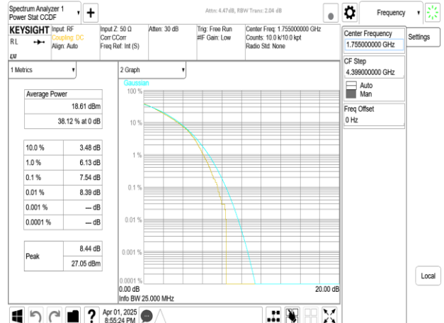
Band66_20MHz+20MHz_256QAM_RB100-0+RB100-0_CH132323+CH132521
