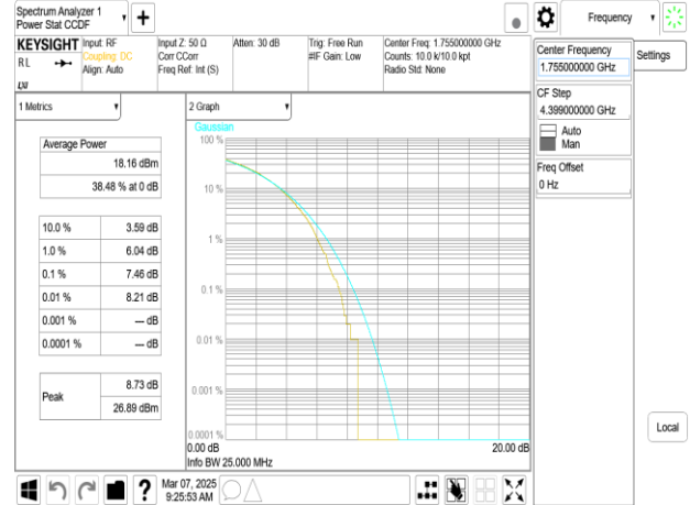
Band66B_10MHz+10MHz_256QAM_RB50-0+RB50-0_CH132373+CH132472
