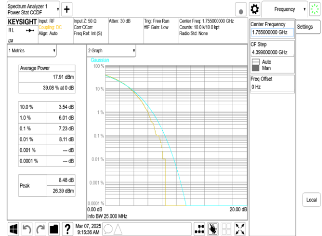
Band66B_15MHz+5MHz_256QAM_RB75-0+RB25-0_CH132398+CH132491
