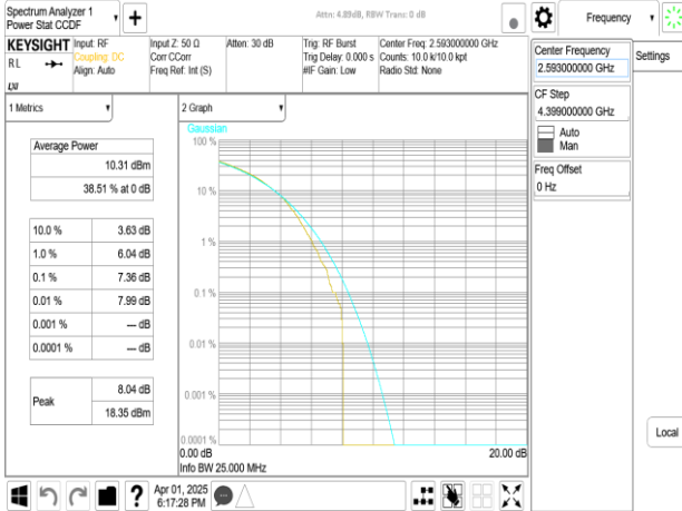
Band41_10MHz+20MHz_256QAM_RB50-0+RB100-0_CH40526+CH40670
