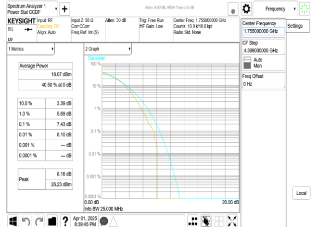
Band66_15MHz+10MHz_256QAM_RB75-0+RB50-0_CH132373+CH132493
