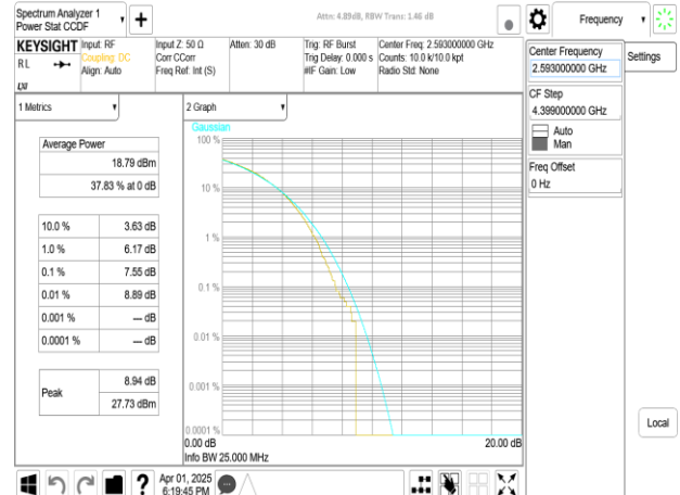
Band41_15MHz+20MHz_256QAM_RB75-0+RB100-0_CH40523+CH40694
