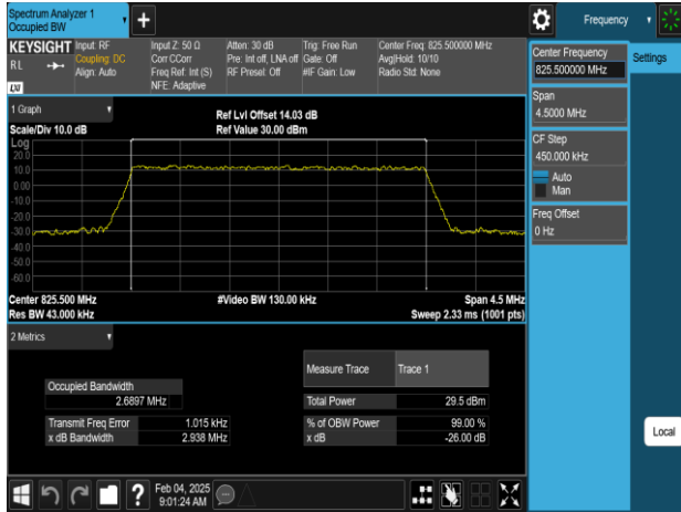
Band5_3MHz_64QAM_RB15_0_CH20415
