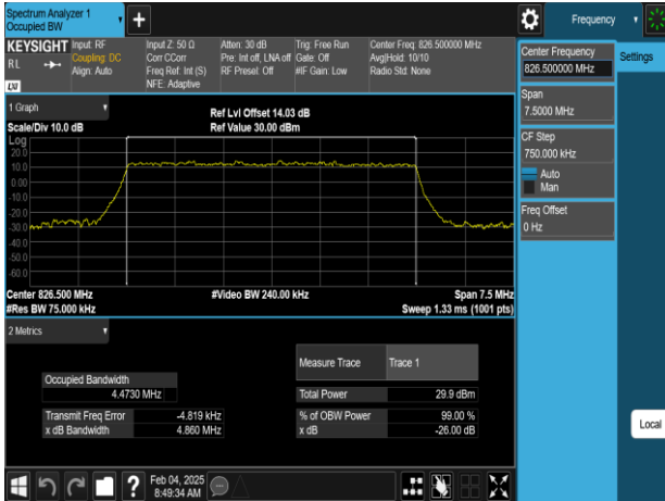
Band5_5MHz_64QAM_RB25_0_CH20425
