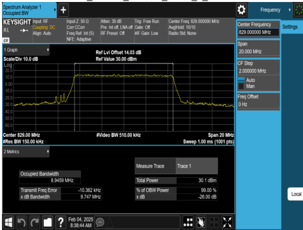
Band5_10MHz_64QAM_RB50_0_CH20450
