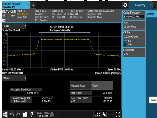
Band5_10MHz_256QAM_RB50_0_CH20525
