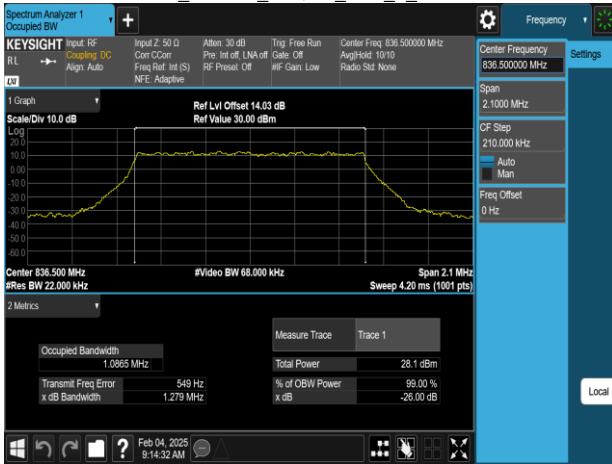
Band5_1.4MHz_256QAM_RB6_0_CH20525
