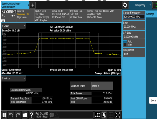
Band5_10MHz_16QAM_RB50_0_CH20450
