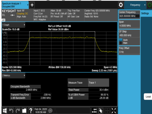
Band5_3MHz_16QAM_RB15_0_CH20415
