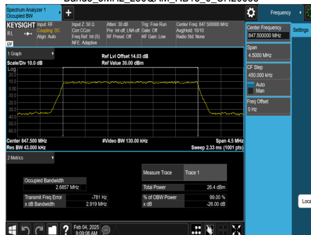
Band5_3MHz_256QAM_RB15_0_CH20635
