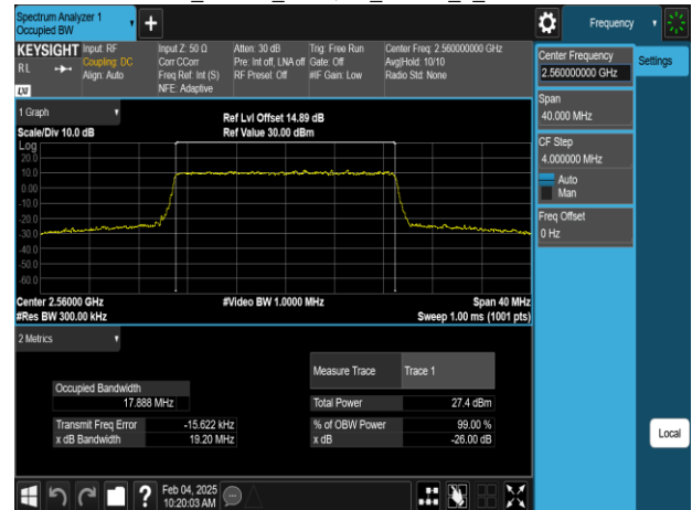
Band7_20MHz_256QAM_RB100_0_CH21350
