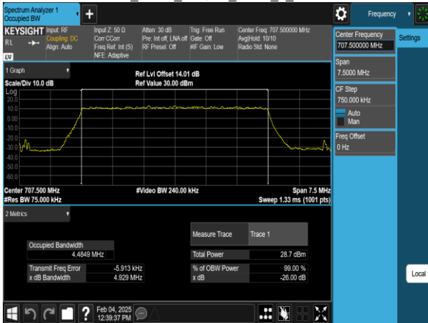
Band12_5MHz_256QAM_RB25_0_CH23095
