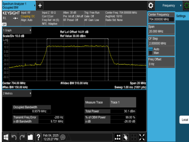
Band12_10MHz_64QAM_RB50_0_CH23060
