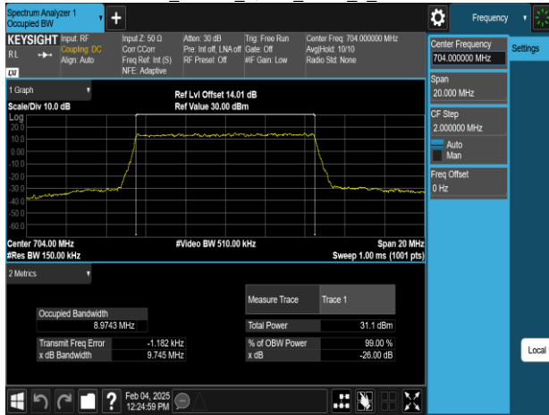
Band12_10MHz_16QAM_RB50_0_CH23060
