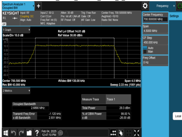
Band12_3MHz_64QAM_RB15_0_CH23025
