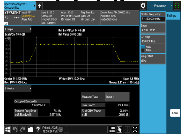
Band12_3MHz_64QAM_RB15_0_CH23165
