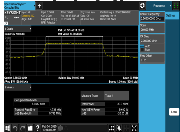
Band7_10MHz_64QAM_RB50_0_CH21400
