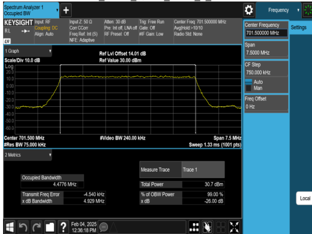
Band12_5MHz_16QAM_RB25_0_CH23035
