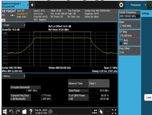
Band12_1.4MHz_16QAM_RB6_0_CH23017
