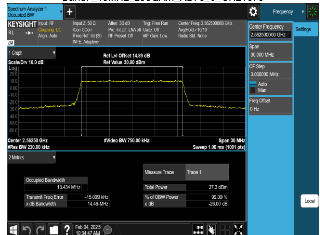
Band7 15MHz 256QAM_RB75_0_CH21375
