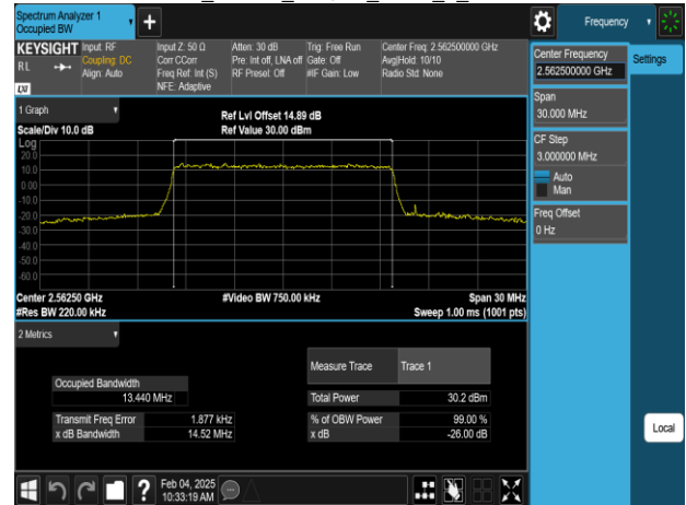
Band7 15MHz 64QAM_RB75_0_CH21375
