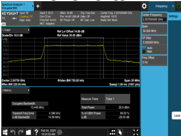
Band7_15MHz_64QAM_RB75_0_CH20825
