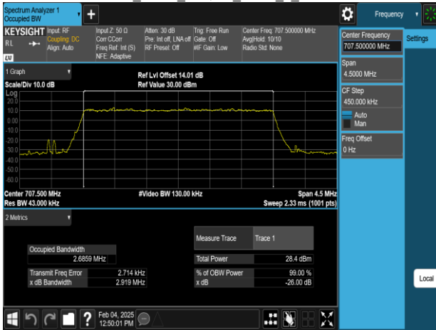
Band12_3MHz_256QAM_RB15_0_CH23095
