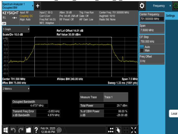
Band12_5MHz_64QAM_RB25_0_CH23035
