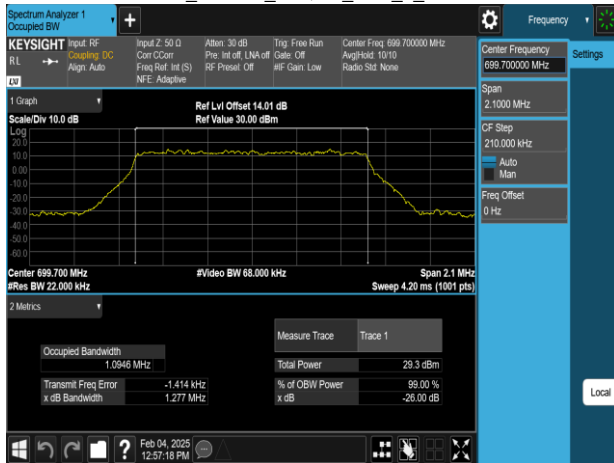
Band12_1.4MHz_64QAM_RB6_0_CH23017
