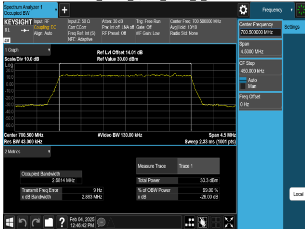
Band12_3MHz_16QAM_RB15_0_CH23025
