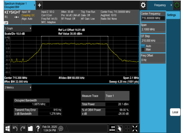
Band12 1.4MHz 256QAM_RB6_0_CH23173
