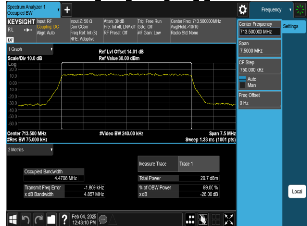
Band12_5MHz_64QAM_RB25_0_CH23155
