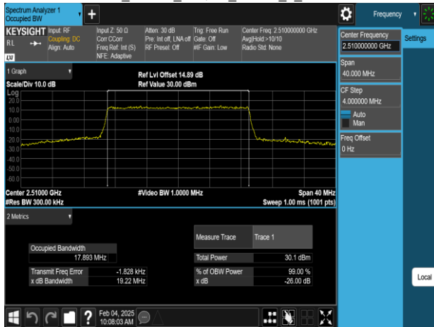
Band7_20MHz_64QAM_RB100_0_CH20850
