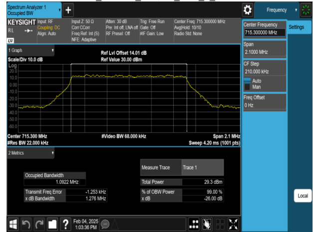
Band12 1.4MHz 64QAM_RB6_0_CH23173
