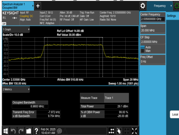
Band7_10MHz_256QAM_RB50_0_CH21100
