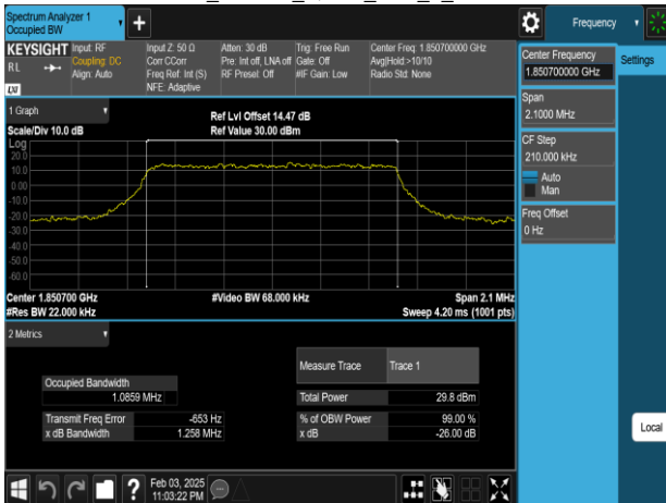
Band25 1.4MHz_QPSK_RB6_0_CH26047
