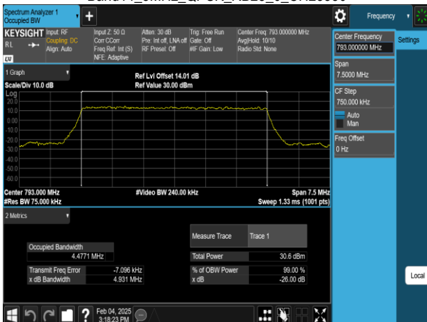
Band14_5MHz_QPSK_RB25_0_CH23330
