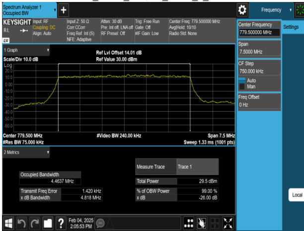
Band13_5MHz_64QAM_RB25_0_CH23205
