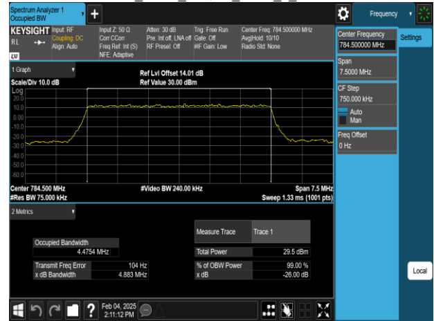
Band13_5MHz_64QAM_RB25_0_CH23255
