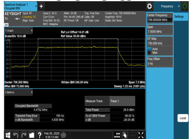
Band17_5MHz_256QAM_RB25_0_CH23755
