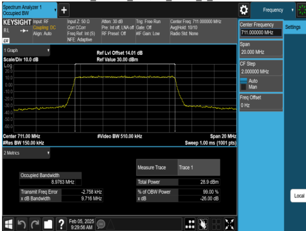
Band17 10MHz_256QAM_RB50_0_CH23800
