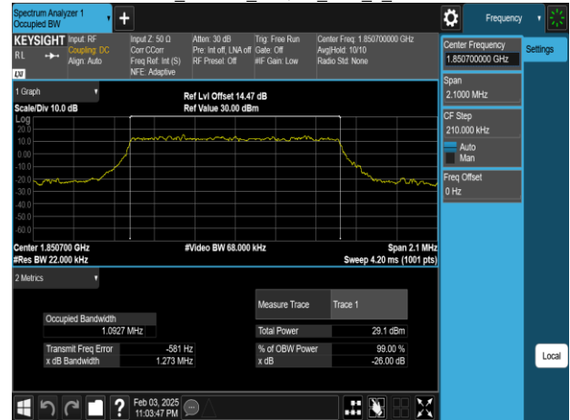
Band25 1.4MHz_64QAM_RB6_0_CH26047
