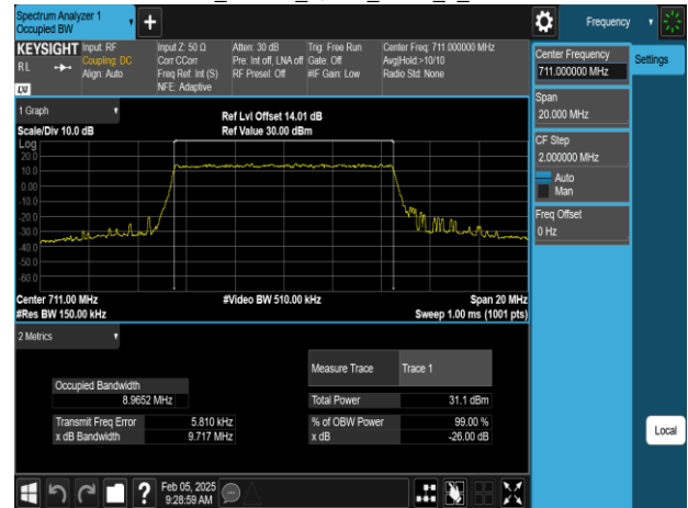
Band17_10MHz_16QAM_RB50_0_CH23800
