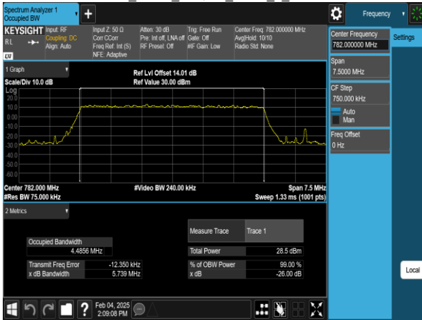
Band13_5MHz_256QAM_RB25_0_CH23230
