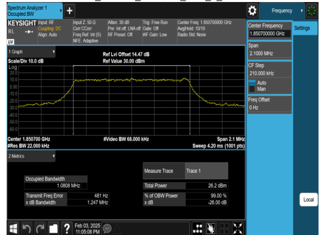
Band25 1.4MHz_256QAM_RB6_0_CH26047
