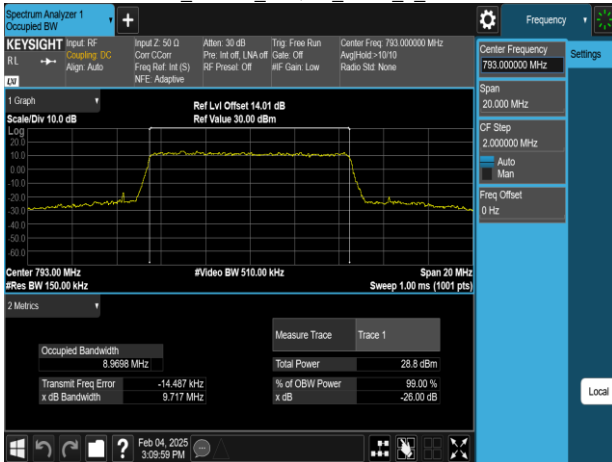
Band14_10MHz_256QAM_RB50_0_CH23330
