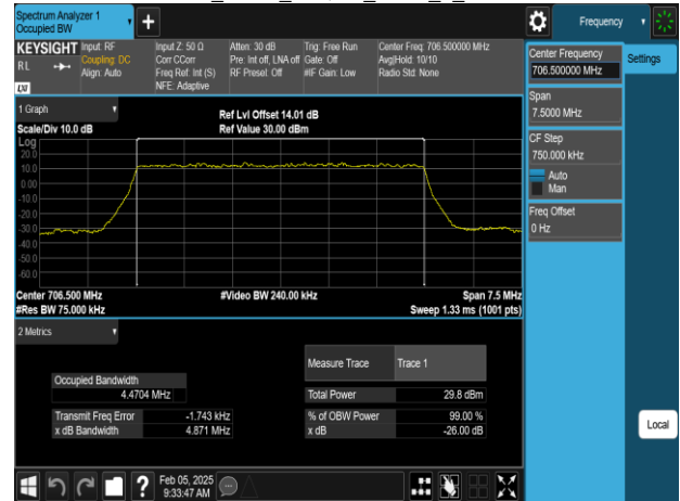
Band17_5MHz_64QAM_RB25_0_CH23755
