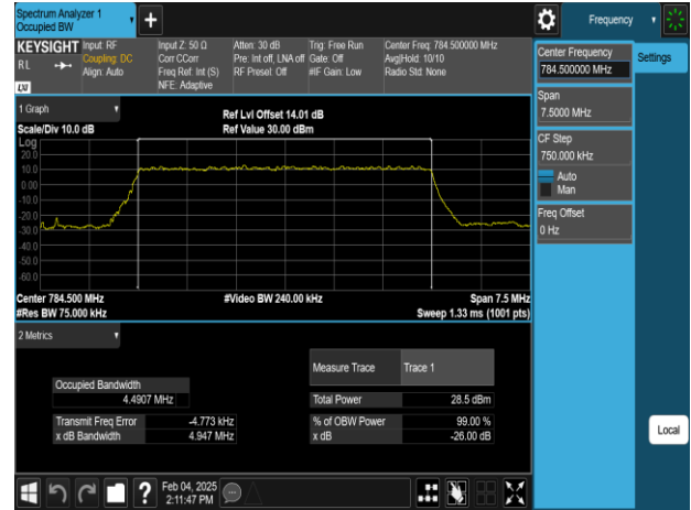
Band13_5MHz_256QAM_RB25_0_CH23255
