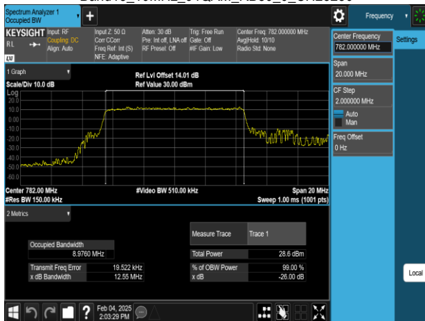
Band13_10MHz_64QAM_RB50_0_CH23230
