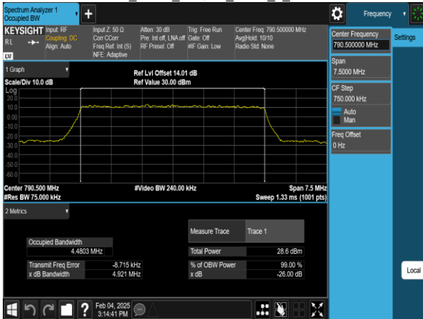
Band14_5MHz_256QAM_RB25_0_CH23305
