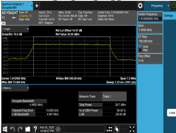
Band25_5MHz_256QAM_RB25_0_CH26665
