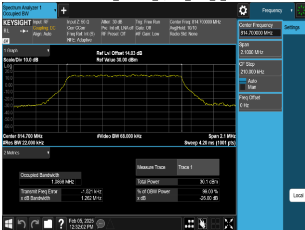
Band26-Part90s 1.4MHz QPSK RB6_0 CH26697
