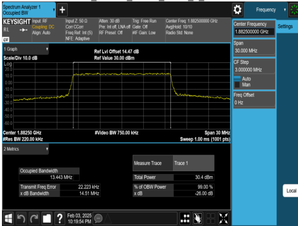
Band25_15MHz_16QAM_RB75_0_CH26365
