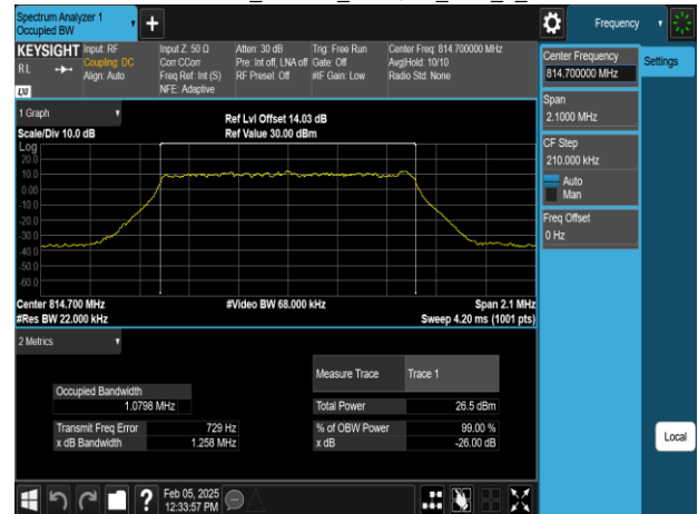
Band26-Part90s 1.4MHz 256QAM RB6_0 CH26697
