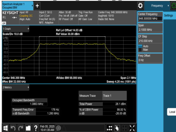
Band26 1.4MHz_256QAM_RB6_0_CH27033
