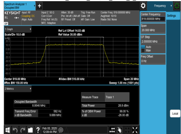
Band26-Part90s_10MHz_256QAM_RB50_0_CH26740
