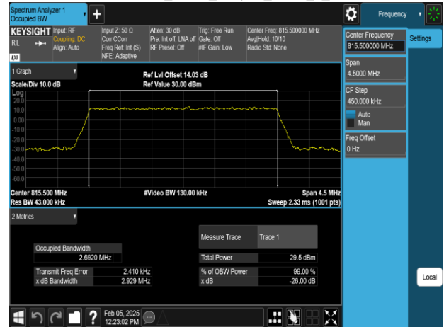
Band26-Part90s_3MHz_64QAM_RB15_0_CH26705
