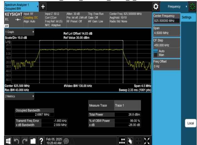
Band26_3MHz_256QAM_RB15_0_CH26805
