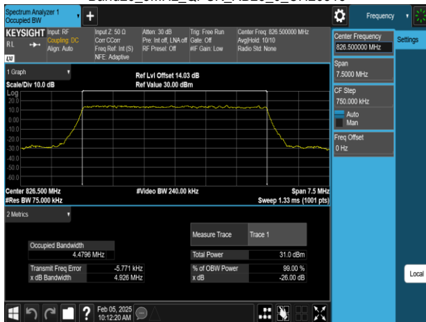
Band26_5MHz_QPSK_RB25_0_CH26815
