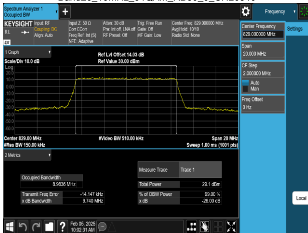
Band26 10MHz_64QAM_RB50_0_CH26840
