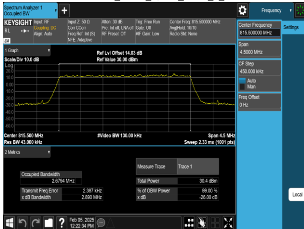
Band26-Part90s_3MHz_QPSK_RB15_0_CH26705
