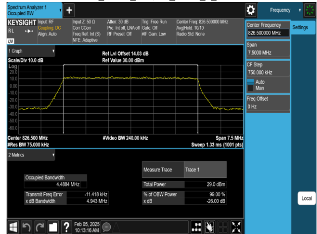
Band26_5MHz_256QAM_RB25_0_CH26815
