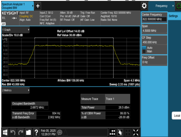
Band26-Part90s_3MHz_256QAM_RB15_0_CH26775
