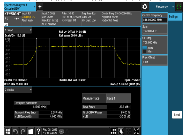
Band26-Part90s_5MHz_256QAM_RB25_0_CH26715
