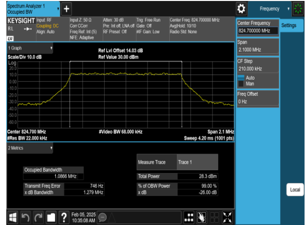
Band26_1.4MHz_256QAM_RB6_0_CH26797
