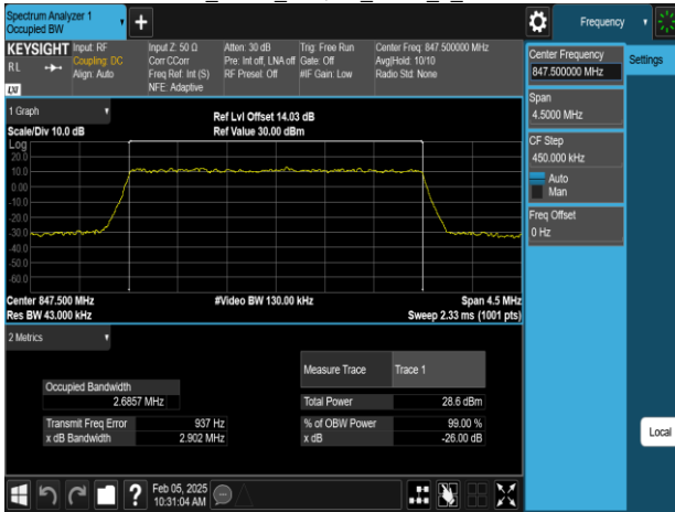
Band26_3MHz_256QAM_RB15_0_CH27025
