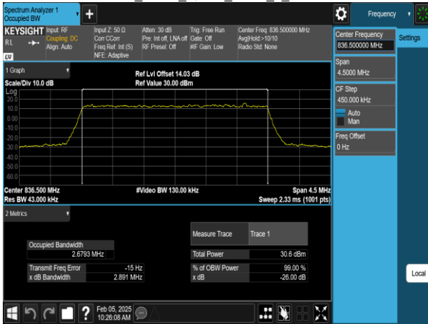
Band26_3MHz_16QAM_RB15_0_CH26915
