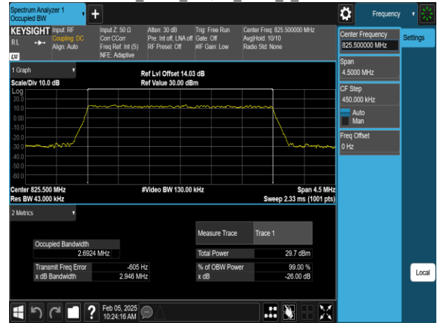
Band26_3MHz_64QAM_RB15_0_CH26805
