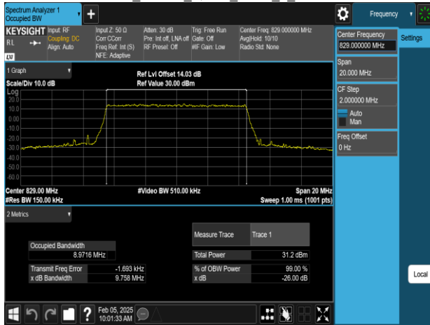
Band26 10MHz_16QAM_RB50_0_CH26840
