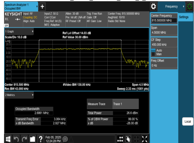
Band26-Part90s_3MHz_256QAM_RB15_0_CH26705
