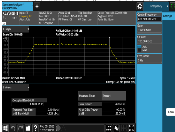
Band26-Part90s_5MHz_256QAM_RB25_0_CH26765
