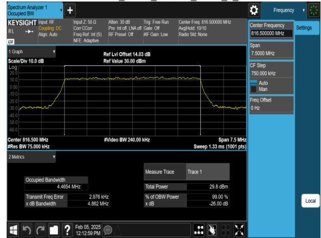
Band26-Part90s_5MHz_64QAM_RB25_0_CH26715
