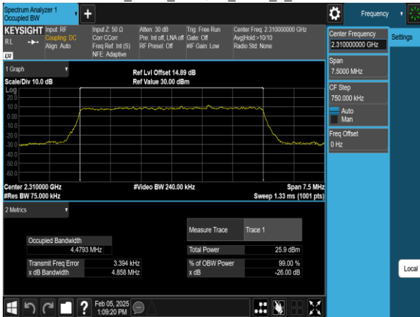
Band30_5MHz_QPSK_RB25_0_CH27735
