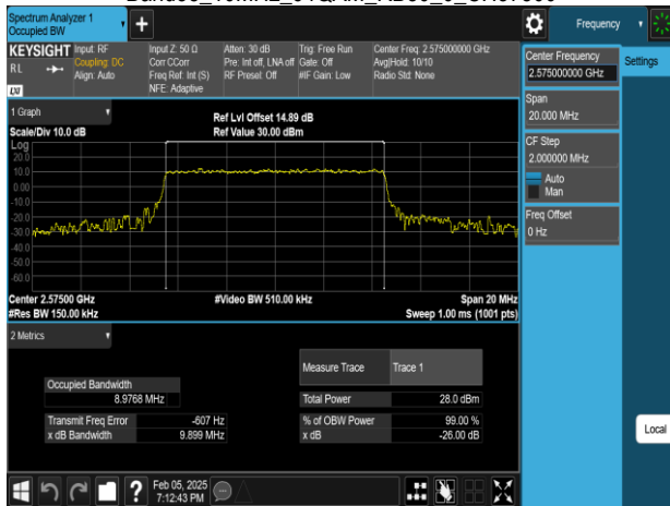
Band38_10MHz_256QAM_RB50_0_CH37800
