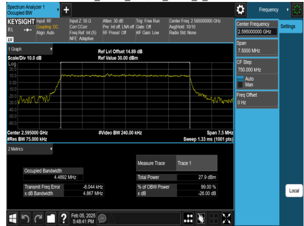
Band38 5MHz 256QAM RB25_0 CH38000
