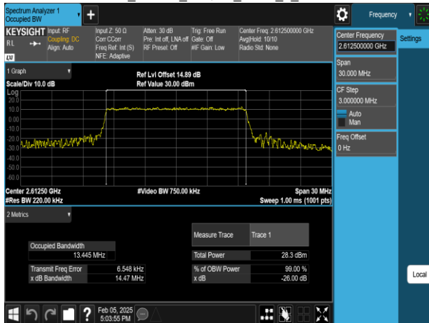
Band38_15MHz_64QAM_RB75_0_CH38175
