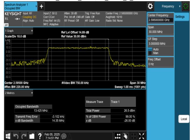
Band38_15MHz_256QAM_RB75_0_CH38000
