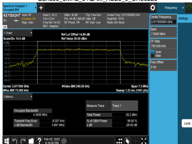
Band38_5MHz_64QAM_RB25_0_CH38225
