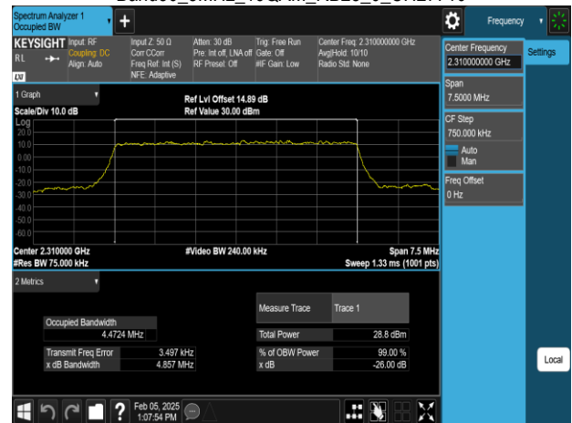
Band30_5MHz_16QAM_RB25_0_CH27710
