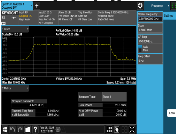
Band30_5MHz_64QAM_RB25_0_CH27685
