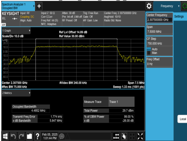
Band30_5MHz_16QAM_RB25_0_CH27685
