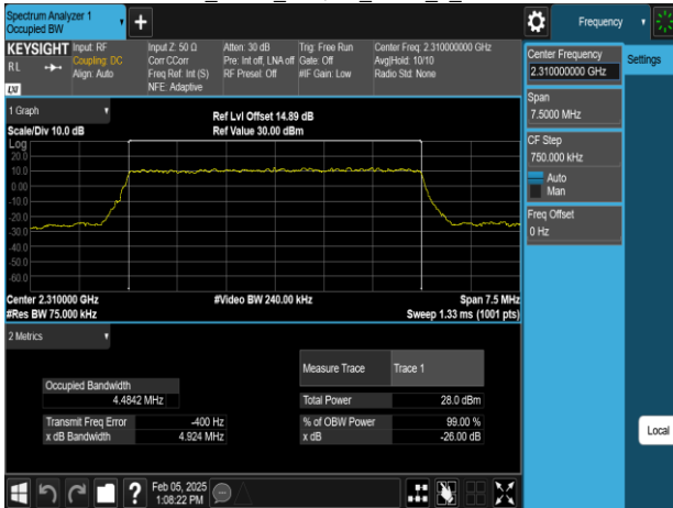
Band30_5MHz_256QAM_RB25_0_CH27710
