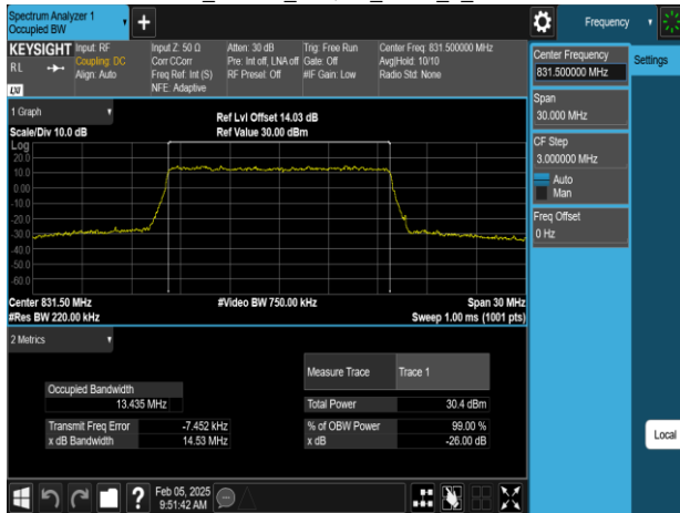
Band26 15MHz_64QAM_RB75_0_CH26865
