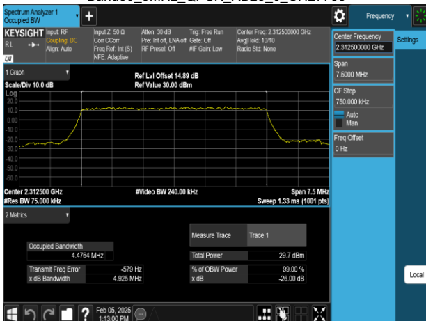
Band30_5MHz_QPSK_RB25_0_CH27735
