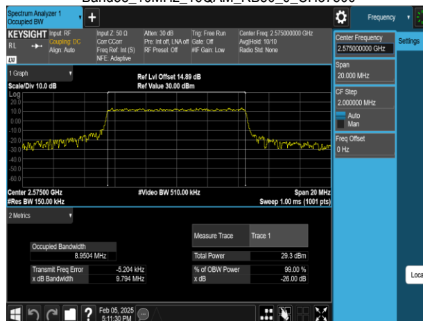
Band38_10MHz_16QAM_RB50_0_CH37800
