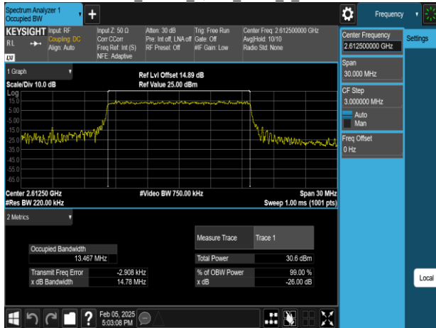
Band38_15MHz_16QAM_RB75_0_CH38175
