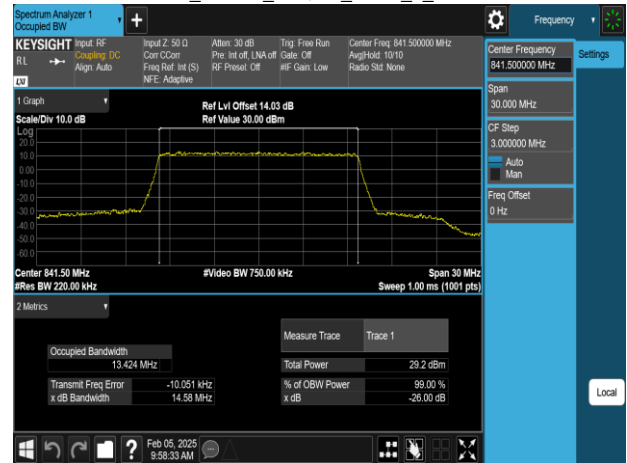
Band26_15MHz_256QAM_RB75_0_CH26965
