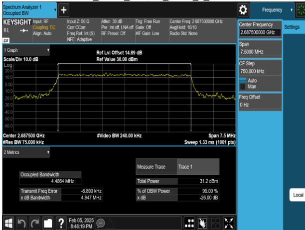
Band41_5MHz_256QAM_RB25_0_CH41565
