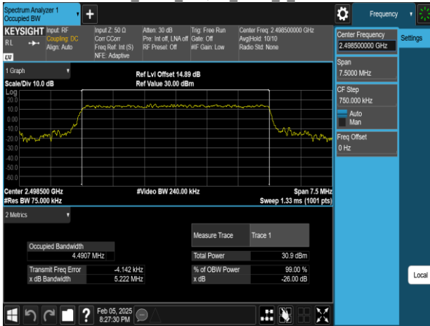
Band41_5MHz_256QAM_RB25_0_CH39675
