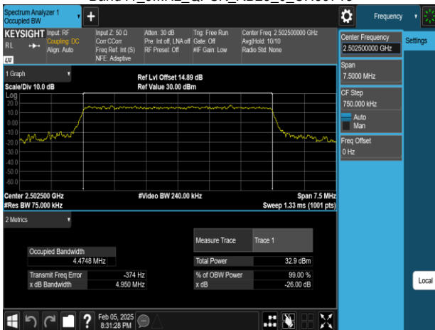
Band41_5MHz_QPSK_RB25_0_CH39715
