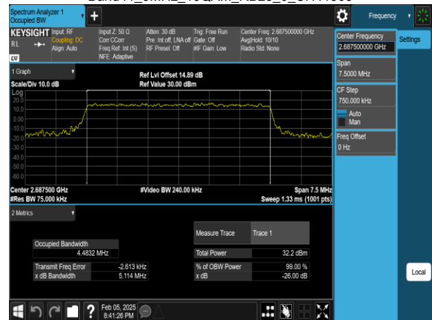
Band41_5MHz_16QAM_RB25_0_CH41565
