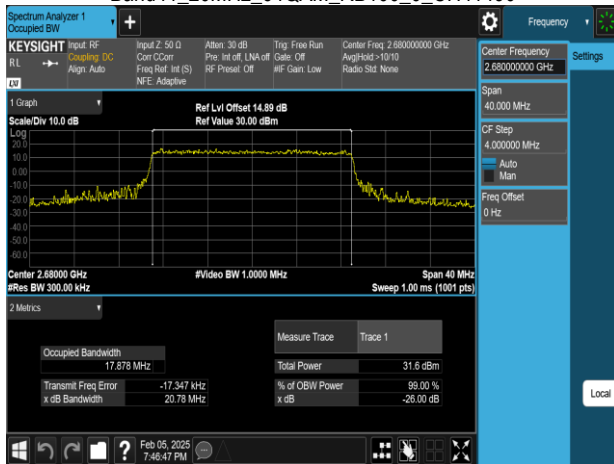
Band41_20MHz_256QAM_RB100_0_CH41490
