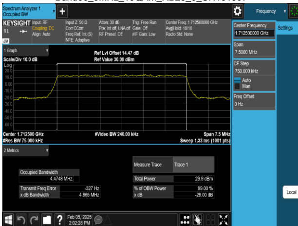
Band66_5MHz_16QAM_RB25_0_CH131997
