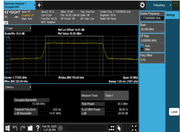
Band66_15MHz_64QAM_RB75_0_CH132597
