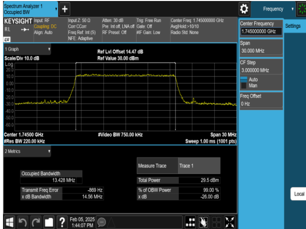
Band66_15MHz_256QAM_RB75_0_CH132322
