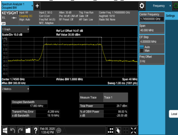
Band66_20MHz_256QAM_RB100_0_CH132322
