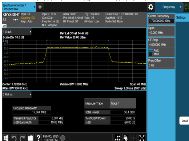
Band66 20MHz_16QAM_RB100_0_CH132072
