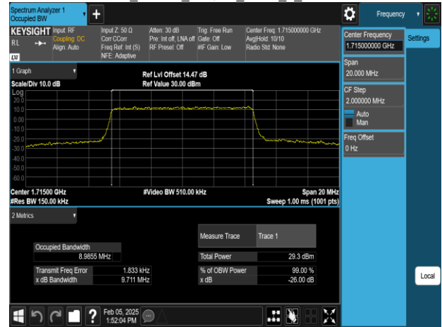
Band66_10MHz_256QAM_RB50_0_CH132022
