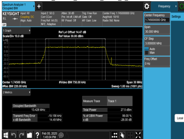
Band66_15MHz_256QAM_RB75_0_CH132322
