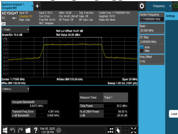
Band66_10MHz_16QAM_RB50_0_CH132022
