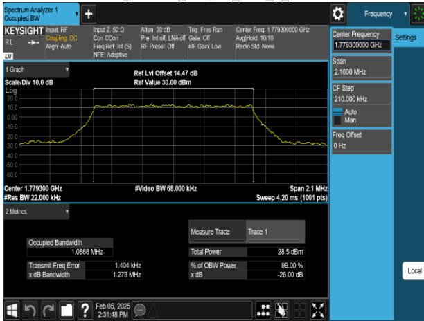
Band66 1.4MHz_256QAM_RB6_0_CH132665
