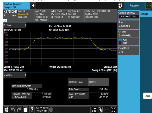
Band66_1.4MHz_256QAM_RB6_0_CH131979
