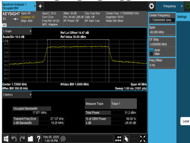
Band66 20MHz_16QAM_RB100_0_CH132072
