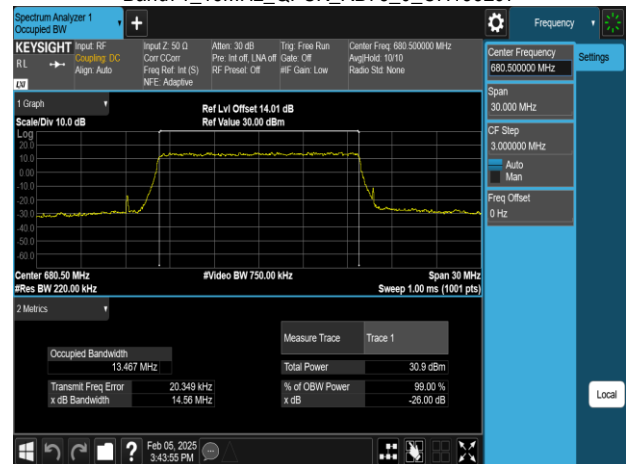
Band71_15MHz_QPSK_RB75_0_CH133297
