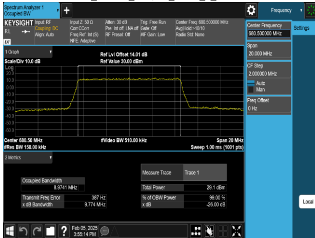
Band71_10MHz_256QAM_RB50_0_CH133297
