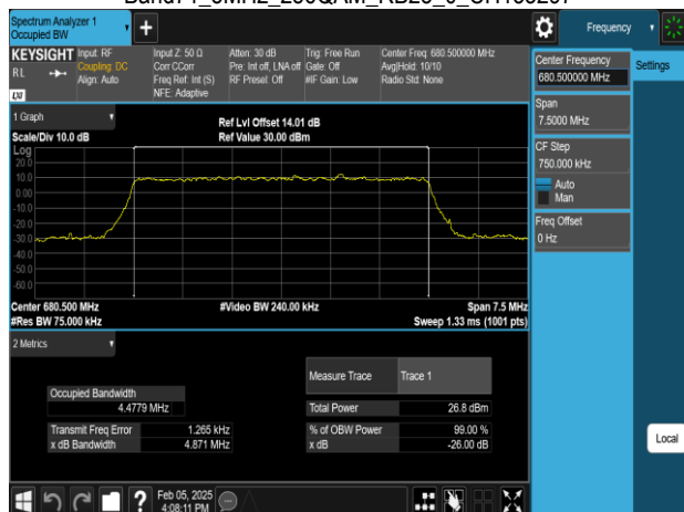
Band71_5MHz_256QAM_RB25_0_CH133297
