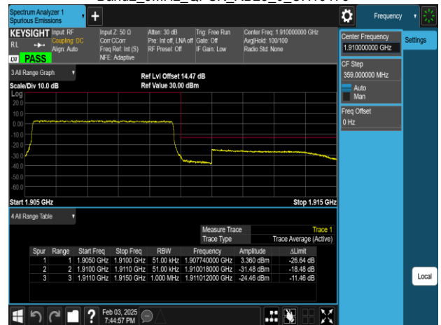
Band2_5MHz_QPSK_RB25_0_CH19175
