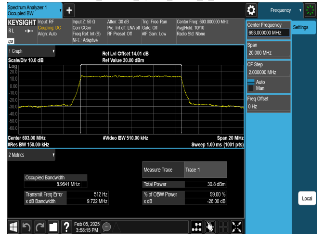
Band71_10MHz_16QAM_RB50_0_CH133422
