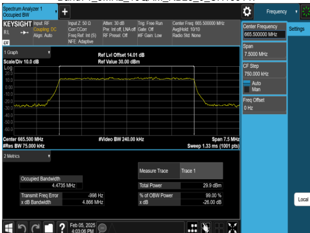
Band71_5MHz_16QAM_RB25_0_CH133147
