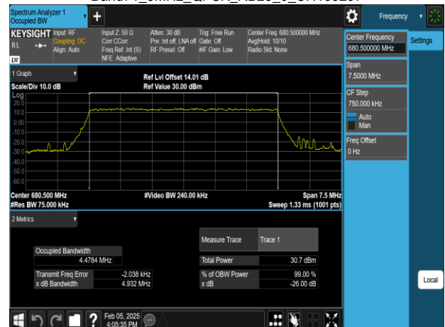
Band71_5MHz_QPSK_RB25_0_CH133297
