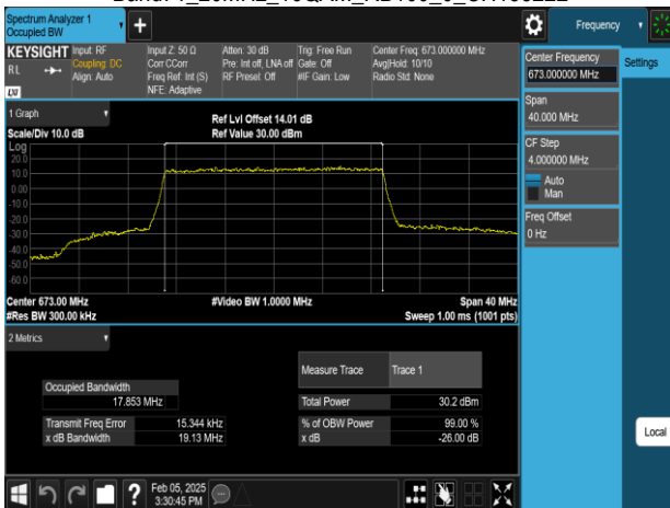
Band71_20MHz_16QAM_RB100_0_CH133222
