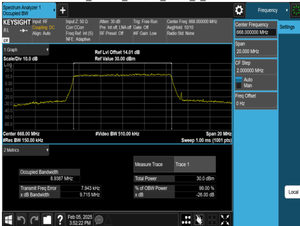
Band71_10MHz_16QAM_RB50_0_CH133172
