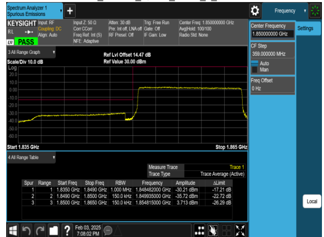
Band2_15MHz_QPSK_RB75_0_CH18675
