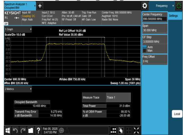
Band71_15MHz_16QAM_RB75_0_CH133397
