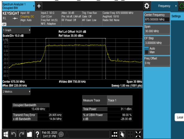
Band71_15MHz_16QAM_RB75_0_CH133197
