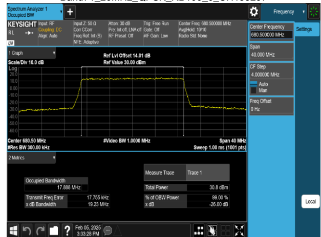
Band71_20MHz_QPSK_RB100_0_CH133297
