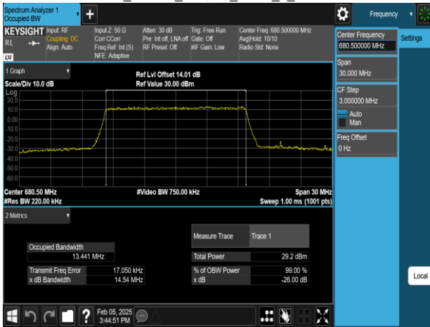
Band71_15MHz_256QAM_RB75_0_CH133297
