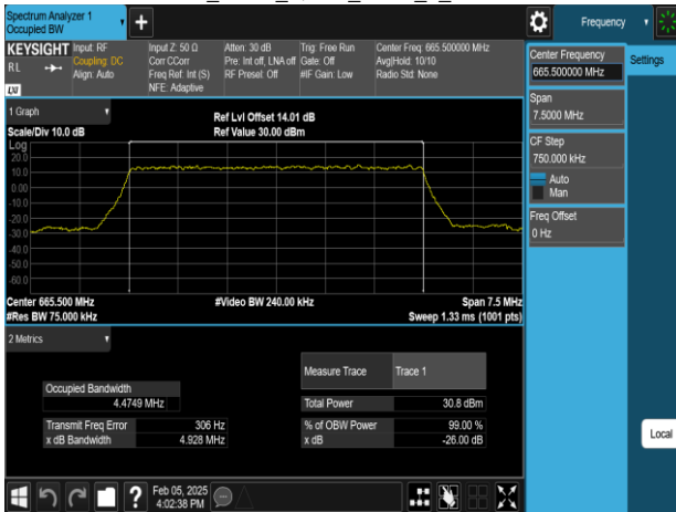
Band71_5MHz_16QAM_RB25_0_CH133147
