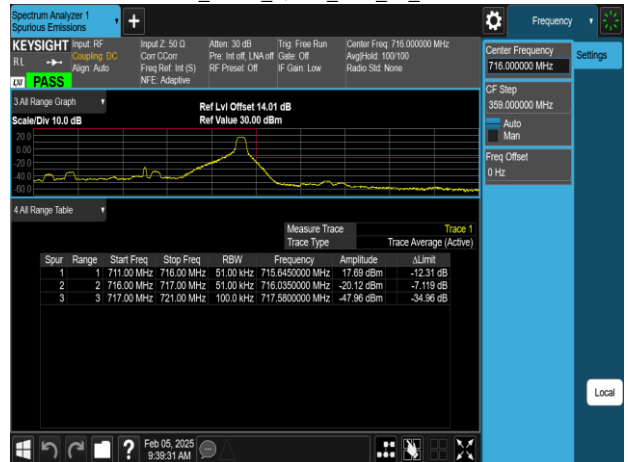
Band17_5MHz_QPSK_RB1_24_CH23825
