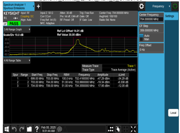
Band17_5MHz_QPSK_RB25_0_CH23755
