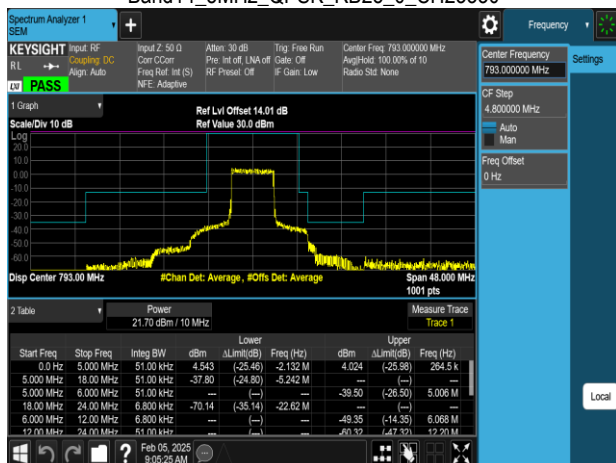
Band14_5MHz_QPSK_RB25_0_CH23330
