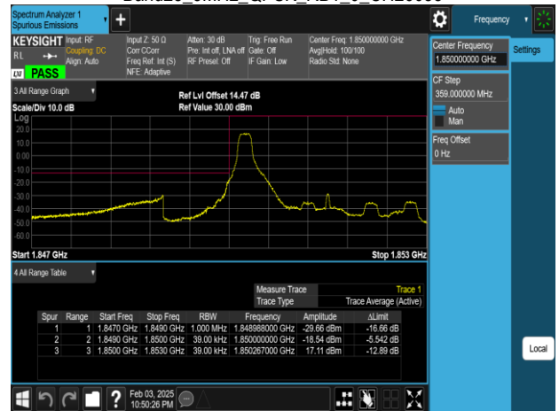
Band25_3MHz_QPSK_RB15_0_CH26055
