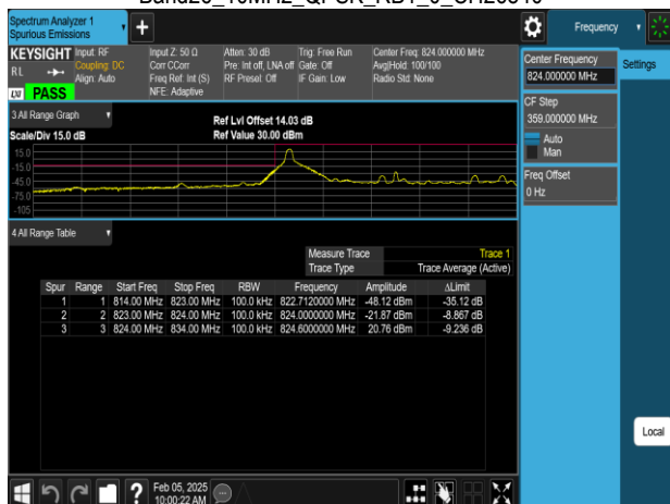
Band26_10MHz_QPSK_RB1_0_CH26840
