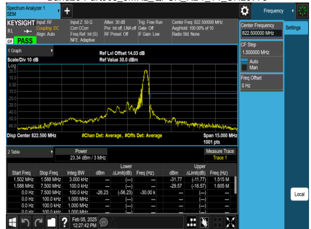
Band26-Part90s_3MHz_QPSK_RB15_0_CH26775
