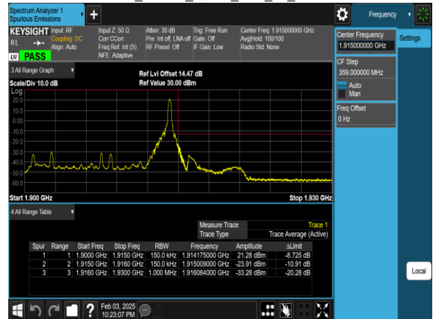
Band25_15MHz_QPSK_RB1_74_CH26615
