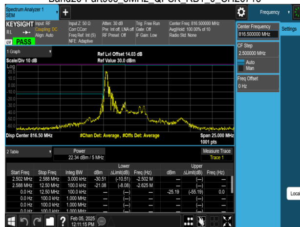
Band26-Part90s_5MHz_QPSK_RB25_0_CH26715
