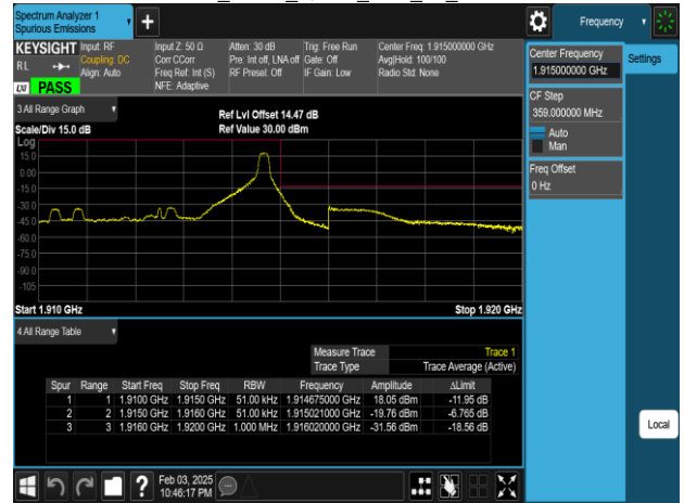
Band25_5MHz_QPSK_RB25_0_CH26665
