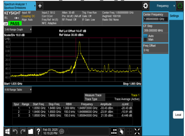
Band25_15MHz_QPSK_RB75_0_CH26115
