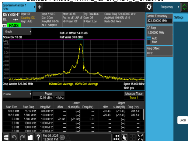
Band26-Part90s_1.4MHz_QPSK_RB6_0_CH26783
