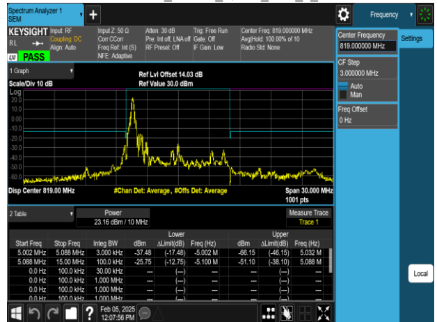
Band26-Part90s_10MHz_QPSK_RB1_0_CH26740
