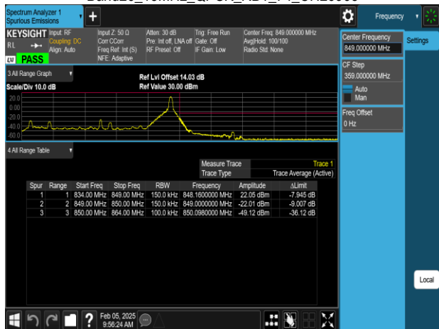
Band26 15MHz_QPSK_RB1_74_CH26965
