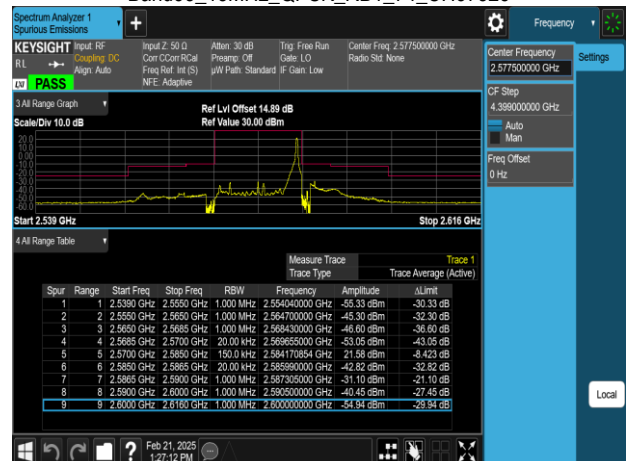
Band38_15MHz_QPSK_RB1_74_CH37825
