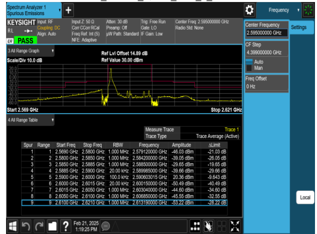
Band38_10MHz_QPSK_RB1_49_CH38000
