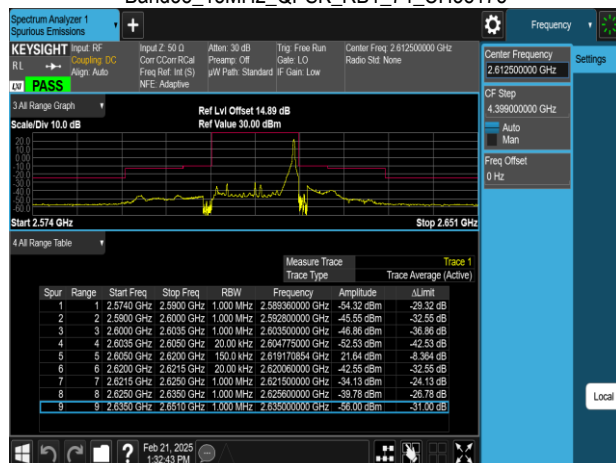
Band38_15MHz_QPSK_RB1_74_CH38175
