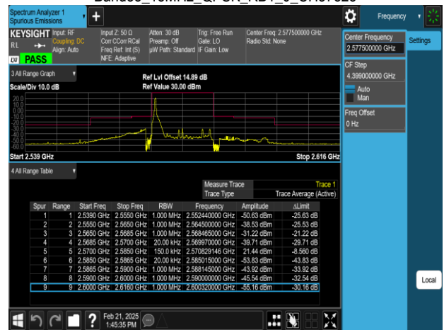
Band38_15MHz_QPSK_RB1_74_CH37825
