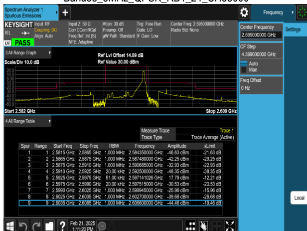
Band38_5MHz_QPSK_RB1_24_CH38000
