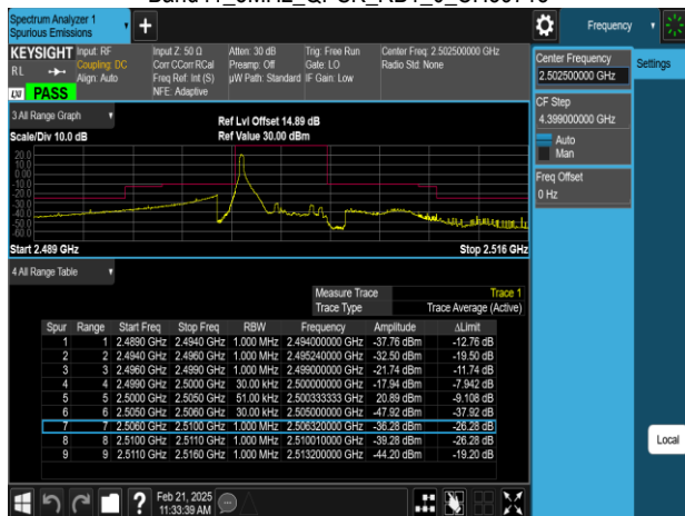
Band41 5MHz QPSK RB1_24 CH39715
