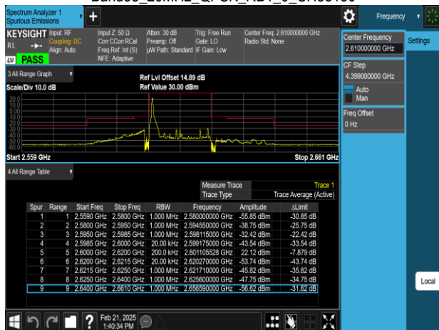
Band38 20MHz QPSK RB1_99 CH38150
