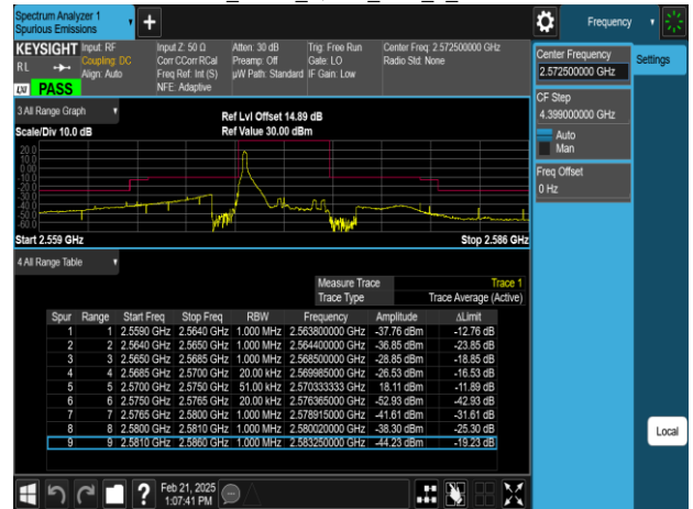
Band38_5MHz_QPSK_RB1_24_CH37775
