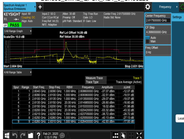
Band38_5MHz_QPSK_RB1_24_CH38225
