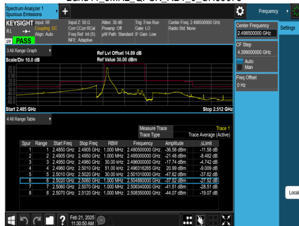
Band41 5MHz QPSK RB1_24 CH39675
