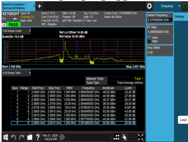
Band38_10MHz_QPSK_RB1_49_CH37800
