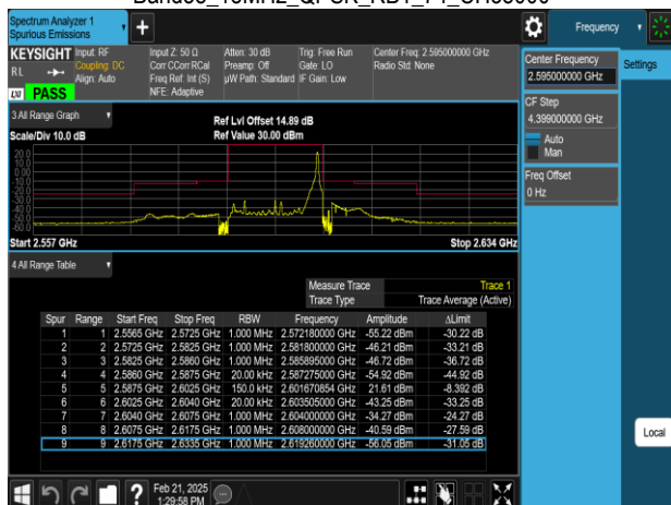
Band38_15MHz_QPSK_RB1_74_CH38000
