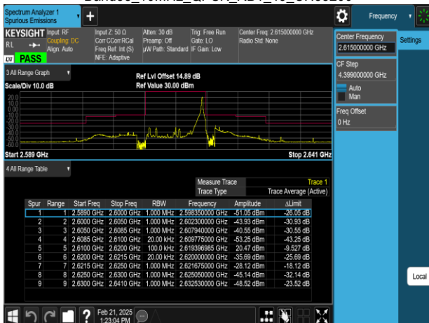
Band38_10MHz_QPSK_RB1_49_CH38200
