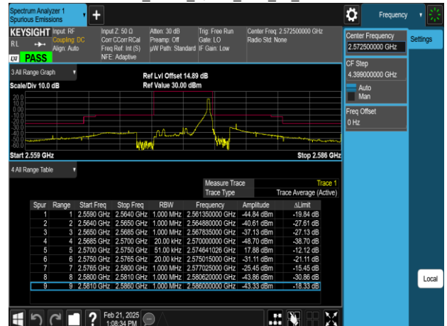
Band38_5MHz_QPSK_RB1_24_CH37775
