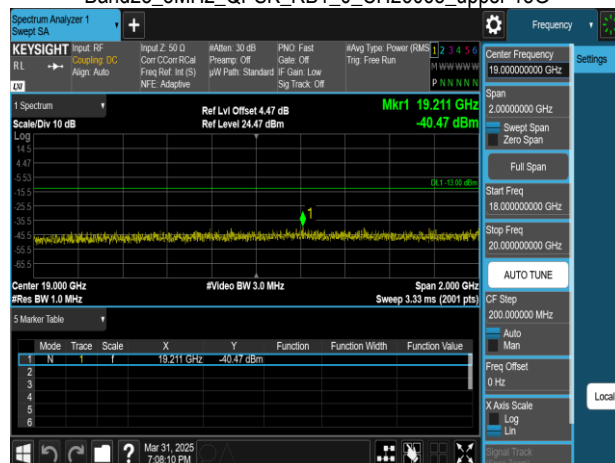
Band25_5MHz_QPSK_RB1_0_CH26065_upper 18G
