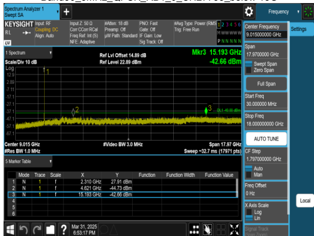
Band30_5MHz_QPSK_RB1_0_CH27735_below 18G
