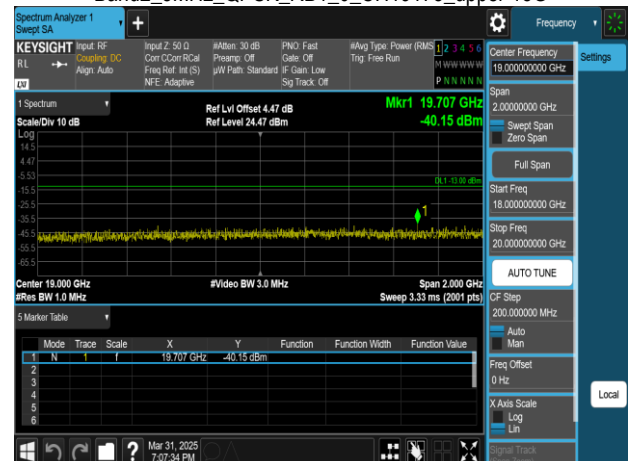
Band2_5MHz_QPSK_RB1_0_CH19175_upper 18G
