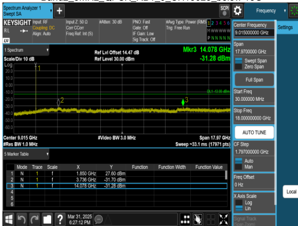
Band2_5MHz_QPSK_RB1_0_CH18625_upper 18G
