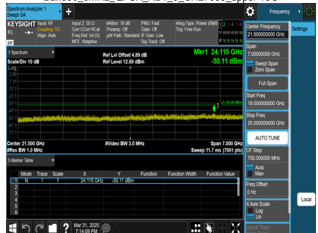
Band30_5MHz_QPSK_RB1_0_CH27685_upper 18G
