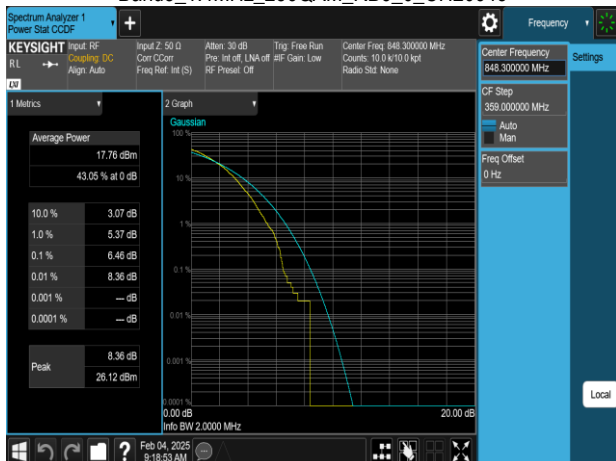
Band5 1.4MHz_256QAM_RB6_0_CH20643
