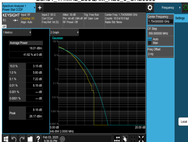
Band4 1.4MHz_256QAM_RB6_0_CH20393
