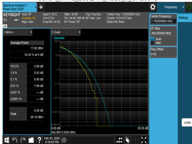
Band4_5MHz_256QAM_RB25_0_CH20375
