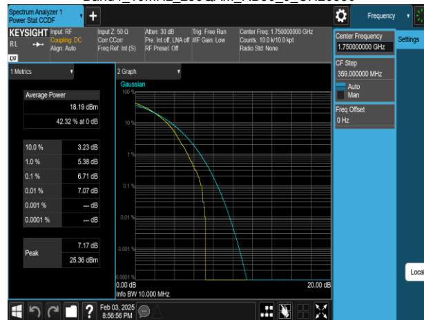
Band4_10MHz_256QAM_RB50_0_CH20350
