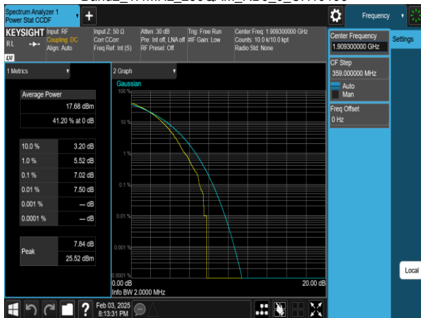
Band2_1.4MHz_256QAM_RB6_0_CH19193
