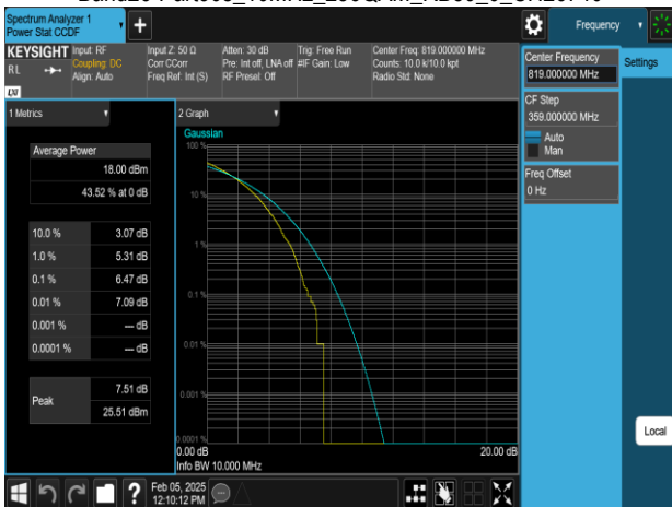
Band26-Part90s_10MHz_256QAM_RB50_0_CH26740
