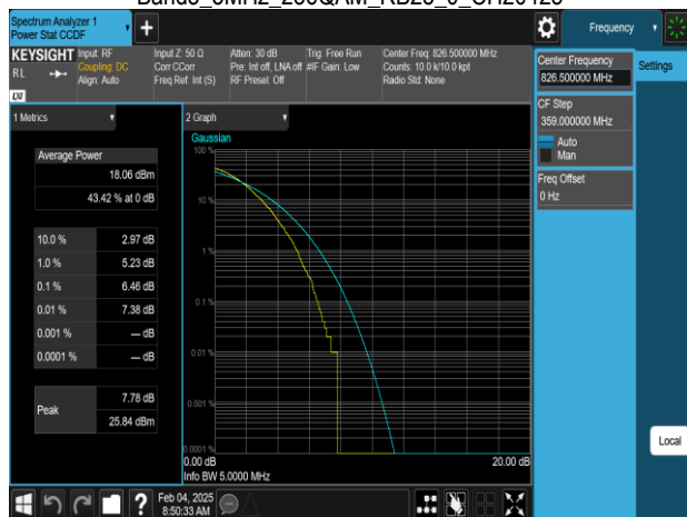
Band5_5MHz_256QAM_RB25_0_CH20525
