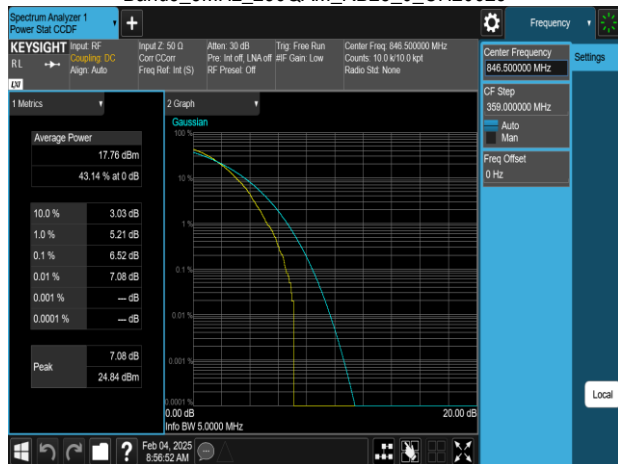
Band5_5MHz_256QAM_RB25_0_CH20625
