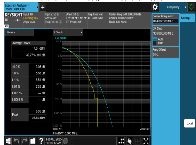
Band26_10MHz_256QAM_RB50_0_CH26990
