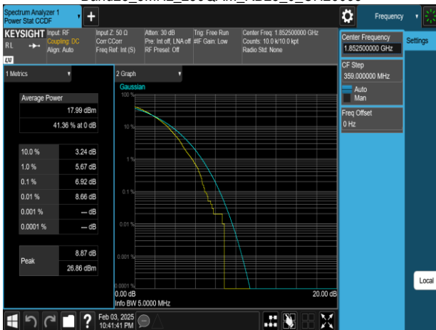
Band25_5MHz_256QAM_RB25_0_CH26065
