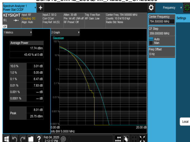
Band13_5MHz_256QAM_RB25_0_CH23255
