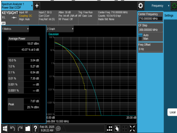
Band17_10MHz_256QAM_RB50_0_CH23800
