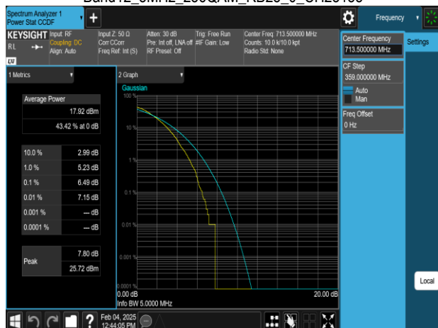
Band12_5MHz_256QAM_RB25_0_CH23155
