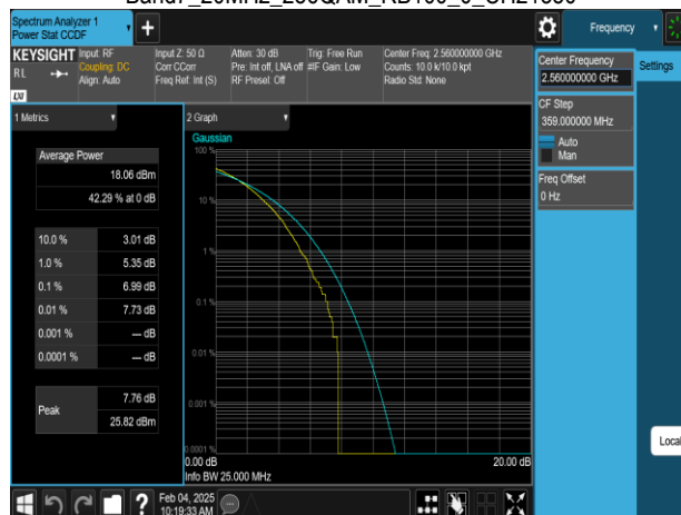
Band7_20MHz_256QAM_RB100_0_CH21350
