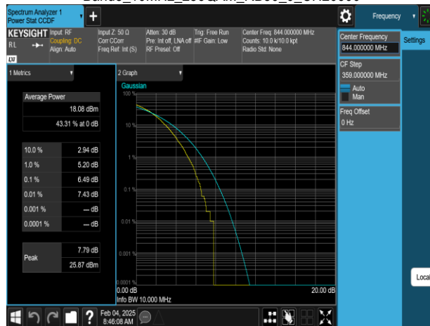
Band5_10MHz_256QAM_RB50_0_CH20600
