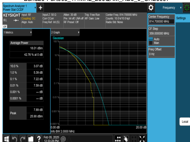
Band26-Part90s_1.4MHz_256QAM_RB6_0_CH26697
