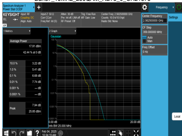
Band7_15MHz_256QAM_RB75_0_CH21375
