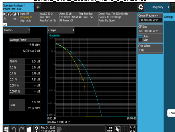
Band12_3MHz_256QAM_RB15_0_CH23165
