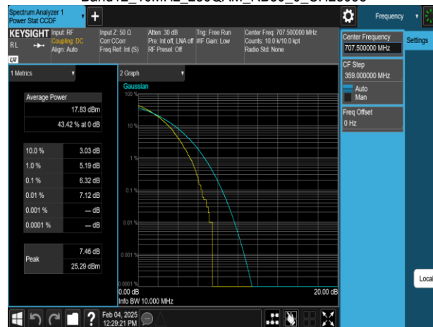
Band12_10MHz_256QAM_RB50_0_CH23130
