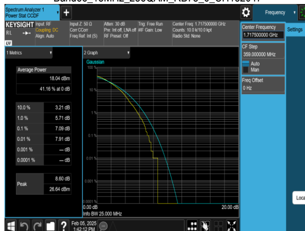
Band66_15MHz_256QAM_RB75_0_CH132047
