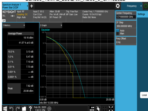
Band66_10MHz_256QAM_RB50_0_CH132022
