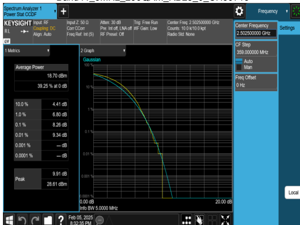
Band41 5MHz_256QAM_RB25_0_CH39715
