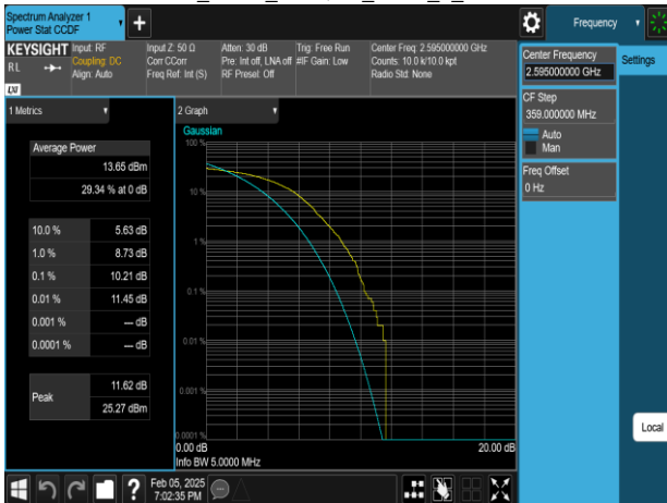
Band38_5MHz_256QAM_RB25_0_CH38000
