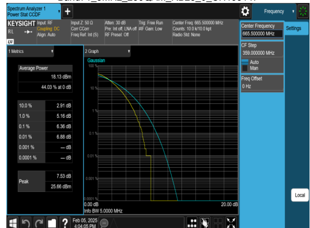
Band71 5MHz_256QAM_RB25_0_CH131347
