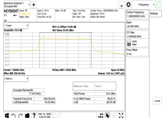
Band2_20MHz_DFT_s_OFDM_SCS15kHz_16QAM_RB100_0_CH380000
