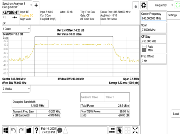
Band5_5MHz_DFT_s_OFDM_SCS15kHz_64QAM_RB25_0_CH169300
