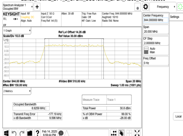
Band5_10MHz_DFT_s_OFDM_SCS15kHz_BPSK_RB50_0_CH168800
