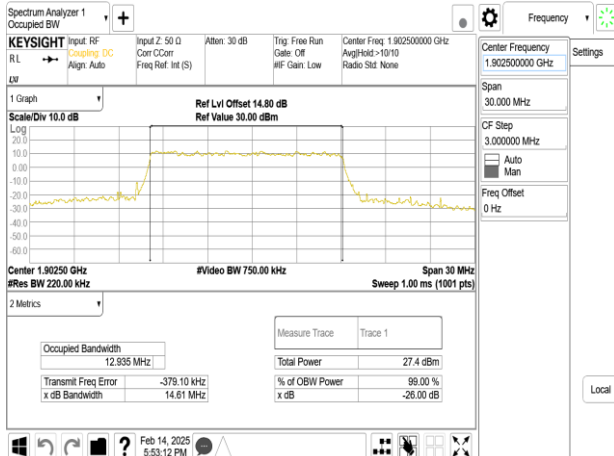
Band2_15MHz_DFT_s_OFDM_SCS30kHz_256QAM_RB36_0_CH380500
