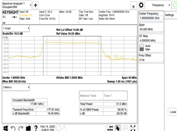
Band2_20MHz_DFT_s_OFDM_SCS30kHz_BPSK_RB50_0_CH380000
