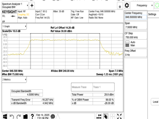
Band5_5MHz_DFT_s_OFDM_SCS15kHz_QPSK_RB25_0_CH169300
