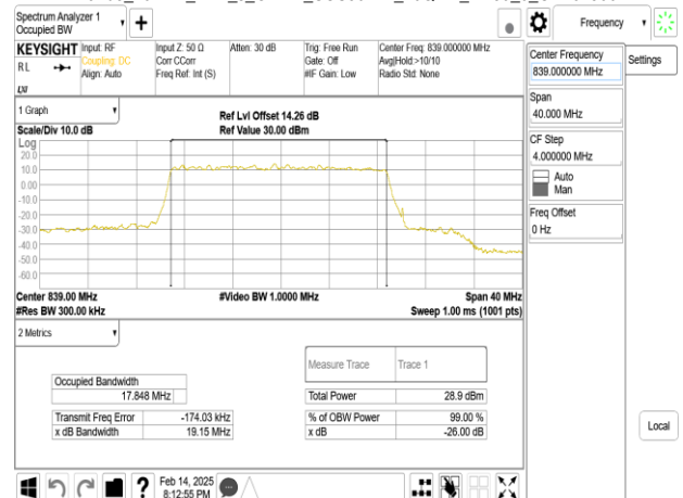
Band5_20MHz_DFT_s_OFDM_SCS30kHz_16QAM_RB50_0_CH167800
