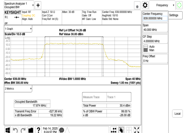
Band5_20MHz_DFT_s_OFDM_SCS15kHz_QPSK_RB100_0_CH167800
