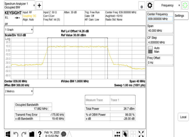
Band5_20MHz_DFT_s_OFDM_SCS30kHz_256QAM_RB50_0_CH167800
