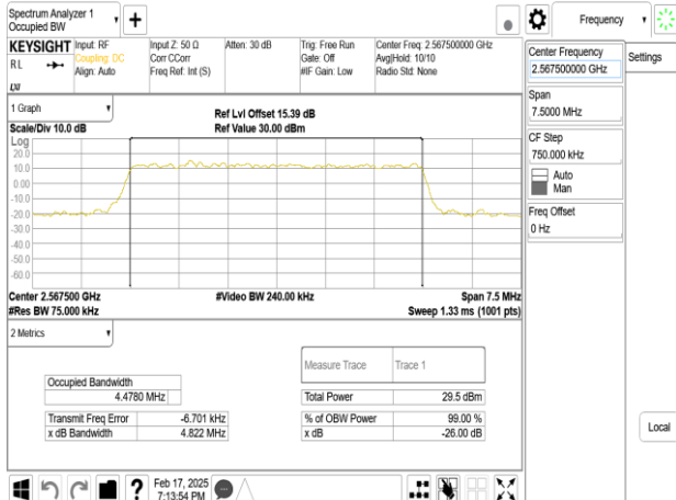
Band7_5MHz_DFT_s_OFDM_SCS15kHz_16QAM_RB25_0_CH513500
