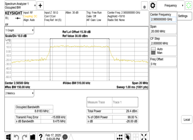
Band7_10MHz_DFT_s_OFDM_SCS30kHz_64QAM_RB24_0_CH513000
