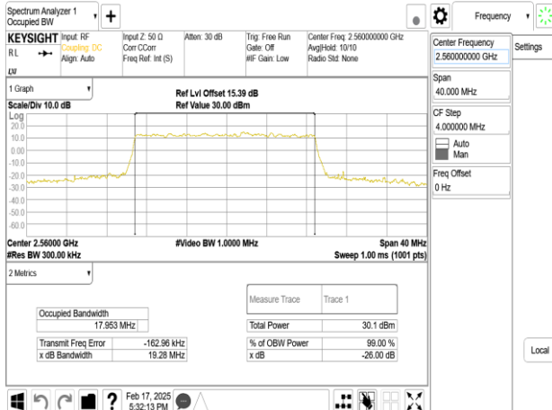
Band7_20MHz_DFT_s_OFDM_SCS30kHz_16QAM_RB50_0_CH512000
