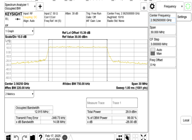
Band7_15MHz_DFT_s_OFDM_SCS30kHz_64QAM_RB36_0_CH512500
