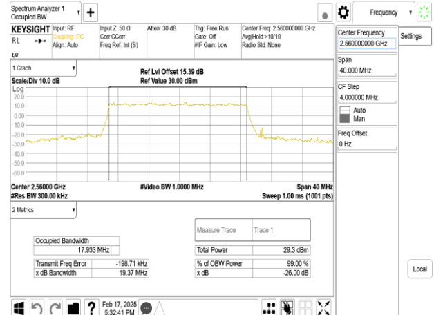
Band7_20MHz_DFT_s_OFDM_SCS30kHz_64QAM_RB50_0_CH512000
