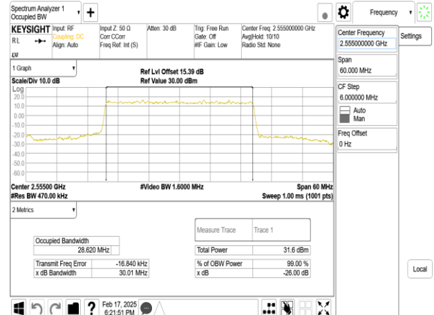
Band7_30MHz_DFT_s_OFDM_SCS15kHz_BPSK_RB160_0_CH511000
