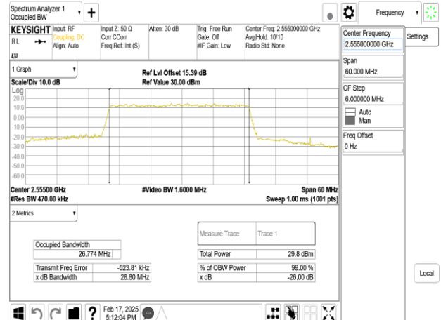
Band7_30MHz_DFT_s_OFDM_SCS30kHz_64QAM_RB75_0_CH511000
