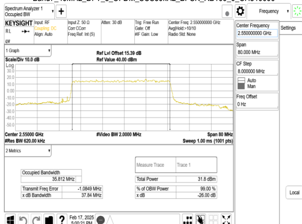
Band7_40MHz_DFT_s_OFDM_SCS30kHz_BPSK_RB100_0_CH510000
