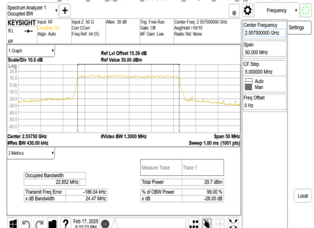
Band7_25MHz_DFT_s_OFDM_SCS30kHz_64QAM_RB64_0_CH511500
