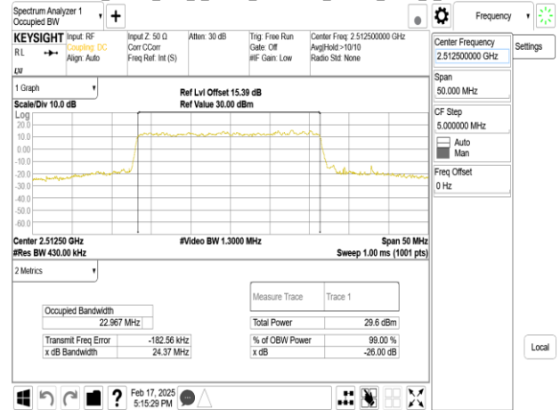
Band7_25MHz_DFT_s_OFDM_SCS30kHz_64QAM_RB64_0_CH057000
