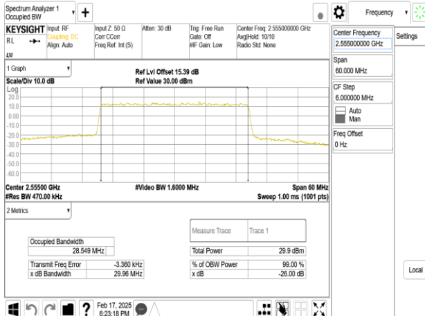
Band7_30MHz_DFT_s_OFDM_SCS15kHz_64QAM_RB160_0_CH511000
