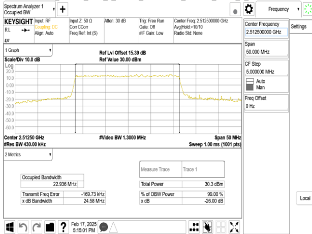
Band7_25MHz_DFT_s_OFDM_SCS30kHz_16QAM_RB64_0_CH057000
