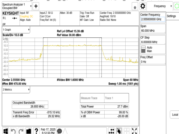
Band7_30MHz_DFT_s_OFDM_SCS30kHz_256QAM_RB75_0_CH511000
