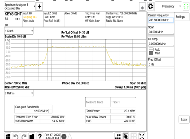
Band12_15MHz_DFT_s_OFDM_SCS30kHz_16QAM_RB36_0_CH141700
