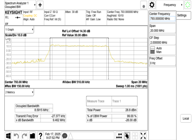
Band14_10MHz_DFT_s_OFDM_SCS30kHz_64QAM_RB24_0_CH158600
