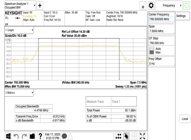
Band14_5MHz_DFT_s_OFDM_SCS15kHz_QPSK_RB25_0_CH159100
