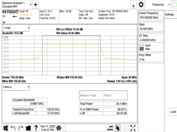
Band14_10MHz_DFT_s_OFDM_SCS30kHz_BPSK_RB24_0_CH158600
