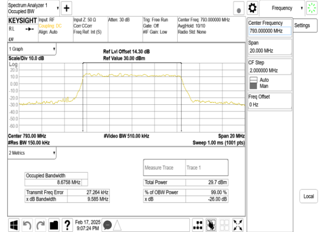
Band14_10MHz_DFT_s_OFDM_SCS30kHz_16QAM_RB24_0_CH158600
