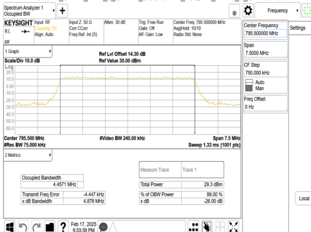
Band14_5MHz_DFT_s_OFDM_SCS15kHz_16QAM_RB25_0_CH159100
