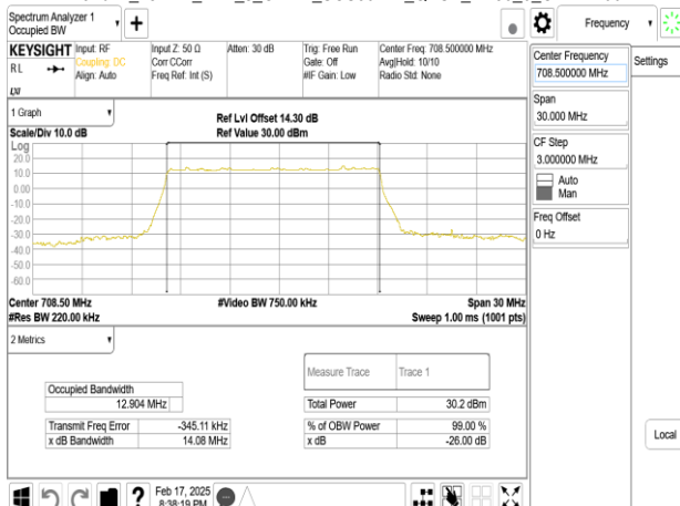
Band12_15MHz_DFT_s_OFDM_SCS30kHz_QPSK_RB36_0_CH141700
