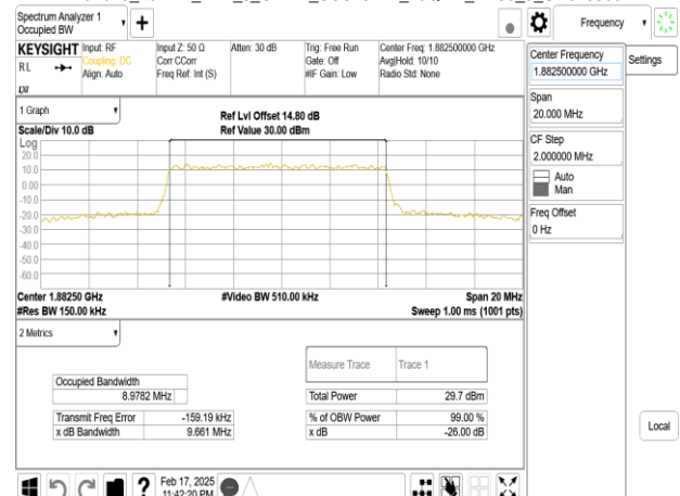
Band25_10MHz_DFT_s_OFDM_SCS15kHz_16QAM_RB50_0_CH376500
