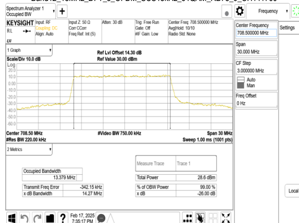
Band12_15MHz_DFT_s_OFDM_SCS15kHz_64QAM_RB75_0_CH141700
