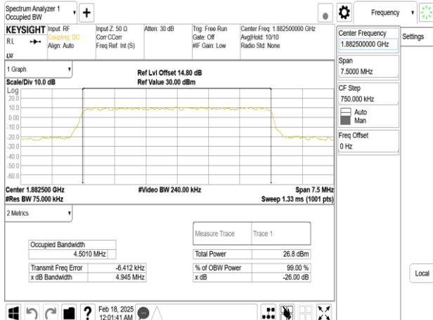
Band25_5MHz_DFT_s_OFDM_SCS15kHz_256QAM_RB25_0_CH376500
