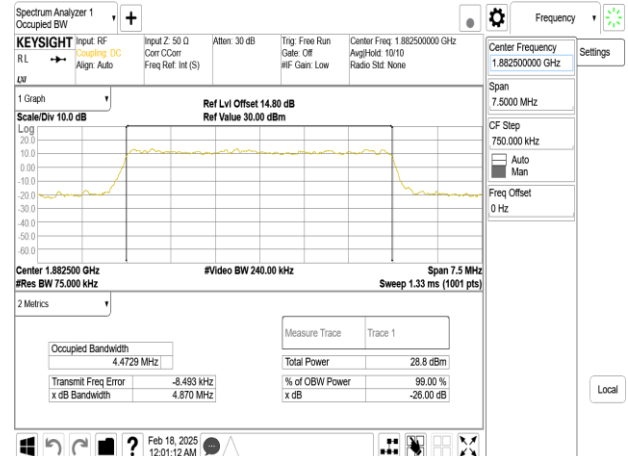
Band25_5MHz_DFT_s_OFDM_SCS15kHz_64QAM_RB25_0_CH376500
