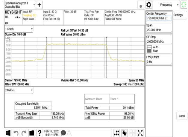
Band14_10MHz_DFT_s_OFDM_SCS15kHz_16QAM_RB50_0_CH158600
