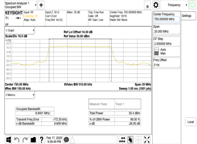
Band14_10MHz_DFT_s_OFDM_SCS15kHz_QPSK_RB50_0_CH158600
