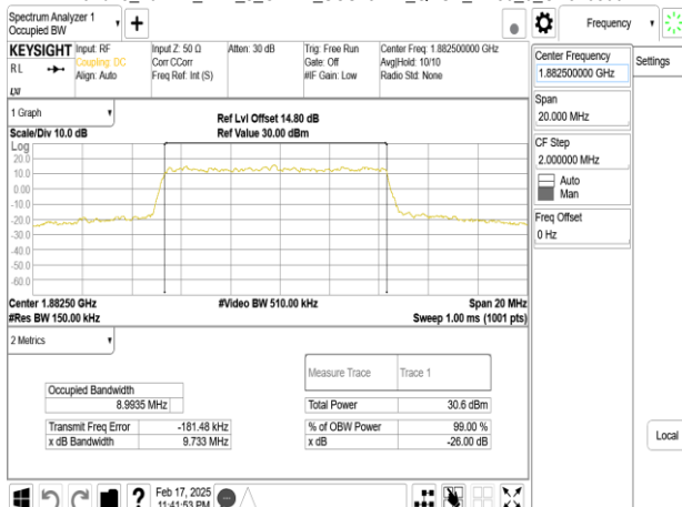
Band25_10MHz_DFT_s_OFDM_SCS15kHz_QPSK_RB50_0_CH376500
