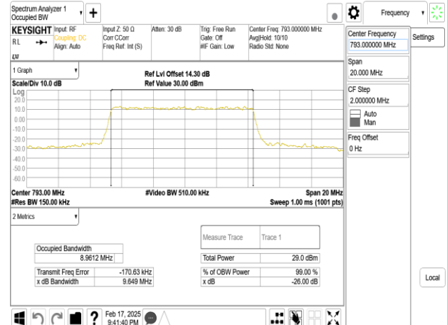
Band14_10MHz_DFT_s_OFDM_SCS15kHz_16QAM_RB50_0_CH158600
