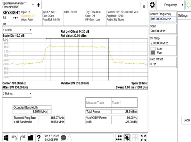
Band14_10MHz_DFT_s_OFDM_SCS15kHz_256QAM_RB50_0_CH158600
