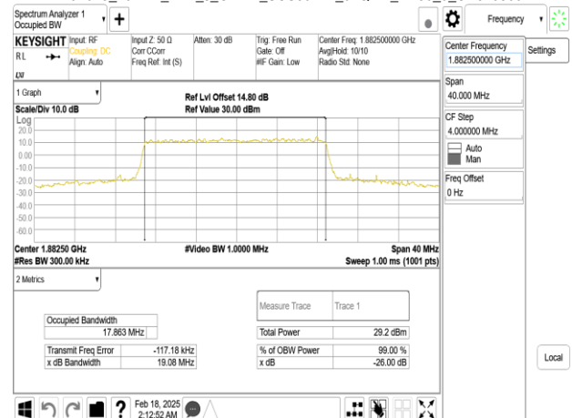
Band25_20MHz_DFT_s_OFDM_SCS30kHz_64QAM_RB50_0_CH376500
