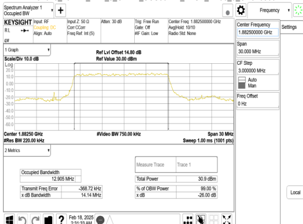
Band25_15MHz_DFT_s_OFDM_SCS30kHz_BPSK_RB36_0_CH376500
