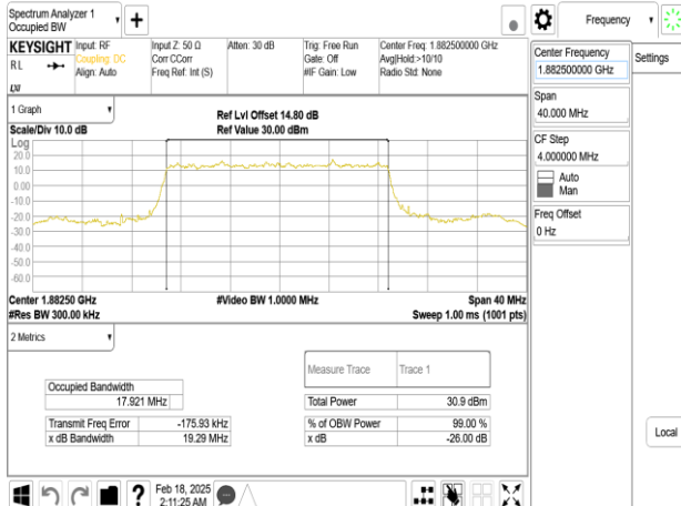
Band25_20MHz_DFT_s_OFDM_SCS30kHz_BPSK_RB50_0_CH376500
