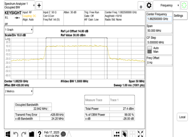
Band25_25MHz_DFT_s_OFDM_SCS15kHz_256QAM_RB128_0_CH376500
