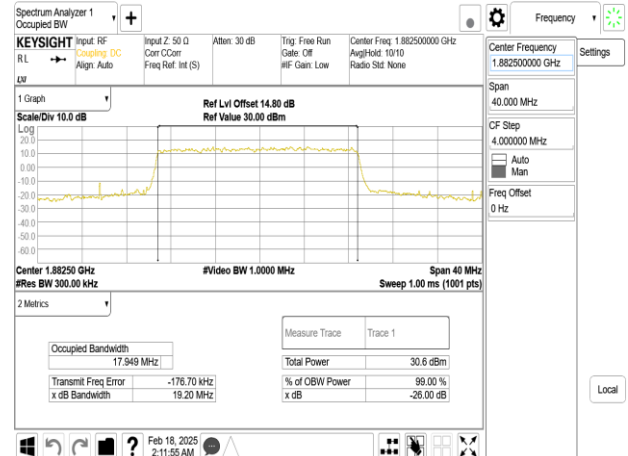
Band25_20MHz_DFT_s_OFDM_SCS30kHz_QPSK_RB50_0_CH376500
