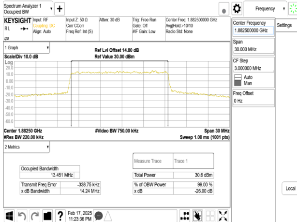
Band25_15MHz_DFT_s_OFDM_SCS15kHz_QPSK_RB75_0_CH376500
