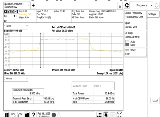
Band25_15MHz_DFT_s_OFDM_SCS30kHz_QPSK_RB36_0_CH376500
