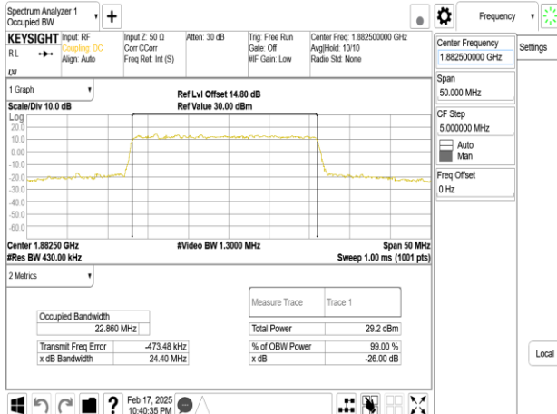
Band25_25MHz_DFT_s_OFDM_SCS15kHz_64QAM_RB128_0_CH376500
