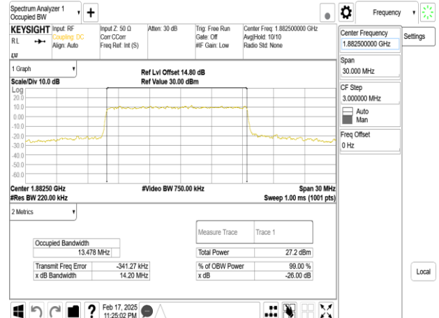
Band25_15MHz_DFT_s_OFDM_SCS15kHz_256QAM_RB75_0_CH376500
