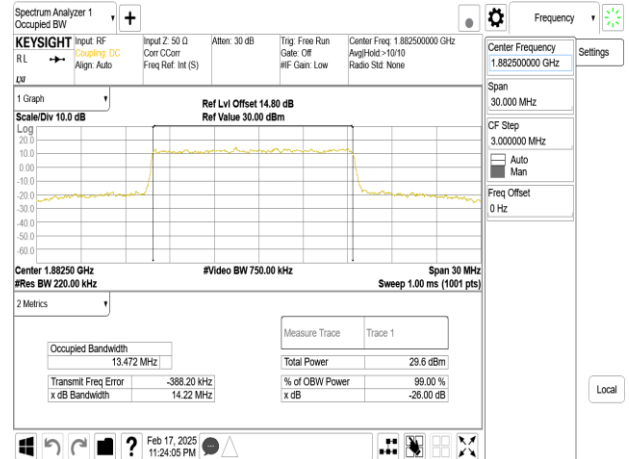
Band25_15MHz_DFT_s_OFDM_SCS15kHz_16QAM_RB75_0_CH376500
