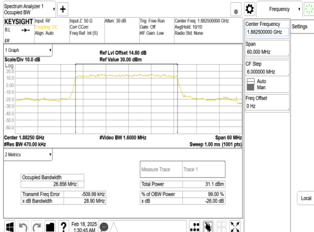
Band25_30MHz_DFT_s_OFDM_SCS30kHz_BPSK_RB75_0_CH376500
