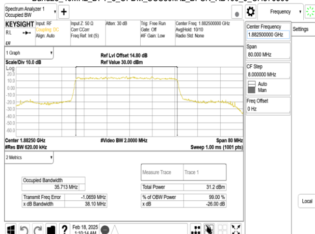
Band25_40MHz_DFT_s_OFDM_SCS30kHz_BPSK_RB100_0_CH376500
