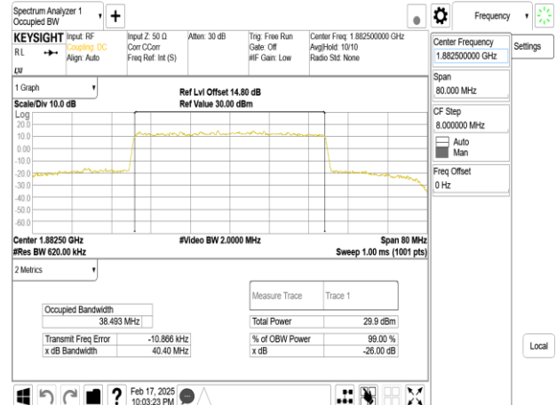
Band25_40MHz_DFT_s_OFDM_SCS15kHz_16QAM_RB216_0_CH376500
