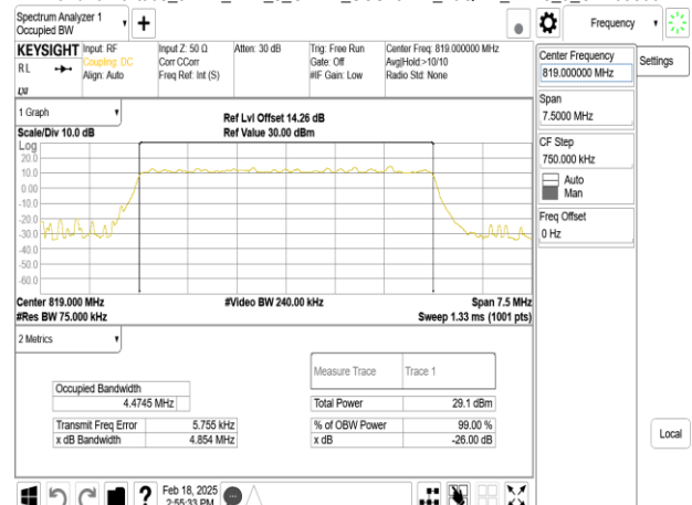
Band26-Part90s_5MHz_DFT_s_OFDM_SCS15kHz_16QAM_RB25_0_CH163800
