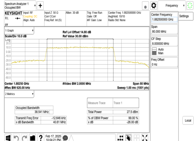
Band25_40MHz_DFT_s_OFDM_SCS15kHz_256QAM_RB216_0_CH376500
