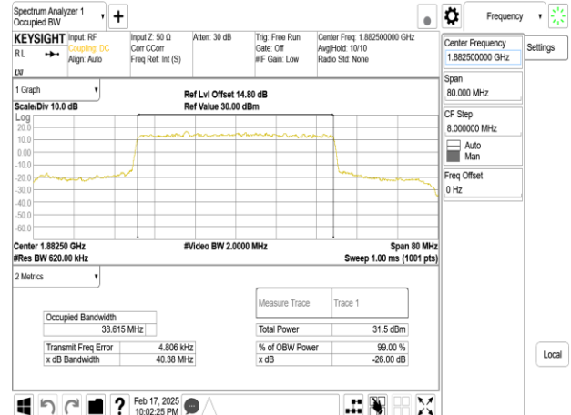
Band25_40MHz_DFT_s_OFDM_SCS15kHz_BPSK_RB216_0_CH376500
