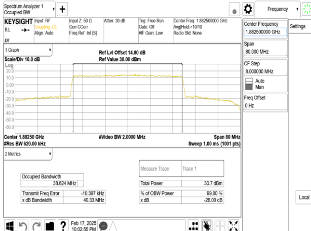
Band25_40MHz_DFT_s_OFDM_SCS15kHz_QPSK_RB216_0_CH376500
