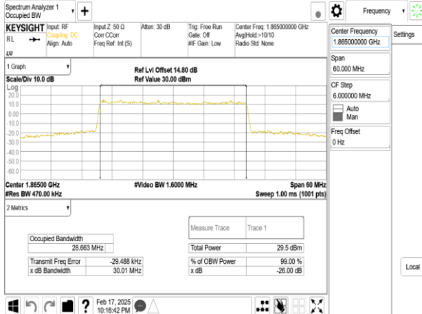
Band25_30MHz_DFT_s_OFDM_SCS15kHz_64QAM_RB160_0_CH376500
