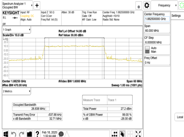
Band25_30MHz_DFT_s_OFDM_SCS30kHz_256QAM_RB75_0_CH376500
