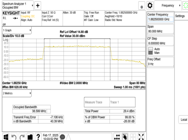
Band25_40MHz_DFT_s_OFDM_SCS15kHz_64QAM_RB216_0_CH376500
