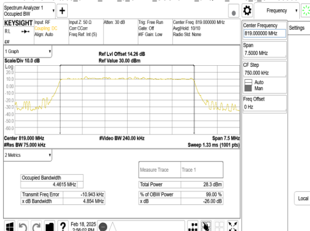
Band26-Part90s_5MHz_DFT_s_OFDM_SCS15kHz_64QAM_RB25_0_CH163800
