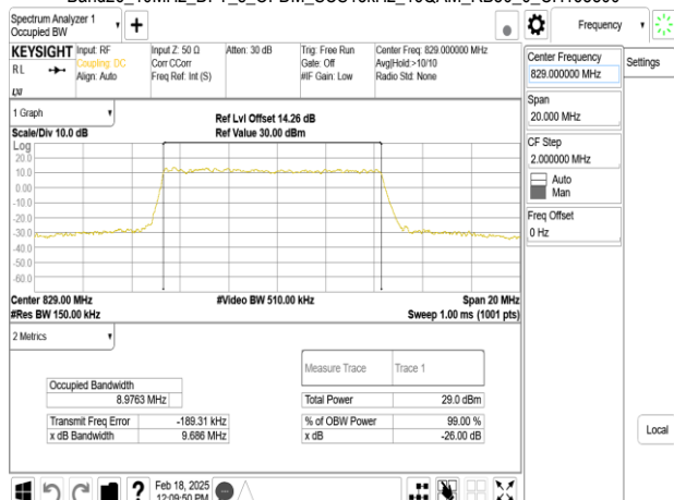
Band26_10MHz_DFT_s_OFDM_SCS15kHz_16QAM_RB50_0_CH165800
