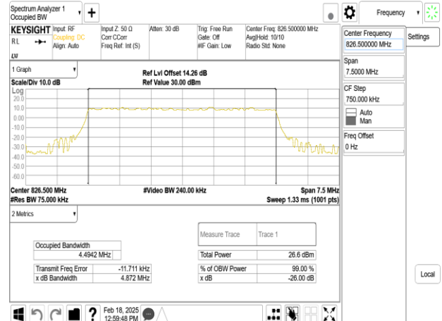
Band26_5MHz_DFT_s_OFDM_SCS15kHz_256QAM_RB25_0_CH165300
