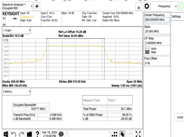
Band26_10MHz_DFT_s_OFDM_SCS30kHz_QPSK_RB24_0_CH165800
