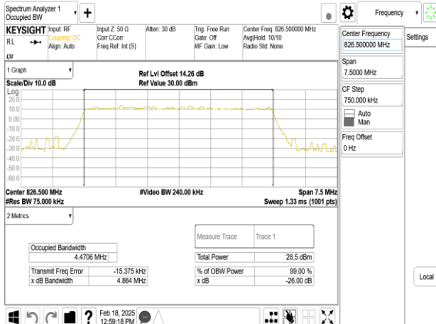
Band26_5MHz_DFT_s_OFDM_SCS15kHz_64QAM_RB25_0_CH165300
