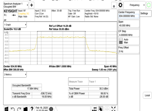
Band26_20MHz_DFT_s_OFDM_SCS15kHz_QPSK_RB100_0_CH166800
