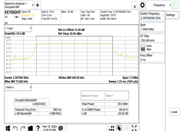
Band30_5MHz_DFT_s_OFDM_SCS15kHz_QPSK_RB25_0_CH461500
