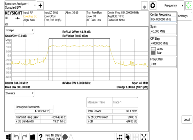
Band26_20MHz_DFT_s_OFDM_SCS30kHz_BPSK_RB50_0_CH166800
