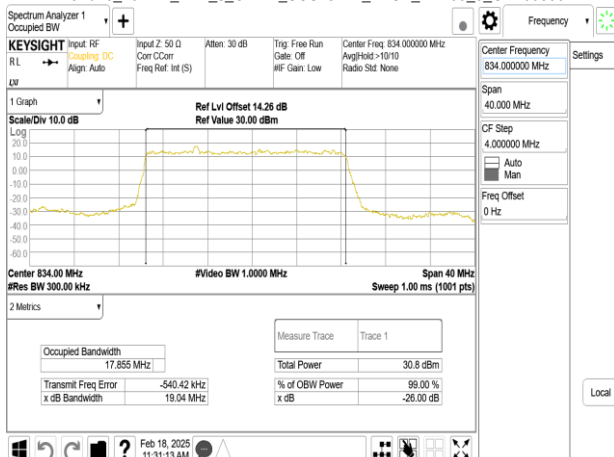
Band26_20MHz_DFT_s_OFDM_SCS15kHz_BPSK_RB100_0_CH166800
