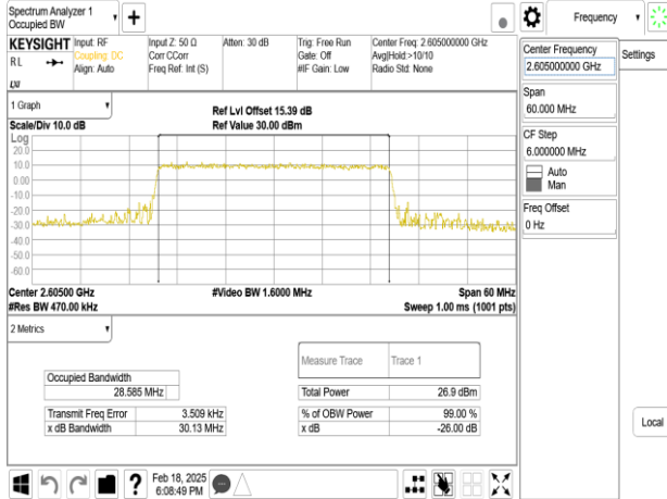
Band38_30MHz_DFT_s_OFDM_SCS30kHz_BPSK_RB75_0_CH517000
