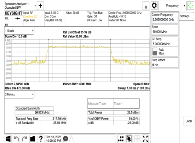
Band38_30MHz_DFT_s_OFDM_SCS30kHz_64QAM_RB75_0_CH517000
