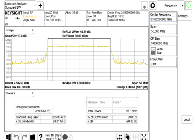
Band38_25MHz_DFT_s_OFDM_SCS30kHz_64QAM_RB64_0_CH516500
