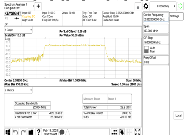
Band38_25MHz_DFT_s_OFDM_SCS15kHz_QPSK_RB128_0_CH516500
