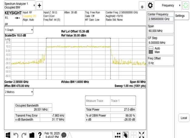
Band38_30MHz_DFT_s_OFDM_SCS15kHz_256QAM_RB160_0_CH517000
