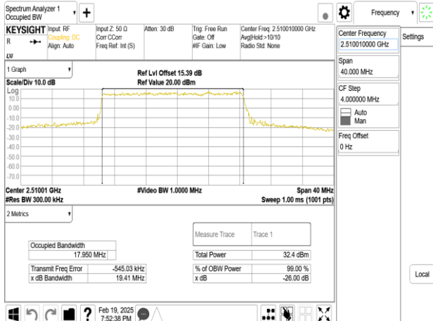
Band41_20MHz_DFT_s_OFDM_SCS15kHz_16QAM_RB100_0_CH502002
