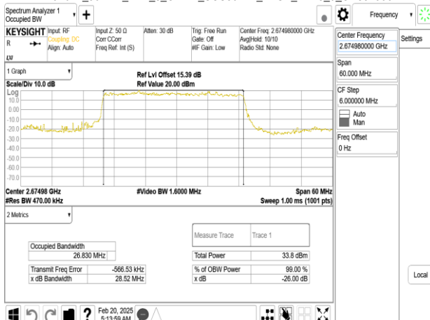
Band41_30MHz_DFT_s_OFDM_SCS30kHz_BPSK_RB75_0_CH534996
