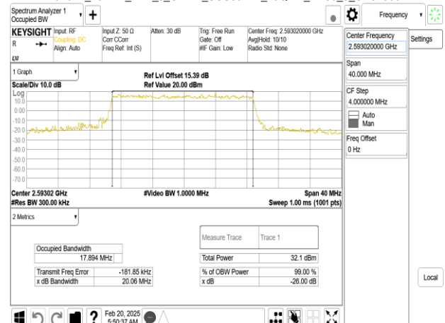
Band41_20MHz_DFT_s_OFDM_SCS30kHz_16QAM_RB50_0_CH518604
