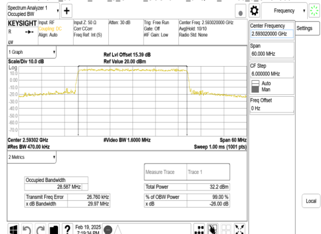
Band41_30MHz_DFT_s_OFDM_SCS15kHz_64QAM_RB160_0_CH518604
