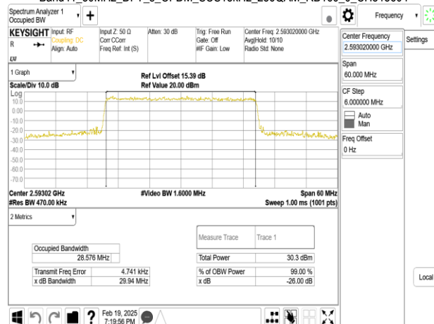
Band41_30MHz_DFT_s_OFDM_SCS15kHz_256QAM_RB160_0_CH534996
