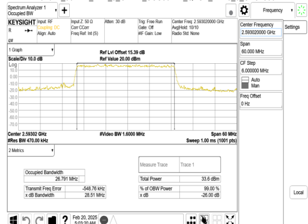
Band41_30MHz_DFT_s_OFDM_SCS30kHz_QPSK_RB75_0_CH518604
