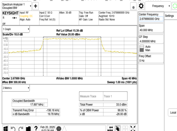
Band41_20MHz_DFT_s_OFDM_SCS30kHz_QPSK_RB50_0_CH535998
