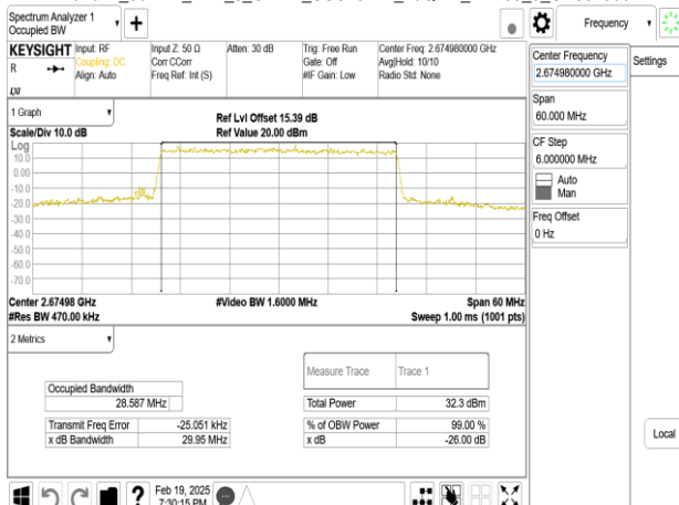
Band41_30MHz_DFT_s_OFDM_SCS15kHz_16QAM_RB160_0_CH534996
