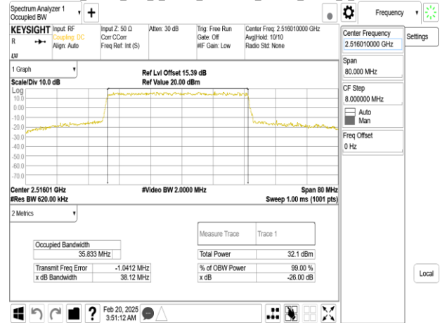
Band41_40MHz_DFT_s_OFDM_SCS30kHz_64QAM_RB100_0_CH504000
