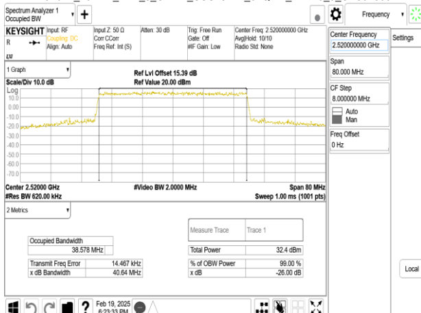
Band41_40MHz_DFT_s_OFDM_SCS15kHz_64QAM_RB216_0_CH504000
