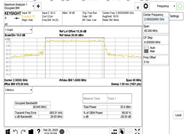
Band41_30MHz_DFT_s_OFDM_SCS30kHz_256QAM_RB75_0_CH518604
