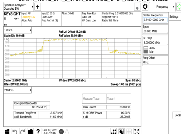
Band41_40MHz_DFT_s_OFDM_SCS15kHz_QPSK_RB216_0_CH503202
