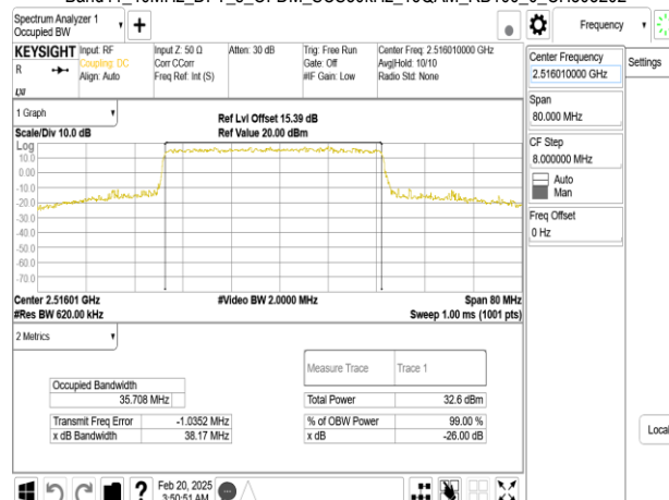
Band41_40MHz_DFT_s_OFDM_SCS30kHz_16QAM_RB100_0_CH503202
