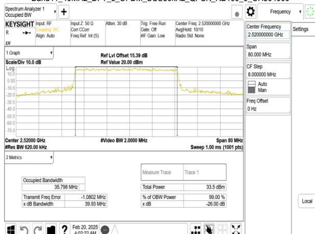
Band41_40MHz_DFT_s_OFDM_SCS30kHz_QPSK_RB100_0_CH504000
