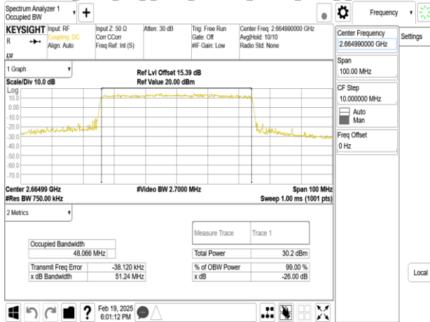
Band41_50MHz_DFT_s_OFDM_SCS30kHz_BPSK_RB128_0_CH504204
