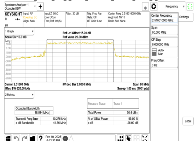
Band41_40MHz_DFT_s_OFDM_SCS15kHz_256QAM_RB216_0_CH503202
