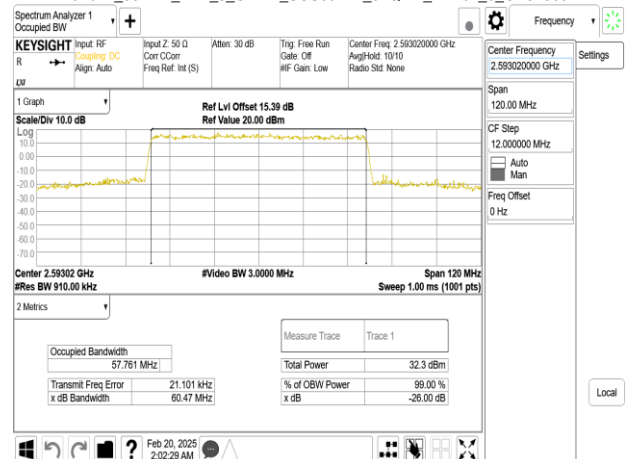
Band41_60MHz_DFT_s_OFDM_SCS30kHz_64QAM_RB162_0_CH518604
