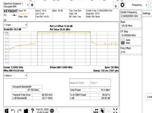
Band41_60MHz_DFT_s_OFDM_SCS30kHz_BPSK_RB162_0_CH518604
