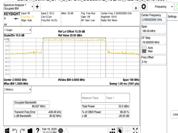
Band41_90MHz_DFT_s_OFDM_SCS30kHz_16QAM_RB243_0_CH518604
