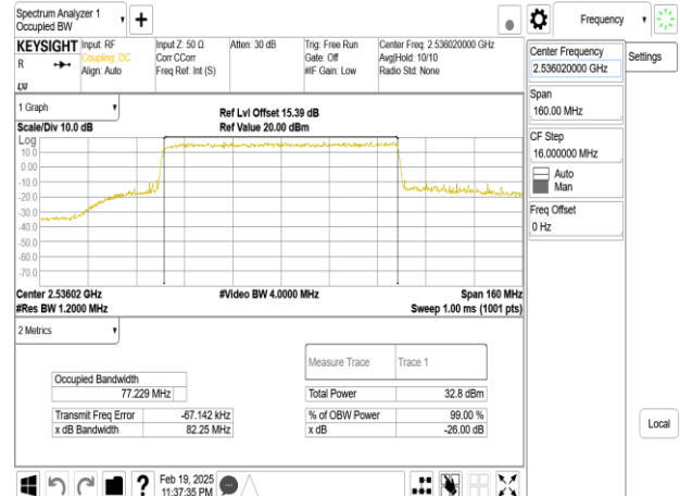
Band41_80MHz_DFT_s_OFDM_SCS30kHz_64QAM_RB216_0_CH507204
