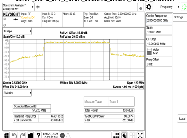
Band41_60MHz_DFT_s_OFDM_SCS30kHz_256QAM_RB162_0_CH506004
