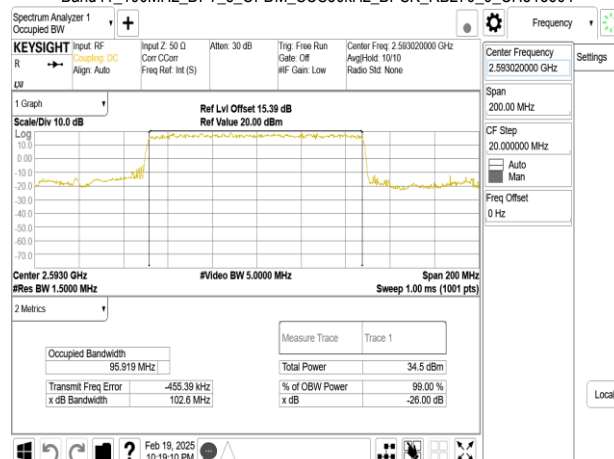
Band41_100MHz_DFT_s_OFDM_SCS30kHz_BPSK_RB270_0_CH518604
