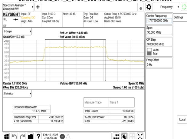
Band66_15MHz_DFT_s_OFDM_SCS15kHz_16QAM_RB75_0_CH343500
