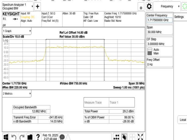
Band66_15MHz_DFT_s_OFDM_SCS30kHz_64QAM_RB36_0_CH343500
