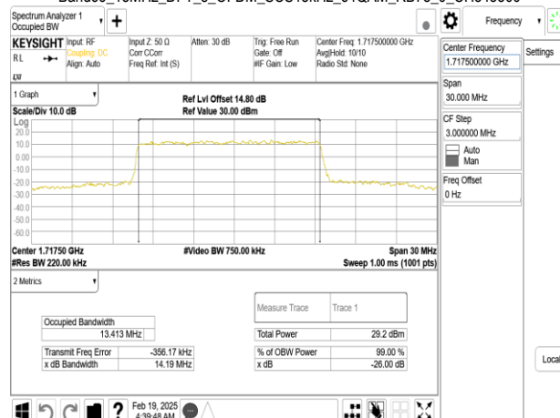
Band66_15MHz_DFT_s_OFDM_SCS15kHz_64QAM_RB75_0_CH343500
