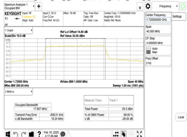
Band66_20MHz_DFT_s_OFDM_SCS15kHz_64QAM_RB100_0_CH344000
