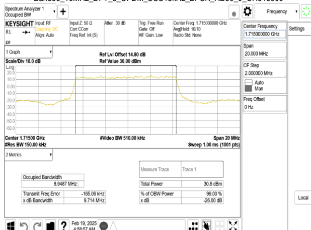
Band66_10MHz_DFT_s_OFDM_SCS15kHz_BPSK_RB50_0_CH343000
