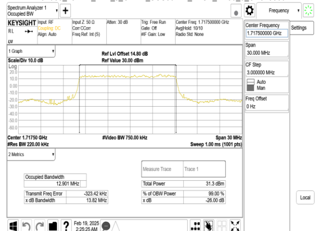
Band66_15MHz_DFT_s_OFDM_SCS30kHz_BPSK_RB36_0_CH343500
