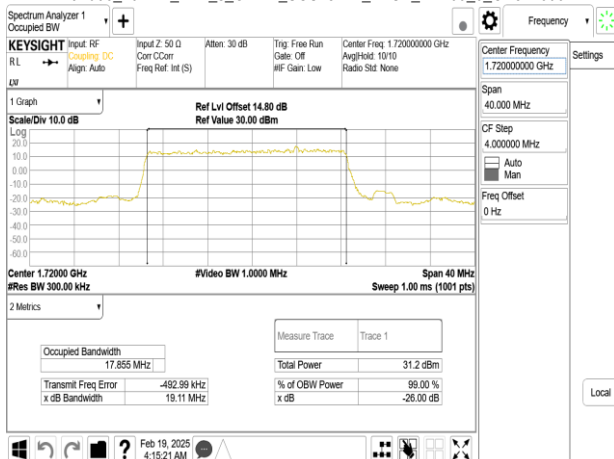
Band66_20MHz_DFT_s_OFDM_SCS15kHz_BPSK_RB100_0_CH344000
