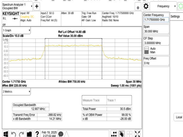
Band66_15MHz_DFT_s_OFDM_SCS30kHz_QPSK_RB36_0_CH343500
