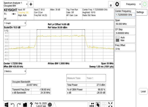
Band66_25MHz_DFT_s_OFDM_SCS30kHz_256QAM_RB64_0_CH344500
