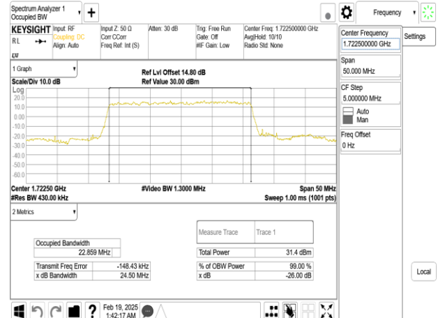
Band66_25MHz_DFT_s_OFDM_SCS30kHz_BPSK_RB64_0_CH344500
