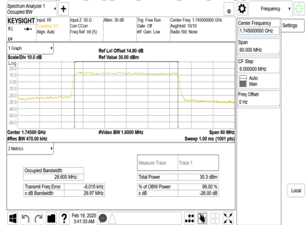
Band66_30MHz_DFT_s_OFDM_SCS15kHz_16QAM_RB160_0_CH353000
