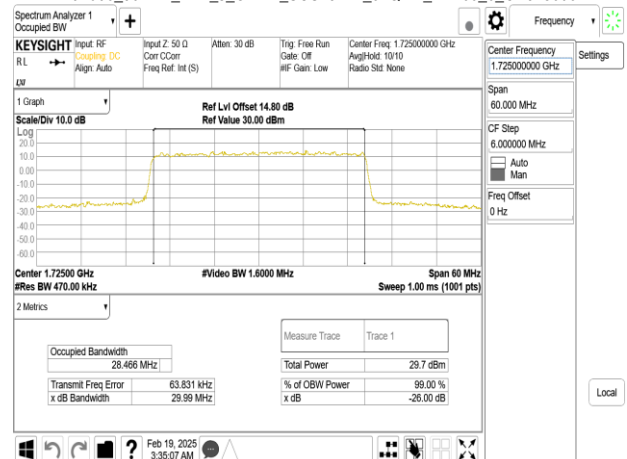
Band66_30MHz_DFT_s_OFDM_SCS15kHz_64QAM_RB160_0_CH345000
