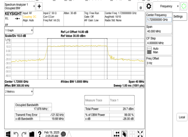
Band66_20MHz_DFT_s_OFDM_SCS30kHz_16QAM_RB50_0_CH344000
