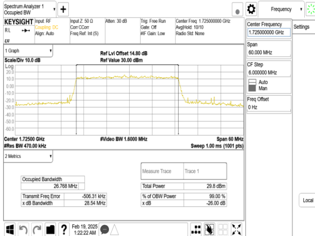
Band66_30MHz_DFT_s_OFDM_SCS30kHz_64QAM_RB75_0_CH345000
