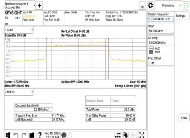
Band66_25MHz_DFT_s_OFDM_SCS15kHz_64QAM_RB128_0_CH344500
