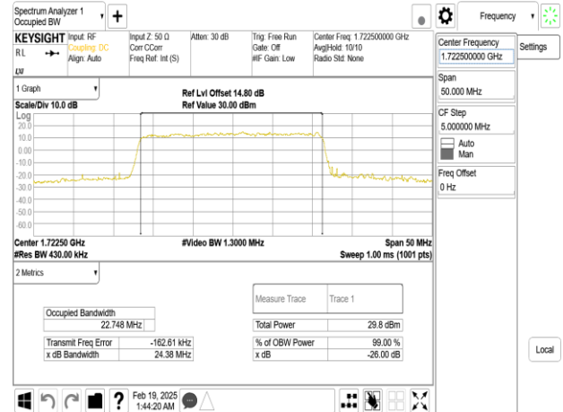
Band66_25MHz_DFT_s_OFDM_SCS30kHz_16QAM_RB64_0_CH344500
