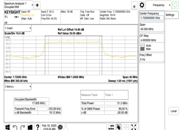
Band66_20MHz_DFT_s_OFDM_SCS30kHz_BPSK_RB50_0_CH344000
