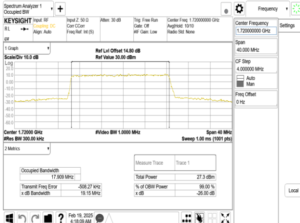
Band66_20MHz_DFT_s_OFDM_SCS15kHz_256QAM_RB100_0_CH344000
