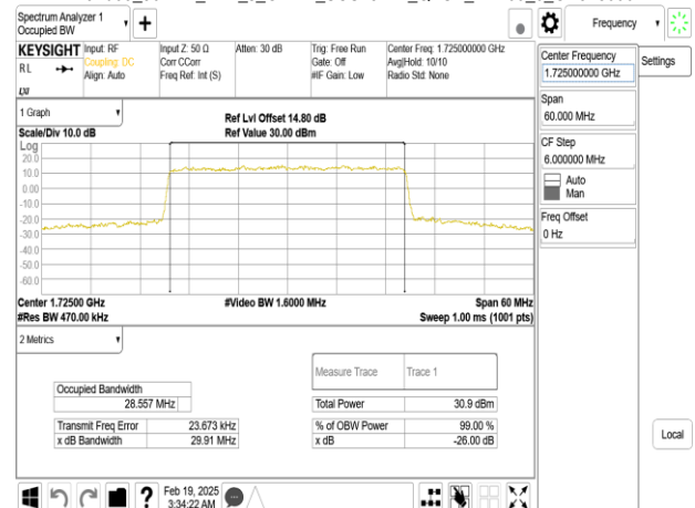
Band66_30MHz_DFT_s_OFDM_SCS15kHz_QPSK_RB160_0_CH345000
