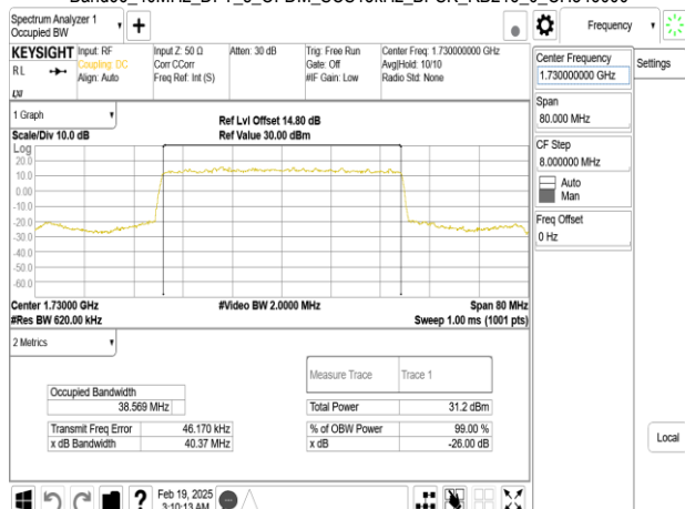
Band66_40MHz_DFT_s_OFDM_SCS15kHz_BPSK_RB216_0_CH346000
