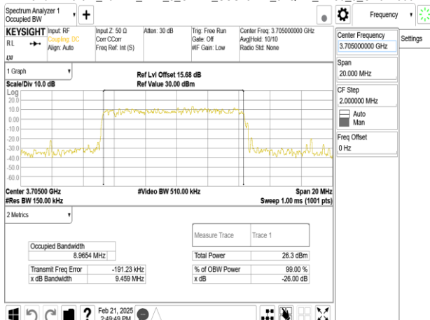
Band77-Part27_10MHz_DFT_s_OFDM_SCS15kHz_64QAM_RB50_0_CH647000
