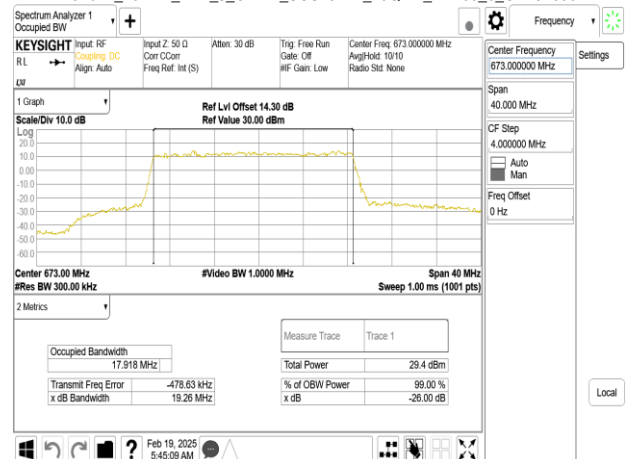
Band71_20MHz_DFT_s_OFDM_SCS15kHz_16QAM_RB100_0_CH134600
