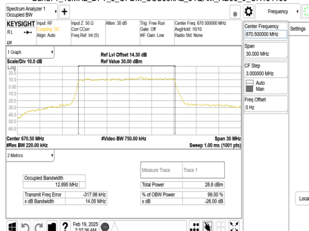
Band71_15MHz_DFT_s_OFDM_SCS30kHz_64QAM_RB36_0_CH134100
