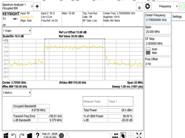
Band77-Part27_10MHz_DFT_s_OFDM_SCS15kHz_QPSK_RB50_0_CH647000
