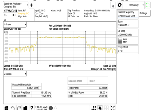
Band77-Part27_10MHz_DFT_s_OFDM_SCS15kHz_256QAM_RB50_0_CH630334
