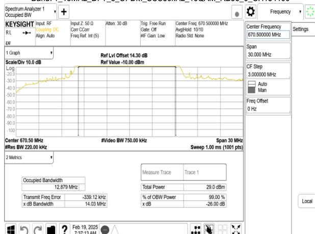
Band71_15MHz_DFT_s_OFDM_SCS30kHz_16QAM_RB36_0_CH134100
