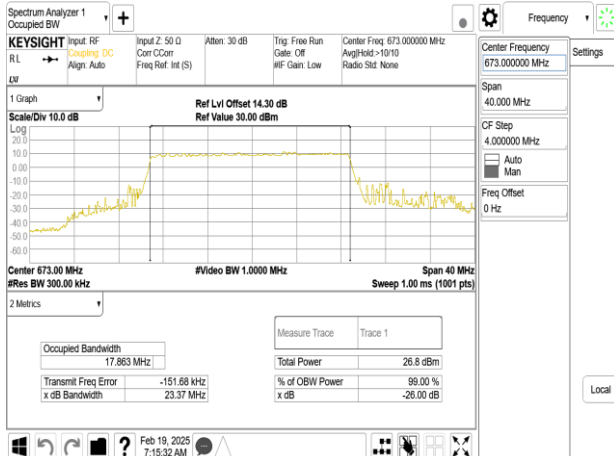
Band71_20MHz_DFT_s_OFDM_SCS30kHz_256QAM_RB50_0_CH134600
