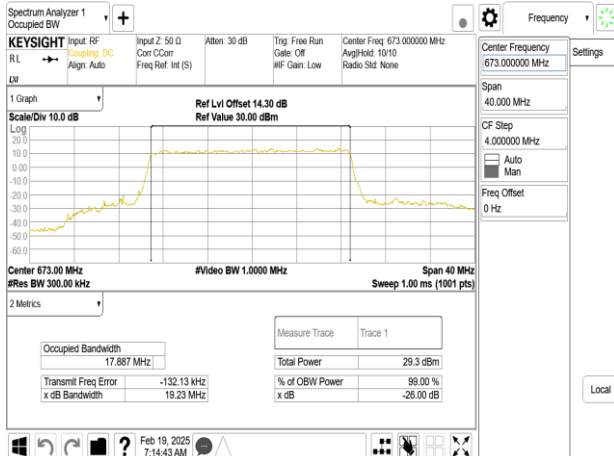
Band71_20MHz_DFT_s_OFDM_SCS30kHz_16QAM_RB50_0_CH134600
