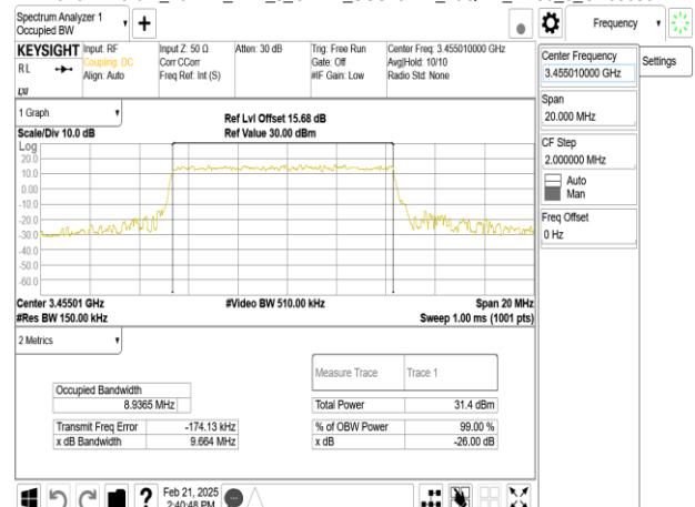
Band77-Part27_10MHz_DFT_s_OFDM_SCS15kHz_16QAM_RB50_0_CH630334
