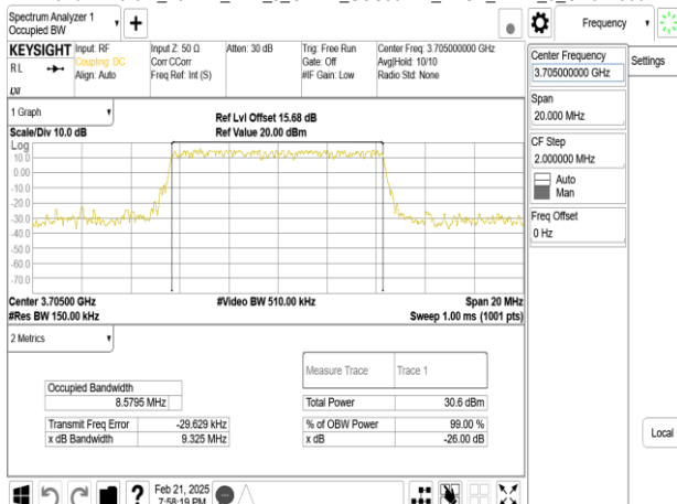
Band77-Part27_10MHz_DFT_s_OFDM_SCS30kHz_BPSK_RB24_0_CH647000
