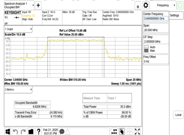
Band77-Part27_10MHz_DFT_s_OFDM_SCS30kHz_BPSK_RB24_0_CH656000
