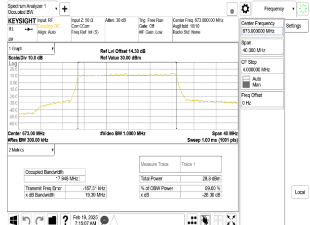
Band71_20MHz_DFT_s_OFDM_SCS30kHz_64QAM_RB50_0_CH134600
