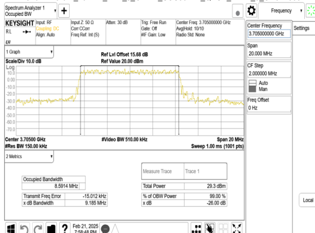
Band77-Part27_10MHz_DFT_s_OFDM_SCS30kHz_QPSK_RB24_0_CH647000
