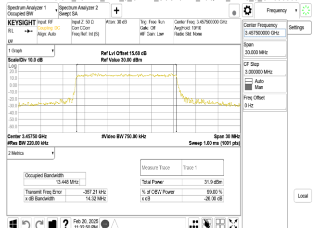
Band77-Part27_15MHz_DFT_s_OFDM_SCS15kHz_16QAM_RB75_0_CH630500
