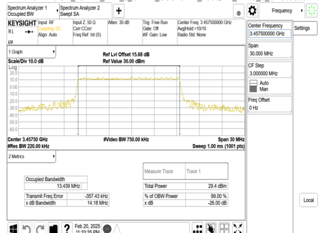
Band77-Part27_15MHz_DFT_s_OFDM_SCS15kHz_256QAM_RB75_0_CH630500
