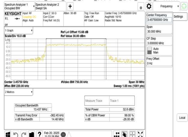
Band77-Part27_15MHz_DFT_s_OFDM_SCS15kHz_QPSK_RB75_0_CH630500
