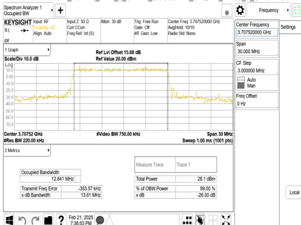
Band77-Part27_15MHz_DFT_s_OFDM_SCS30kHz_64QAM_RB36_0_CH647168
