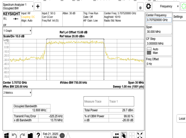
Band77-Part27_15MHz_DFT_s_OFDM_SCS30kHz_QPSK_RB36_0_CH647168
