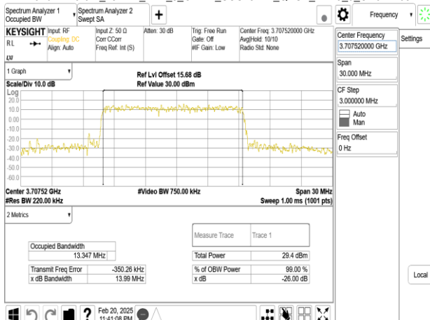
Band77-Part27_15MHz_DFT_s_OFDM_SCS15kHz_QPSK_RB75_0_CH647168
