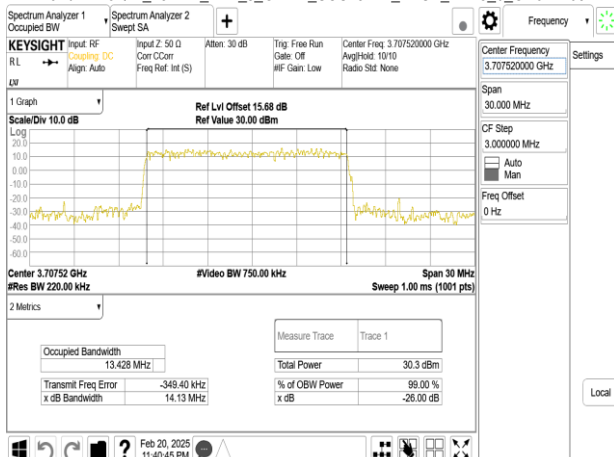
Band77-Part27_15MHz_DFT_s_OFDM_SCS15kHz_BPSK_RB75_0_CH647168
