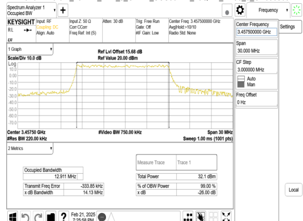
Band77-Part27_15MHz_DFT_s_OFDM_SCS30kHz_16QAM_RB36_0_CH630500
