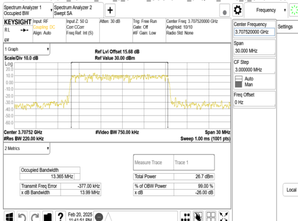
Band77-Part27_15MHz_DFT_s_OFDM_SCS15kHz_64QAM_RB75_0_CH647168
