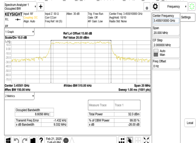
Band77-Part27_10MHz_DFT_s_OFDM_SCS30kHz_16QAM_RB24_0_CH630334
