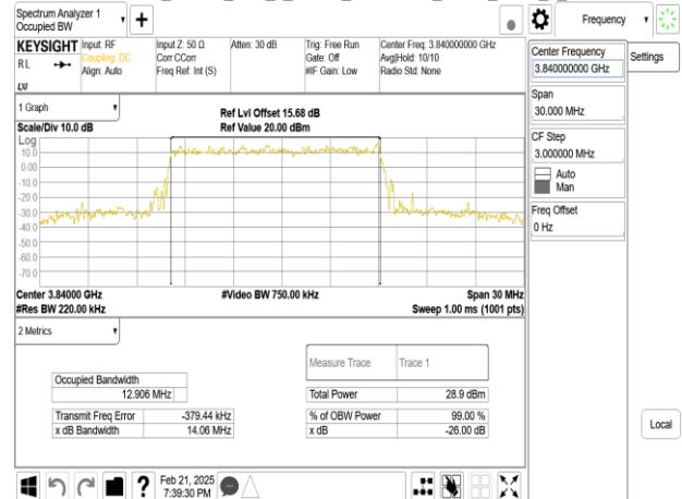
Band77-Part27_15MHz_DFT_s_OFDM_SCS30kHz_QPSK_RB36_0_CH64832
