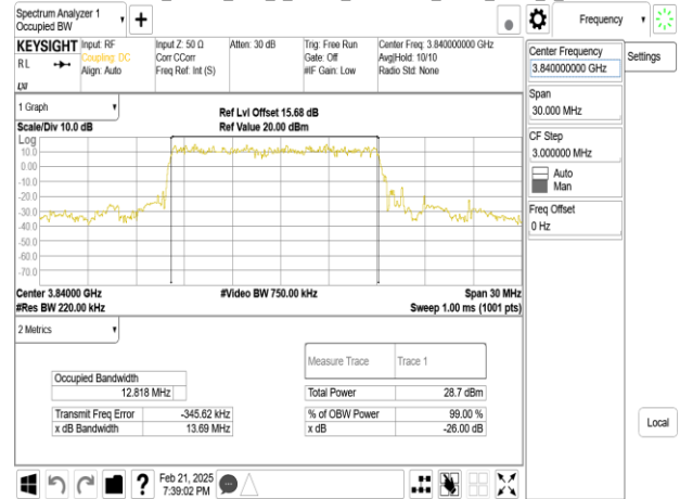
Band77-Part27_15MHz_DFT_s_OFDM_SCS30kHz_BPSK_RB36_0_CH64832
