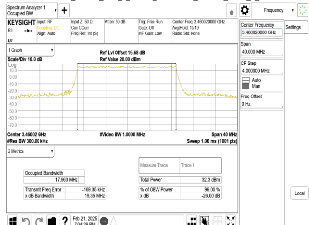
Band77-Part27_20MHz_DFT_s_OFDM_SCS30kHz_16QAM_RB50_0_CH630668
