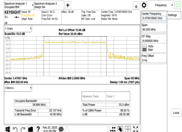
Band77-Part27_40MHz_DFT_s_OFDM_SCS15kHz_QPSK_RB216_0_CH631334
