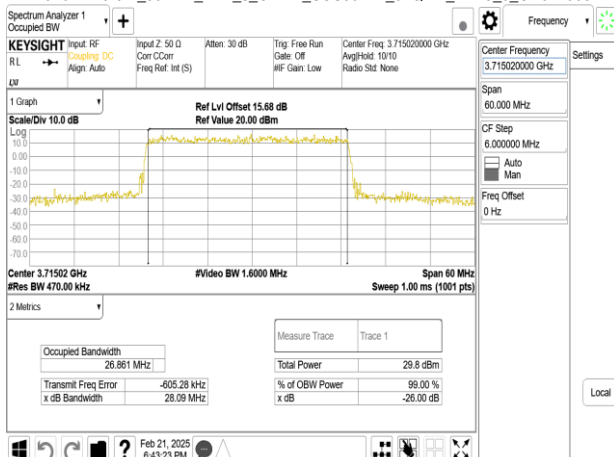
Band77-Part27_30MHz_DFT_s_OFDM_SCS30kHz_64QAM_RB75_0_CH647668
