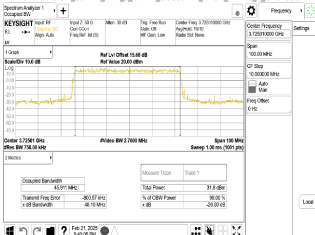
Band77-Part27_50MHz_DFT_s_OFDM_SCS30kHz_BPSK_RB128_0_CH648334
