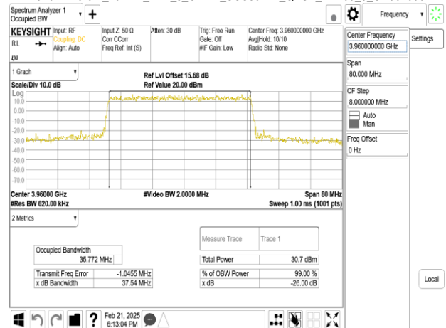
Band77-Part27_40MHz_DFT_s_OFDM_SCS30kHz_16QAM_RB100_0_CH631334
