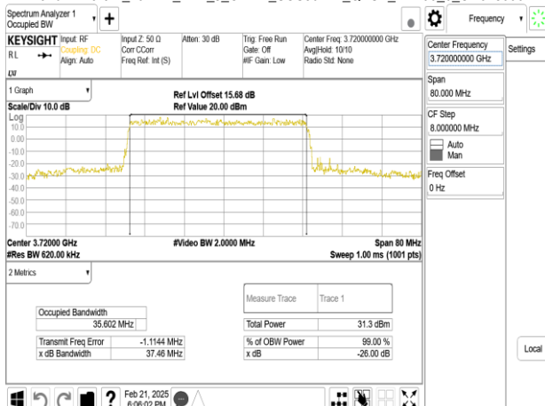
Band77-Part27_40MHz_DFT_s_OFDM_SCS30kHz_QPSK_RB100_0_CH648000
