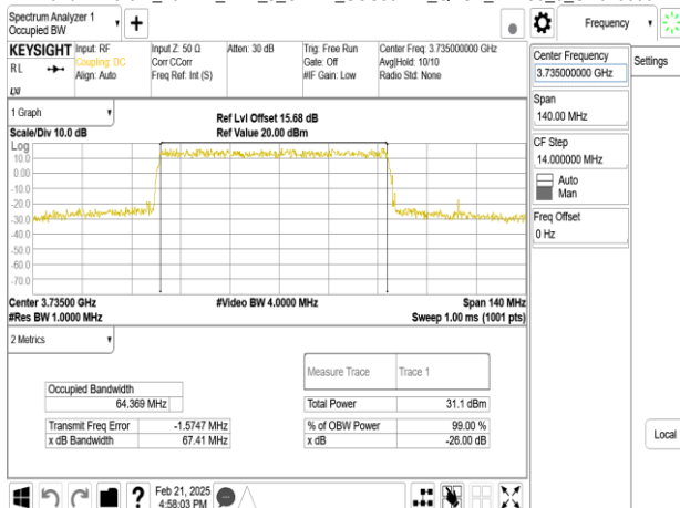
Band77-Part27_70MHz_DFT_s_OFDM_SCS30kHz_QPSK_RB180_0_CH649000
