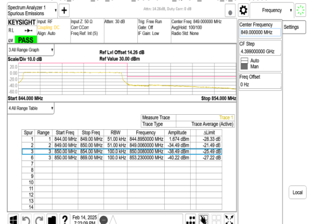
Band5_5MHz_CP_OFDM_SCS15kHz_QPSK_RB25_0_CH169300
