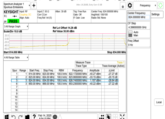
Band5_10MHz_CP_OFDM_SCS15kHz_QPSK_RB50_0_CH165800
