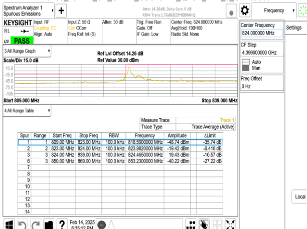
Band5_15MHz_CP_OFDM_SCS15kHz_QPSK_RB1_0_CH166300
