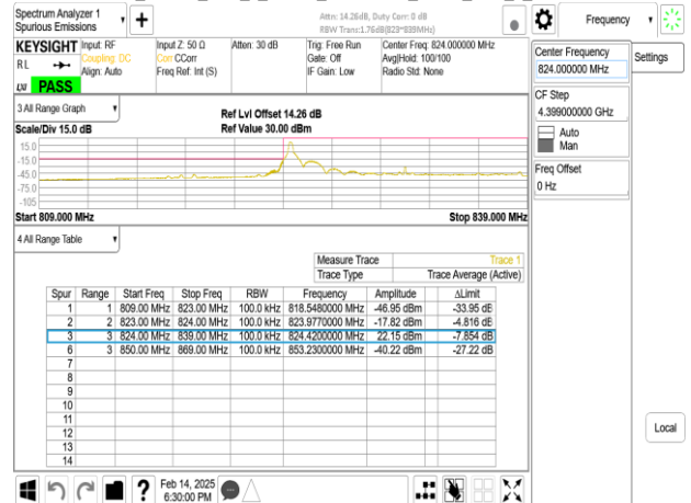
Band5_15MHz_DFT_s_OFDM_SCS15kHz_BPSK_RB75_0_CH166300
