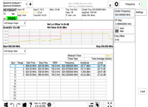
Band5_15MHz_DFT_s_OFDM_SCS15kHz_BPSK_RB75_0_CH166300
