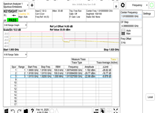
Band2_10MHz_CP_OFDM_SCS15kHz_QPSK_RB52_0_CH381000
