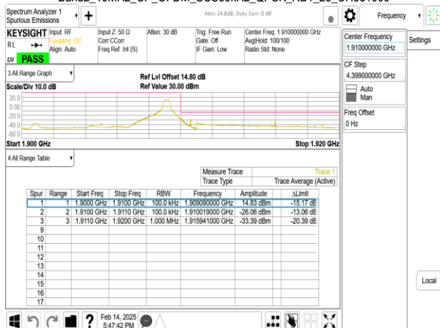
Band2_10MHz_CP_OFDM_SCS30kHz_QPSK_RB24_0_CH381000
