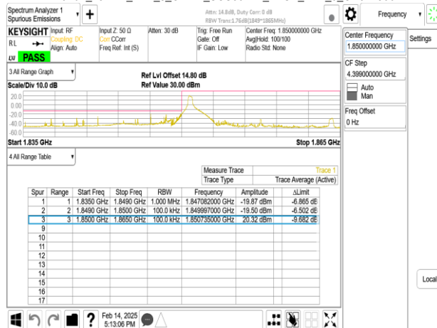
Band2_15MHz_DFT_s_OFDM_SCS30kHz_BPSK_RB36_0_CH371500
