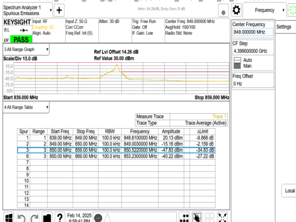
Band5_10MHz_DFT_s_OFDM_SCS15kHz_BPSK_RB1_51_CH168800
