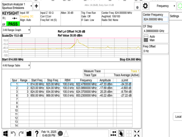
Band5_10MHz_DFT_s_OFDM_SCS15kHz_BPSK_RB50_0_CH165800
