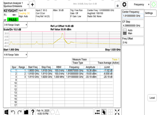
Band2_10MHz_CP_OFDM_SCS15kHz_QPSK_RB52_0_CH381000
