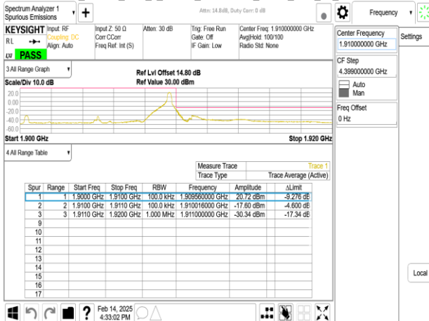
Band2_10MHz_DFT_s_OFDM_SCS15kHz_BPSK_RB50_0_CH381000
