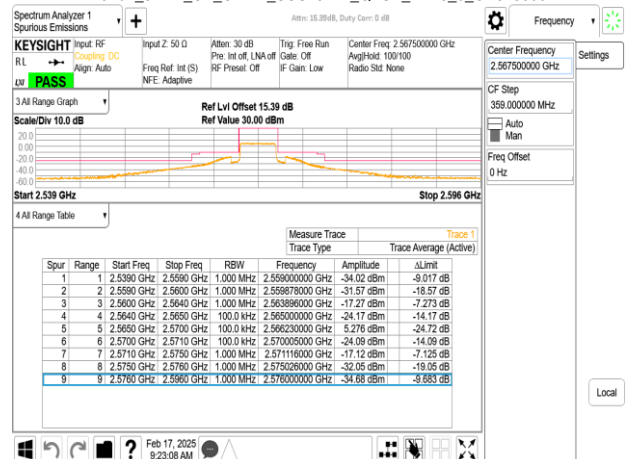
Band7_5MHz_CP_OFDM_SCS15kHz_QPSK_RB25_0_CH513500
