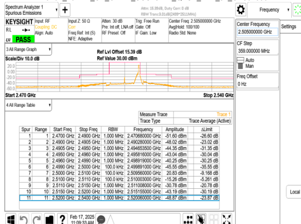
Band7_10MHz_CP_OFDM_SCS15kHz_QPSK_RB52_0_CH501000
