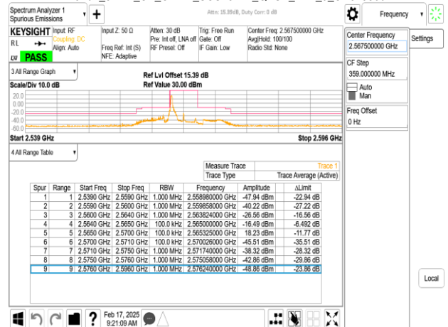
Band7_5MHz_CP_OFDM_SCS15kHz_QPSK_RB1_24_CH513500
