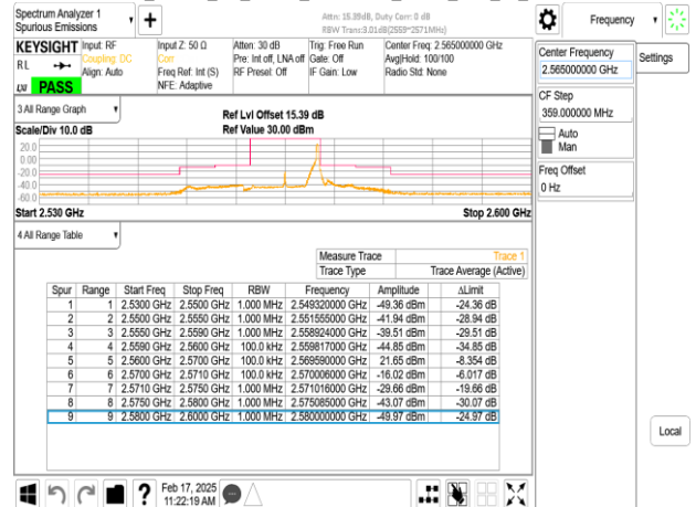
Band7_10MHz_CP_OFDM_SCS15kHz_QPSK_RB52_0_CH513000
