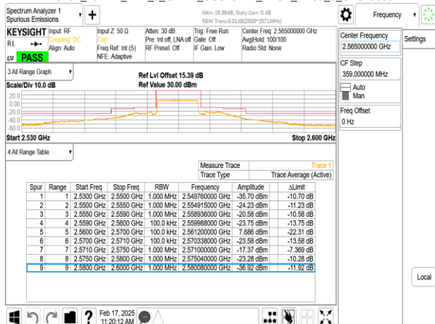
Band7_10MHz_DFT_s_OFDM_SCS15kHz_BPSK_RB50_0_CH513000
