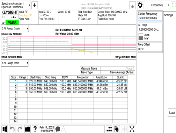
Band5_20MHz_CP_OFDM_SCS30kHz_QPSK_RB1_0_CH166800
