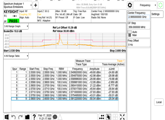
Band7_10MHz_CP_OFDM_SCS15kHz_QPSK_RB1_51_CH513000
