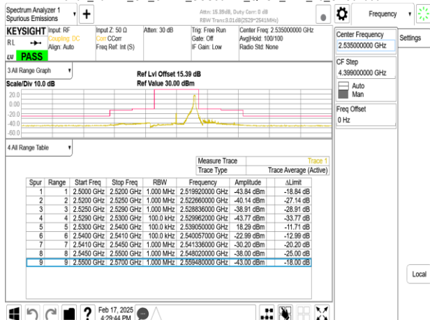
Band7_10MHz_CP_OFDM_SCS30kHz_QPSK_RB24_0_CH507000
