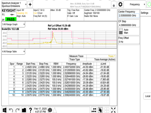
Band7_15MHz_CP_OFDM_SCS30kHz_QPSK_RB1_37_CH507000
