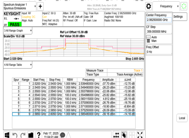
Band7_15MHz_CP_OFDM_SCS15kHz_QPSK_RB79_0_CH512500
