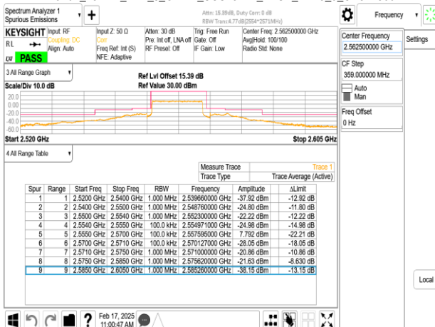
Band7_15MHz_DFT_s_OFDM_SCS15kHz_BPSK_RB75_0_CH512500
