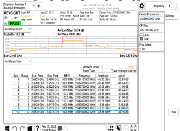
Band7_15MHz_DFT_s_OFDM_SCS15kHz_BPSK_RB75_0_CH507000
