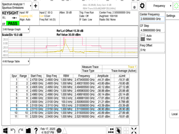
Band7_10MHz_DFT_s_OFDM_SCS30kHz_BPSK_RB1_23_CH501000
