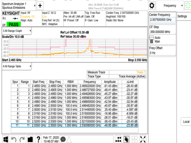
Band7_15MHz_DFT_s_OFDM_SCS15kHz_BPSK_RB75_0_CH501500
