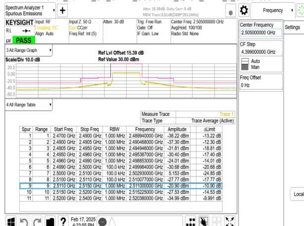
Band7_10MHz_CP_OFDM_SCS30kHz_QPSK_RB24_0_CH501000
