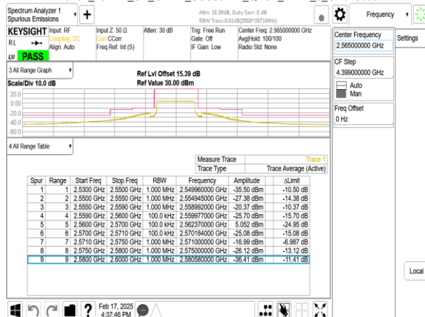
Band7_10MHz_CP_OFDM_SCS30kHz_QPSK_RB24_0_CH513000
