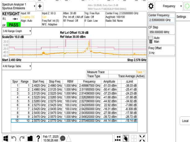
Band7_15MHz_CP_OFDM_SCS15kHz_QPSK_RB79_0_CH507000
