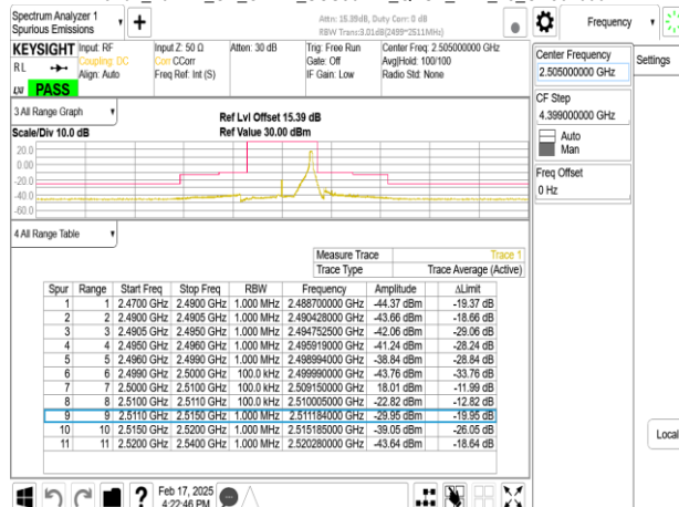
Band7_10MHz_CP_OFDM_SCS30kHz_QPSK_RB24_0_CH501000
