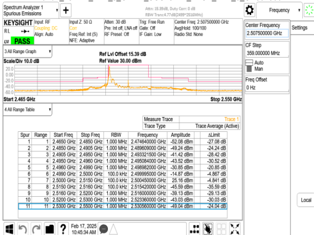
Band7_15MHz_DFT_s_OFDM_SCS15kHz_BPSK_RB1_78_CH501500
