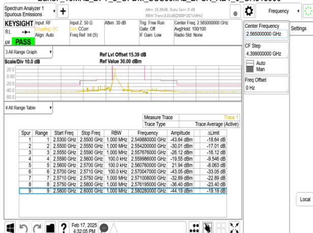
Band7_10MHz_DFT_s_OFDM_SCS30kHz_BPSK_RB1_23_CH513000
