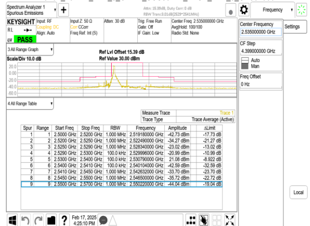
Band7_10MHz_DFT_s_OFDM_SCS30kHz_BPSK_RB1_23_CH507000
