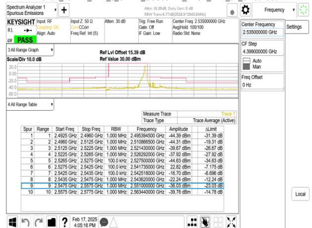
Band7_15MHz_DFT_s_OFDM_SCS30kHz_BPSK_RB36_0_CH507000
