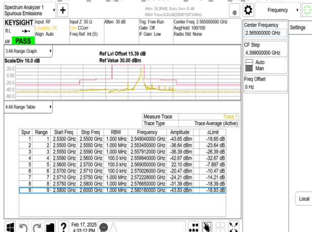
Band7_10MHz_DFT_s_OFDM_SCS30kHz_BPSK_RB24_0_CH513000
