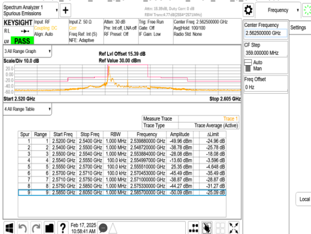
Band7_15MHz_DFT_s_OFDM_SCS15kHz_BPSK_RB1_78_CH512500
