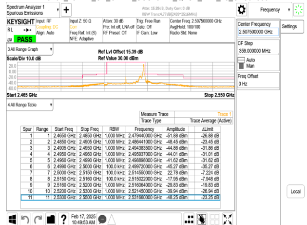
Band7_15MHz_CP_OFDM_SCS15kHz_QPSK_RB79_0_CH501500
