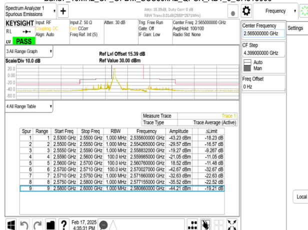
Band7_10MHz_CP_OFDM_SCS30kHz_QPSK_RB1_23_CH513000
