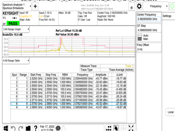
Band7_15MHz_DFT_s_OFDM_SCS30kHz_BPSK_RB1_37_CH512500
