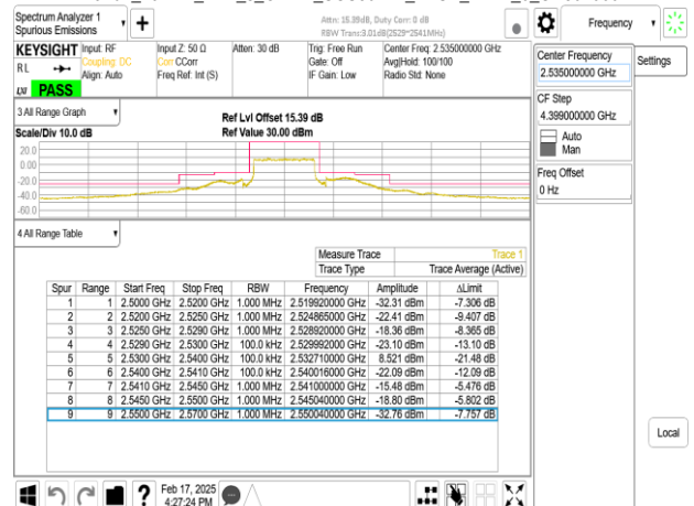
Band7_10MHz_DFT_s_OFDM_SCS30kHz_BPSK_RB24_0_CH507000
