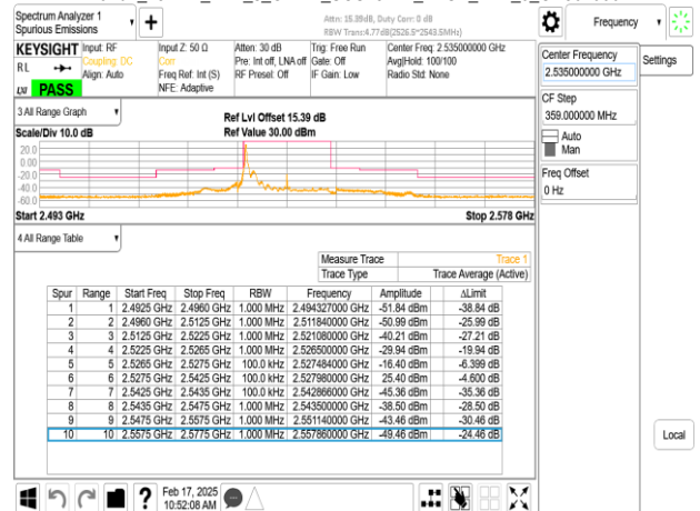
Band7_15MHz_DFT_s_OFDM_SCS15kHz_BPSK_RB1_78_CH507000
