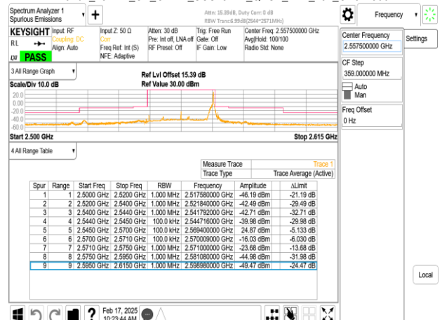
Band7_25MHz_CP_OFDM_SCS15kHz_QPSK_RB1_132_CH511500
