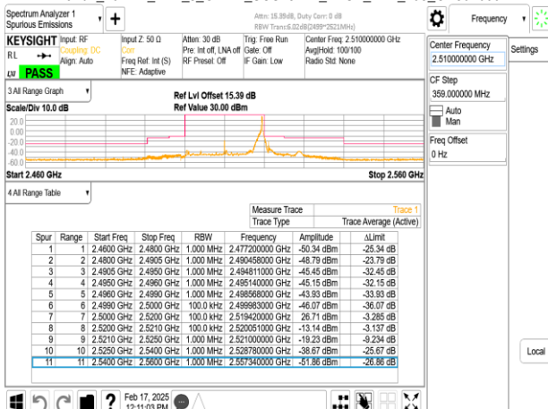
Band7_20MHz_DFT_s_OFDM_SCS15kHz_BPSK_RB1_105_CH502000
