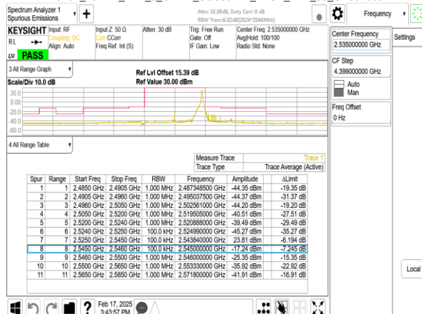
Band7_20MHz_DFT_s_OFDM_SCS30kHz_BPSK_RB50_0_CH507000
