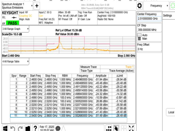
Band7_20MHz_DFT_s_OFDM_SCS15kHz_BPSK_RB1_105_CH502000
