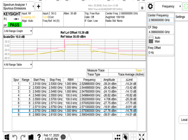
Band7_20MHz_CP_OFDM_SCS30kHz_QPSK_RB51_0_CH512000
