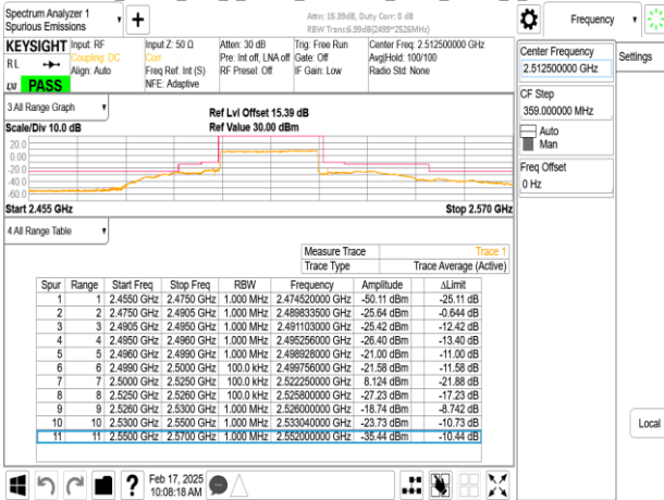
Band7_25MHz_DFT_s_OFDM_SCS15kHz_BPSK_RB1_0_CH502500
