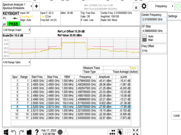
Band7_20MHz_DFT_s_OFDM_SCS30kHz_BPSK_RB50_0_CH502000
