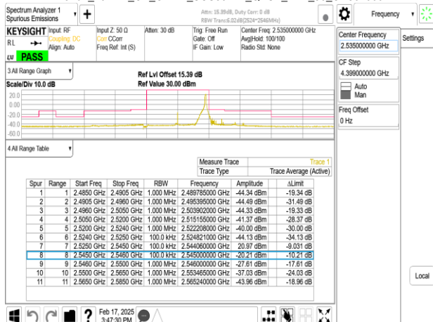
Band7_20MHz_CP_OFDM_SCS30kHz_QPSK_RB51_0_CH507000
