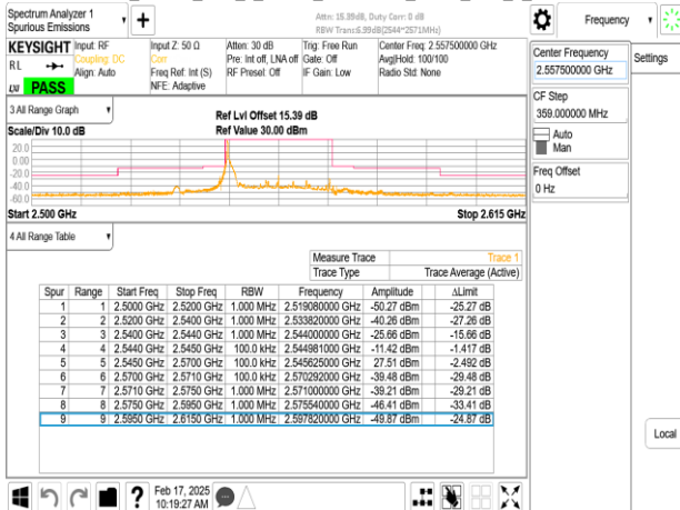
Band7_25MHz_DFT_s_OFDM_SCS15kHz_BPSK_RB1_132_CH511500
