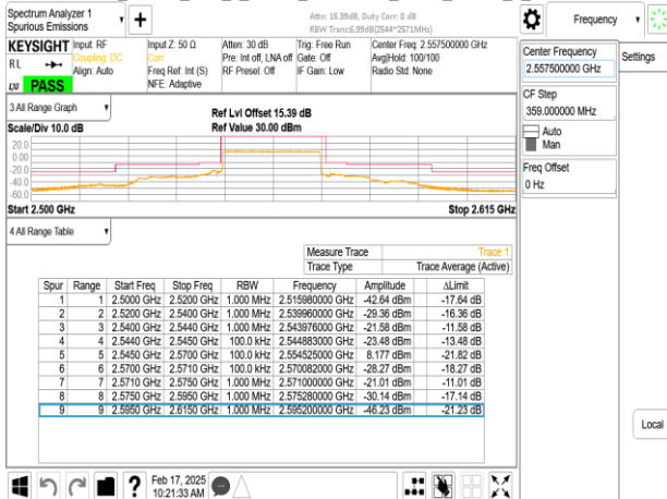
Band7_25MHz_DFT_s_OFDM_SCS15kHz_BPSK_RB1_0_CH511500
