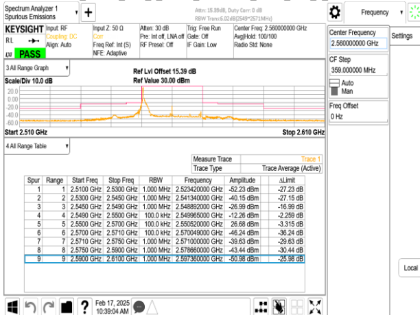
Band7_20MHz_DFT_s_OFDM_SCS15kHz_BPSK_RB1_105_CH512000
