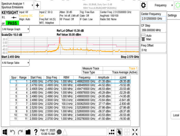
Band7_25MHz_DFT_s_OFDM_SCS15kHz_BPSK_RB1_132_CH502500
