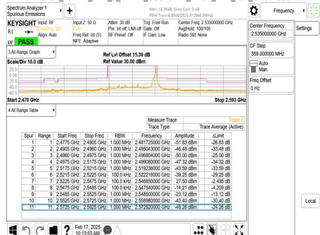
Band7_25MHz_DFT_s_OFDM_SCS15kHz_BPSK_RB1_132_CH507000
