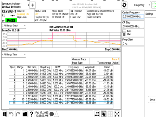
Band7_20MHz_DFT_s_OFDM_SCS15kHz_BPSK_RB1_0_CH502000
