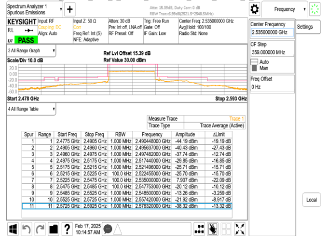
Band7_25MHz_DFT_s_OFDM_SCS15kHz_BPSK_RB1_0_CH507000
