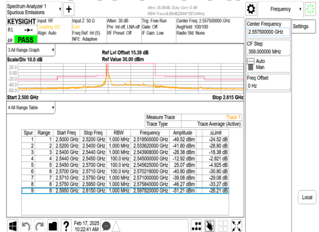
Band7_25MHz_CP_OFDM_SCS15kHz_QPSK_RB1_132_CH511500
