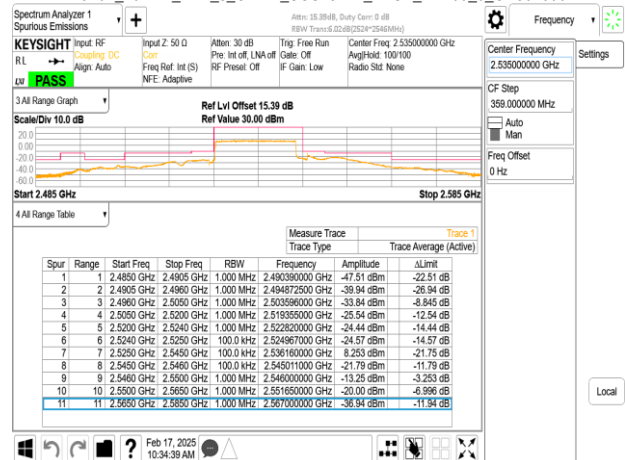
Band7_20MHz_DFT_s_OFDM_SCS15kHz_BPSK_RB1_0_CH507000
