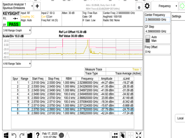
Band7_20MHz_DFT_s_OFDM_SCS30kHz_BPSK_RB50_0_CH512000
