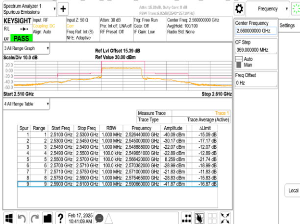
Band7_20MHz_DFT_s_OFDM_SCS15kHz_BPSK_RB1_0_CH512000
