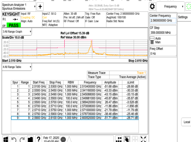
Band7_20MHz_DFT_s_OFDM_SCS15kHz_BPSK_RB1_105_CH512000
