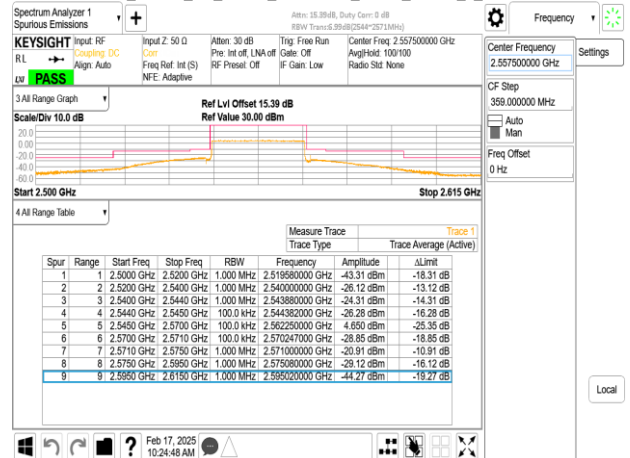
Band7_25MHz_CP_OFDM_SCS15kHz_QPSK_RB1_0_CH511500
