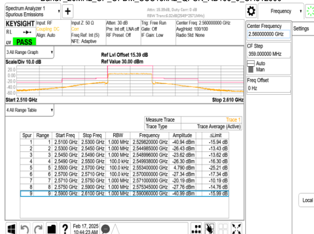
Band7_20MHz_CP_OFDM_SCS15kHz_QPSK_RB1_0_CH512000
