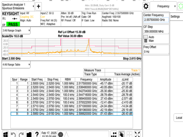
Band7_25MHz_DFT_s_OFDM_SCS15kHz_BPSK_RB1_132_CH511500
