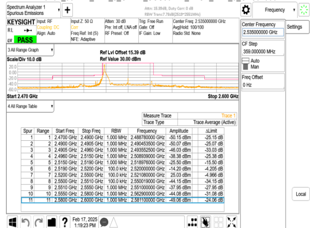
Band7_30MHz_DFT_s_OFDM_SCS30kHz_BPSK_RB1_77_CH507000
