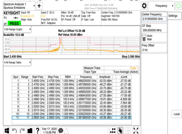
Band7_30MHz_CP_OFDM_SCS30kHz_QPSK_RB1_77_CH503000
