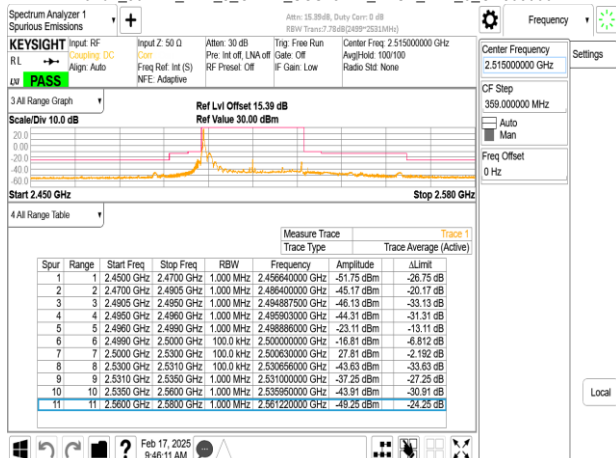
Band7_30MHz_DFT_s_OFDM_SCS15kHz_BPSK_RB1_159_CH503000
