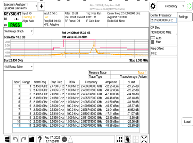
Band7_30MHz_CP_OFDM_SCS30kHz_QPSK_RB78_0_CH503000
