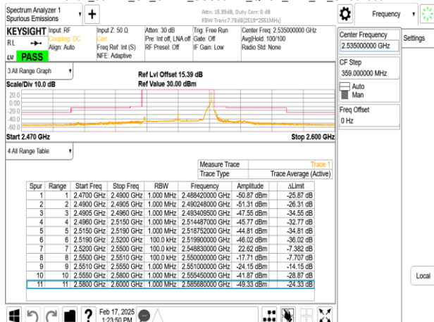
Band7_30MHz_CP_OFDM_SCS30kHz_QPSK_RB78_0_CH507000
