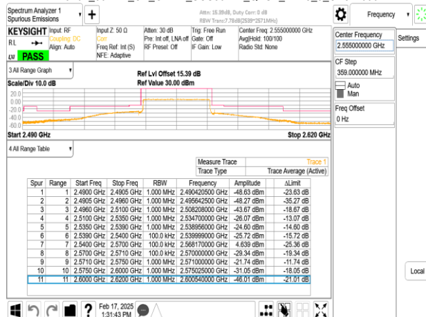
Band7_30MHz_CP_OFDM_SCS30kHz_QPSK_RB78_0_CH511000
