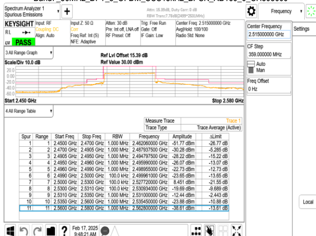
Band7_30MHz_DFT_s_OFDM_SCS15kHz_BPSK_RB1_0_CH503000
