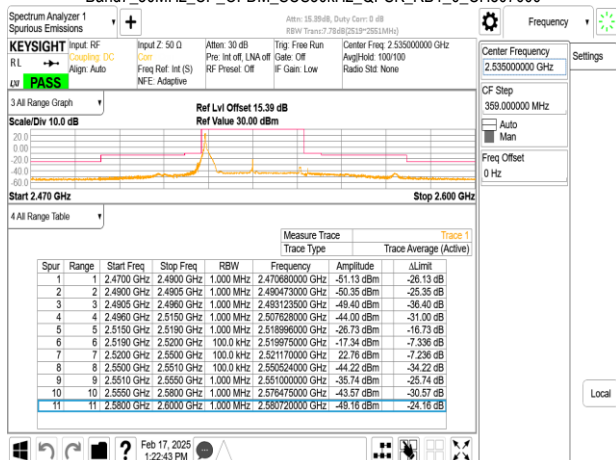
Band7_30MHz_CP_OFDM_SCS30kHz_QPSK_RB1_77_CH507000
