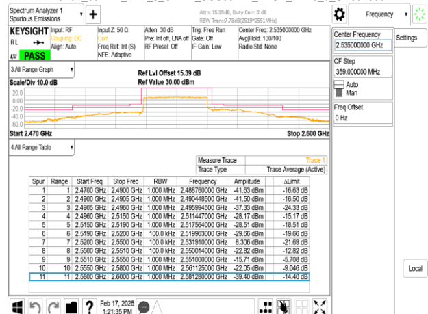
Band7_30MHz_DFT_s_OFDM_SCS30kHz_BPSK_RB75_0_CH507000
