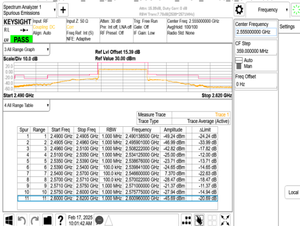
Band7_30MHz_DFT_s_OFDM_SCS15kHz_BPSK_RB1_0_CH511000
