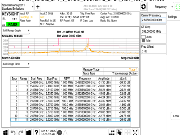
Band7_30MHz_DFT_s_OFDM_SCS15kHz_BPSK_RB1_159_CH511000
