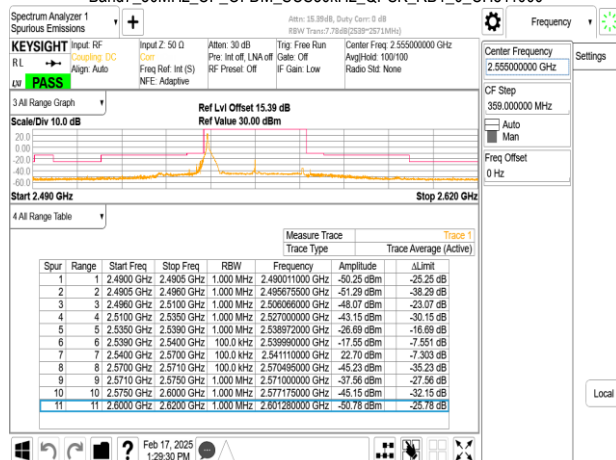
Band7_30MHz_CP_OFDM_SCS30kHz_QPSK_RB1_77_CH511000
