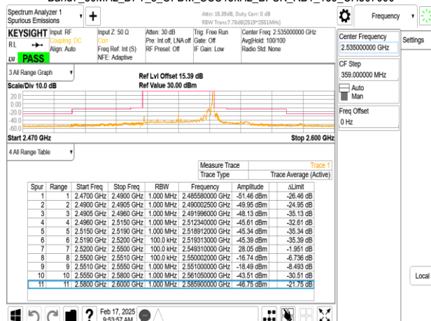
Band7_30MHz_DFT_s_OFDM_SCS15kHz_BPSK_RB1_159_CH507000
