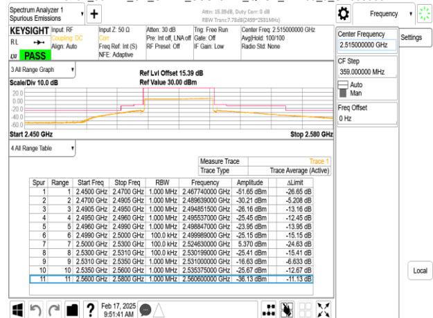
Band7_30MHz_CP_OFDM_SCS15kHz_QPSK_RB1_0_CH503000
